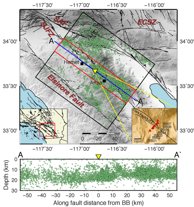
Figure 1. Top panel: the study region (110 km by 100 km black box) centred on the Clark fault in the San Jacinto fault zone (SJFZ). The San Andreas (SAF), Elsinore faults and Eastern California shear zone (ECSZ) are marked. Waveforms from events (light green circles) within the black box are inspected for FZTW. Events within the red rectangle (110 km by 20 km) are used for delay time and FZHW studies. The yellow triangle shows the location of the BB array. The black squares mark the towns of Anza and Hemet. Bottom panel: A depth section of events projected along the profile A–A' on top.
