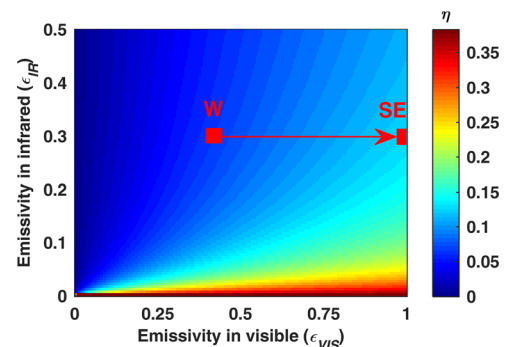
FIG. 2. Influence of a selective emitter's emissivity in the visible and infrared regions on the luminous efficiency of the system when combined with an optical filter of R_{IR}=0.9 and T_{VIS}=1 , at a temperature of 2800 K and F=0.95 . A higher emissivity in the visible and lower emissivity in the infrared lead to higher luminous efficiency. Increasing the emissivity in the visible region of a tungsten filament from \epsilon_{VIS}=0.42 (tungsten emitter, W) to \epsilon_{VIS}=1 (selective emitter, SE) while keeping the infrared emissivity constant increases the luminous efficiency from 6.5 to 12.5%.
