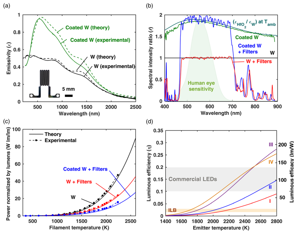
FIG. 4. (a) Theoretical and experimental room temperature emissivity of tungsten and \text{HfO}_2 coated tungsten. The \text{HfO}_2 coated tungsten filament is shown in the inset. (b) Experimental demonstration of the spectral enhancement in the range of 400–887 nm when using a selective emitter ( \text{HfO}_2 coated W ) and optical filters as compared to a bare tungsten emitter ( W ). Filament temperatures at which spectra were taken ranged between 1800 and 2100 K for higher emission at short wavelengths. The maximum and average experimental error on the spectral intensity ratio in the range of 450–850 nm is 0.24 and 0.04, respectively, based on the combined instrumental error and 95% confidence interval on precision error. (c) Filament power consumption normalized by emitted lumens as a function of filament temperature. The view factor between the filament and the filter was approximately 0.93. The experimental error on power was smaller than the symbols (maximum: \pm 0.1 W). (d) Luminous efficiency (%) and efficacy (lm/W) using different selective emitters and filters currently available in the literature [see Fig. S10 (supplementary material) for optical properties] for F=0.99 with corresponding CRI at 2400 K: (I) Tungsten filament + current filter with CRI=91; (II) \text{HfO}_2 coated tungsten filament + current filter with CRI=89; (III) Nanoimprinted superlattice metallic photonic crystal 38 + 600-layer interference filter 39 with CRI=90; (IV) \text{HfO}_2 coated tantalum 34 + 2D metallic photonic crystal filter 23 with CRI=94. Typical ILB and commercial LED luminous efficacies 4 are shown in shaded areas for comparison and are independent of the x-axis (i.e., the efficacies are taken at the nominal operating conditions of the corresponding light sources which are not related to the “Emitter temperature (K)” plotted on the x-axis).
