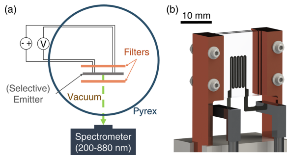
FIG. 3. (a) Schematic (top view) and (b) computer-aided design (CAD) rendering of the experimental setup. A planar radiator-like tungsten filament, fastened to electrical feedthroughs, is sandwiched between planar optical filters (transparent) which are held by copper supports for efficient heat dissipation.
