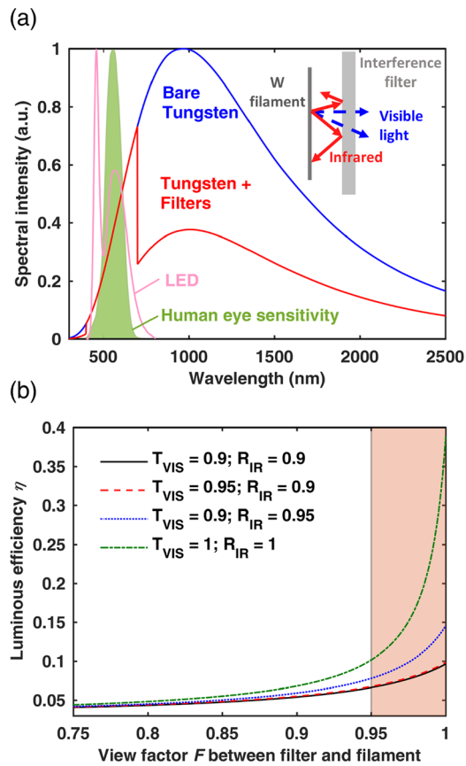
FIG. 1. (a) Spectral intensity for a bare planar tungsten emitter and for a tungsten emitter surrounded with planar selective filters (view factor of F=0.95 ; for the filters, R=1-T is assumed, with typical high performance infrared reflectivity R_{IR}=0.9 and visible transmissivity T_{VIS}=0.95 ). Spectral tailoring using selective filters allows a decrease in the infrared emission and an increase in the luminous efficiency of the light source. The photopic human eye sensitivity curve and the spectrum of a typical white LED 53 are shown for reference. See supplementary material for details of modeling and temperature dependent spectral emissivity of tungsten (Fig. S3). (b) Influence of the filament-filter view factor on the luminous efficiency of a system with a tungsten filament at 2800 K and surrounding filters with different optical properties. Higher view factor, infrared reflectivity, and visible transmissivity lead to higher luminous efficiencies ( \eta ), with a maximum \eta=10.1\% at R_{IR}=1 and T_{VIS}=1 for F \leq 0.95 .
