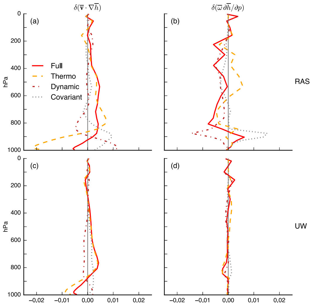
FIG. 8. Profiles of Sahel region-mean values of the 2-K SST warming full response (red curves), and its decomposition into thermodynamic (dashed yellow curves), dynamic (dash-dotted brown curves), and covarying (dotted gray curves) components, for (left) horizontal advection and (right) vertical advection, in (top) RAS and (bottom) UW, in \text{J kg}^{-1} \text{s}^{-1} . Sign conventions are the same as for the transport terms in Fig. 5, namely, with positive values signifying export of MSE.
