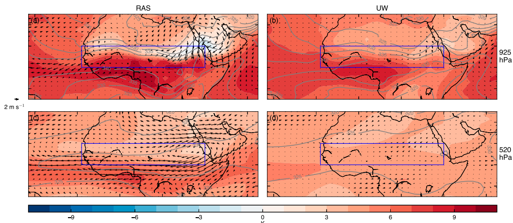
FIG. 10. As in Fig. 4, but for the response in the 2-K SST warming simulation. Responses to 2-K SST warming of MSE, divided by c_p such that units are K (shaded contours), and horizontal wind, in m s^{-1} (arrows), at the model levels corresponding roughly to (top) 925 and (bottom) 520 hPa, in (left) RAS and (right) UW. Note the difference in wind scale compared to Fig. 4.
