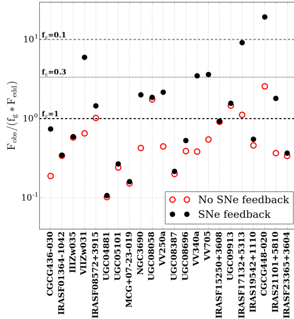
Figure 11. : Observed infrared flux, F_{\text{obs}} (or \Sigma_{\text{IR}}^{33\text{GHz}} ), to predicted Eddington flux times gas fraction, f_g * F_{\text{edd}} , ratio ( F_{\text{obs}}/(f_g * F_{\text{edd}}) ) for each system in the sample. Solid black circles and open red circles show F_{\text{obs}}/(f_g * F_{\text{edd}}) including and not including SNe feedback, respectively. The different horizontal lines indicate how the Eddington limit varies for f_g = 0.1, 0.3, and 1.0 . Assuming a central gas fraction of 1 and considering SNe feedback, we find almost half of our sample is super-Eddington.
