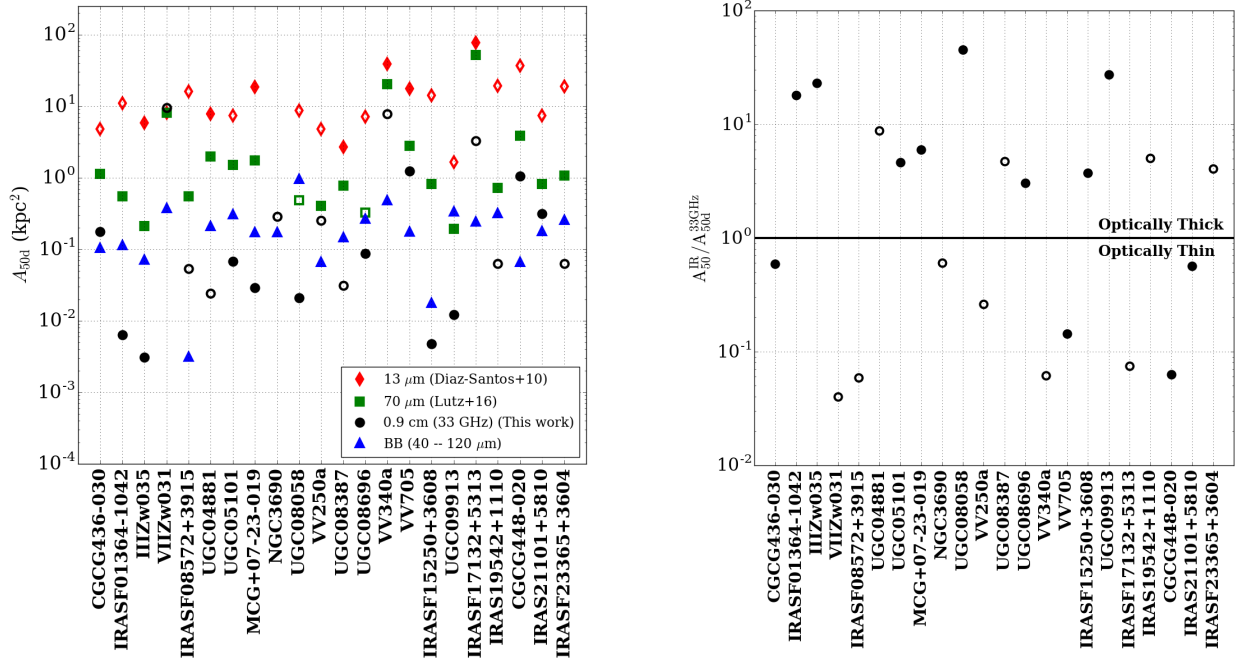
Figure 7. : (Left) Sizes measured at 13 \mu\text{m} (red diamonds), 70 \mu\text{m} (green squares), and 33 GHz (black circles), and those expected for a black body (blue triangles) with L_{\text{IR}} and T_{\text{dust}} (see Section 4.2 for more details). Open symbols indicate upper limits. (Right) Ratio of the area expected for a black body and the area measured at 33 GHz. Open symbols indicate lower limits. The solid horizontal line indicate equality among the areas. Sources above (below) this solid line are optically thick (thin) between 8 and 1000 \mu\text{m} . At least half of the sources in our sample are optically thick at far infrared wavelengths.
