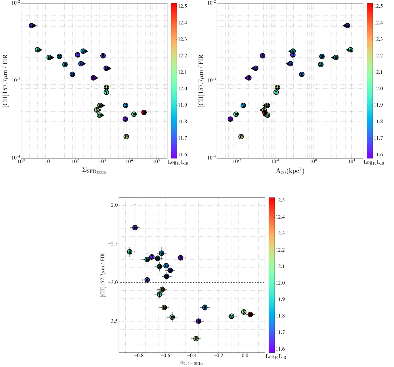
Figure 9. : (Top left) [CII] 158 \mu\text{m} deficit as given by [CII] 158 \mu\text{m} /FIR, where FIR is the far infrared flux density (Díaz-Santos et al. 2013), versus \Sigma_{\text{SFR}_{33\text{GHz}}} , the surface density of star formation inferred from our 33 GHz maps. The systems with the highest star formation per unit area show the highest CII deficit (smallest ratio of [CII] flux/FIR). (Top right) [CII]158 \mu\text{m} /FIR as a function of half-light area at 33 GHz. We observe a higher [CII] deficit for more compact objects. (Bottom) [CII]158 \mu\text{m} /FIR as a function of \alpha_{1.5-6\text{GHz}} . This is consistent with the finding that the [CII] deficit is inversely proportional to mid-IR opacity measurements, i.e., low [CII]158 \mu\text{m} /FIR sources are deeply buried. In all panels, individual systems are labeled by the ID assigned in Table 1 and color coded by their infrared luminosity.
