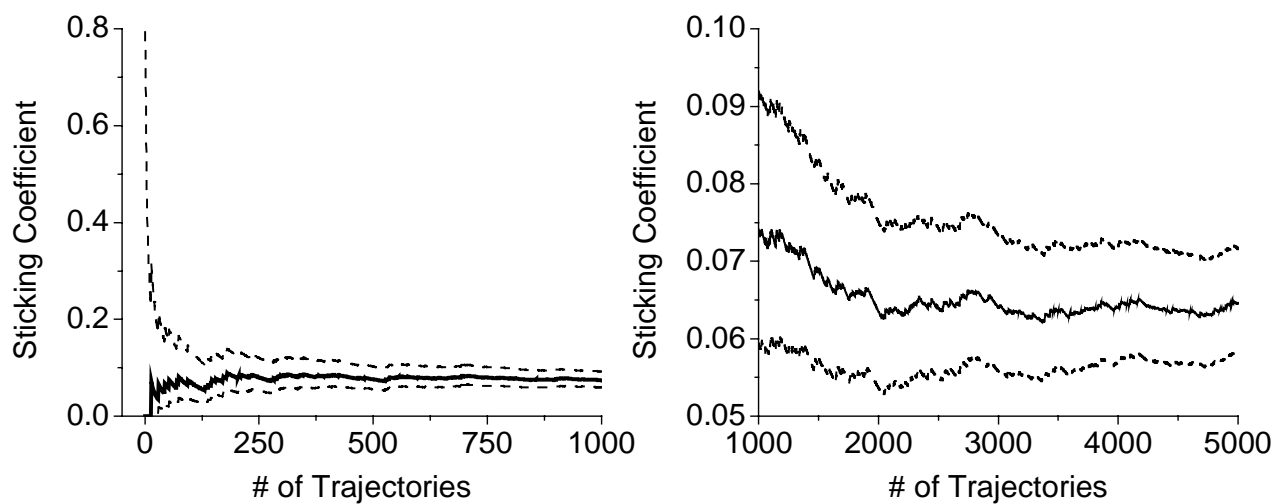
Figure 1S. Pt(533), E=4.0 kcal/mol, normal collision, sticking probability versus number of trajectories up to 1000 (left) and for more trajectories (right). Solid line is best estimate for sticking probability, dotted line is 95% confidence interval estimated using the score confidence interval (see Agresti, A.; Coull, B. A. Am. Stat. 1998 , 52, 119.)
