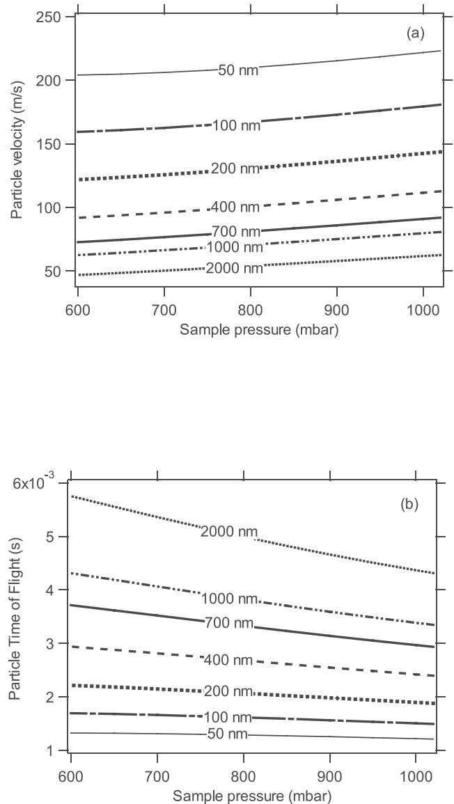
Figure 4. (a) Particle velocity and (b) time of flight variation with ambient pressure for different particle vacuum aerodynamic diameters.
