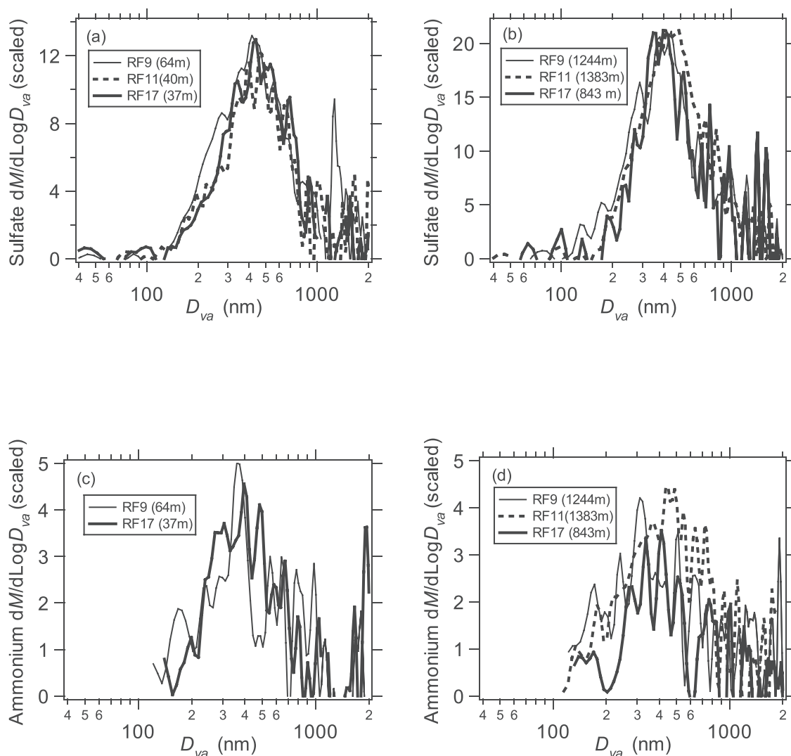
Figure 14. Average sulfate and ammonium mass distributions for (a and c) marine boundary layer and (b and d) pollution layers on Twin Otter RF9, RF11, and RF17 (scaled to the maximum, i.e. scaled to RF9 distribution for marine layer sulfate and ammonium, RF11 distribution for pollution layer sulfate, and RF9 distribution for pollution layer ammonium).
