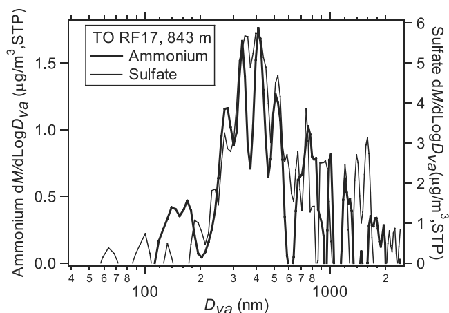
Figure 10. Average ammonium and sulfate mass distributions during Twin Otter RF17 (37 m (00:47–1:35 UTC) and 843 m (3:33–4:20 UTC)).
