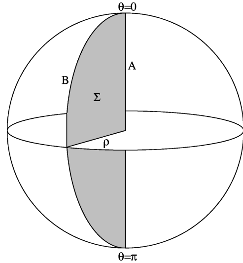
FIG. 2. The Euclidean CCBH instanton. The azimuthal angle is the time \tau/\ell , the polar angle is \theta , and the radius is the proper radius \rho = \int dr/f(r) with \rho(r_H)=0 . Each point represents a circle in the suppressed coordinate \phi . The surface \Sigma is a surface of constant time; its boundary consists of the quasiloc surface B and the axis A of the sphere.
