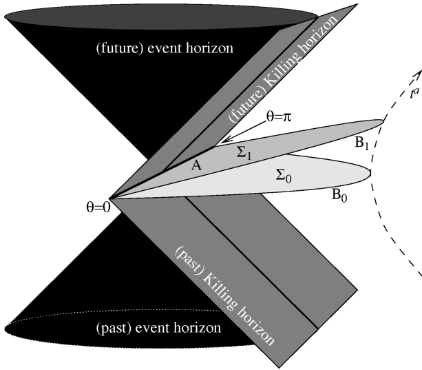
FIG. 1. The Lorentzian CCBH spacetime. The two cones represent the future and past event horizons of the black hole, while the spacelike surfaces \Sigma_0 and \Sigma_1 are surfaces of constant coordinate time. The singularity within the event horizon is not shown. Each point represents a circle in the suppressed coordinate \phi . The outer boundaries of \Sigma_0 and \Sigma_1 are the quasilocal surfaces of constant time and radius. The foliation is degenerate along the axis A , which is the bifurcation surface of the Killing horizon of the vector field t^a . The Killing horizon touches the event horizon along the thick dark lines in the middle of the Killing horizon.
