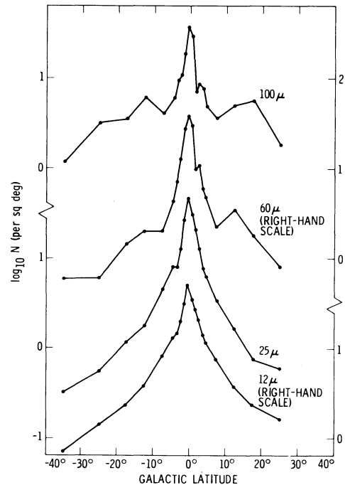
FIG. 1.—The total number of sources per square degree in bins of galactic latitudes for the minisurvey. Each datum point is the average for two strips of the sky, one crossing the galactic plane at a longitude of approximately 338° and the other at approximately 144°. From the bottom, the curves are for the bands centered at 12 \mu\text{m} (lower right-hand scale), 25 \mu\text{m} (lower left-hand scale), 60 \mu\text{m} (upper right-hand scale), and 100 \mu\text{m} (upper left-hand scale).
