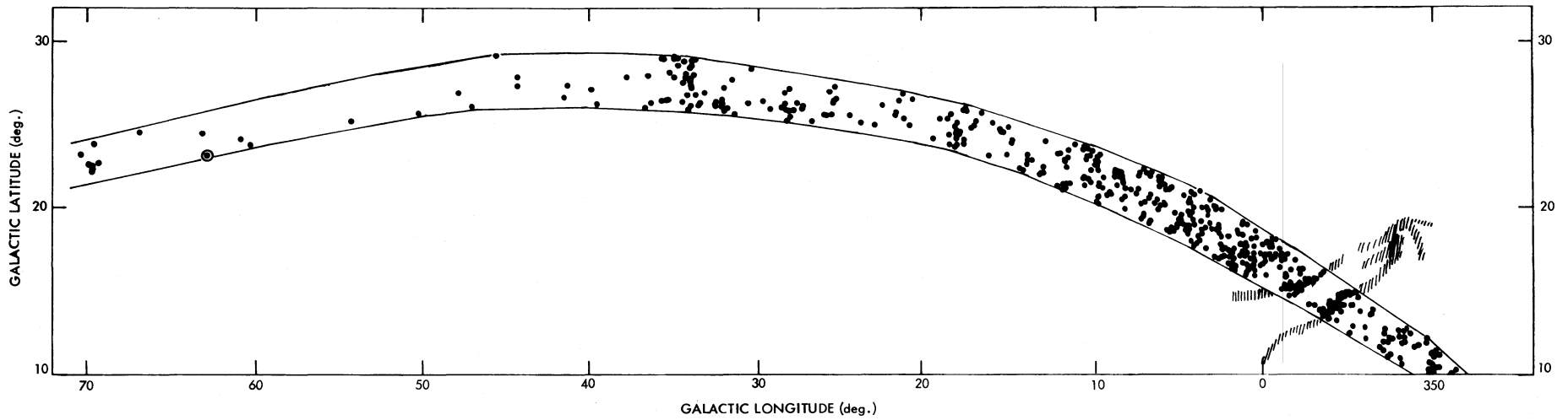
FIG. 4.—The distribution on the sky in galactic coordinates, for a portion of the minisurvey, of the sources seen at 100\ \mu\text{m} only. Note the concentrations of the sources into clouds, particularly for |b| < 20^\circ . A rough sketch of some of the dark clouds associated with the Ophiuchus dark cloud complex, outside the minisurvey strip, is given. Sources associated with galaxies are shown circled.
