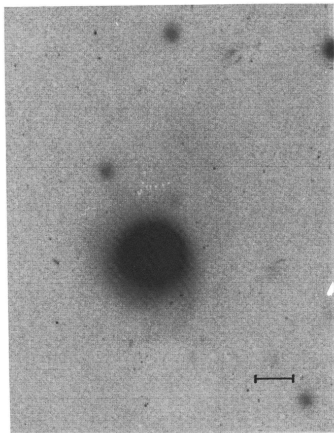
FIG. 2.—CCD images at 6500 \text{ \AA} (Gunn r ) of the ultraluminous infrared galaxy IRAS 05189–2524. For all plots, north is at the top, and east is to the left. The scale is \sim 0''.5 per pixel, and seeing was 1''\text{--}2'' . Two stretches of the same image are presented to show both the nuclear structure and faint large-scale wisps and tails. Bar at the lower right represents 10'' .
