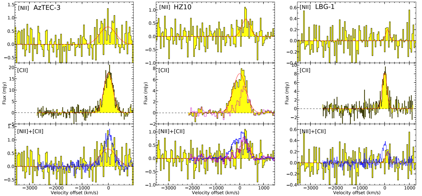
Figure 2. [CII] and [NII] spectra of our sample galaxies at z = 5\text{--}6 , and Gaussian fits to the line emission (red curves). The channel velocity width in all [NII] spectra is \sim 42 \text{ km s}^{-1} ; in the [CII] spectra it is \sim 16 \text{ km s}^{-1} in AzTEC-3 and LBG-1 and \sim 44 \text{ km s}^{-1} in HZ10. [CII] is scaled arbitrarily down in flux density in the bottom panels for comparison. The [NII] line appears to be broader than [CII] in AzTEC-3. HZ10 shows a velocity shift between [CII] and [NII]. The magenta spectra in the central middle and bottom panels show a single-pixel [CII] spectrum extracted at the [NII] peak position (“map peak” method, as defined in Section 3.2; in units of \text{mJy beam}^{-1} , after smoothing to the [NII] resolution), suggesting a common kinematic origin with [NII].
