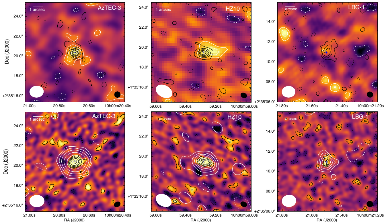
Figure 1. Top: Integrated line maps (over the line FWHM) showing [NII] color-scale with [NII] (white) and [CII] (black) contours. Blue crosses indicate the positions of the 205 \mu\text{m} continuum peak. The [NII] ([CII]) beam is shown in the bottom left (right) corner of each panel. The [NII] ([CII]) contours are multiples of 1\sigma ( 4\sigma ), starting at \pm 2\sigma . The [NII] in the starburst AzTEC-3 is a 5\sigma detection, it is consistent with being centered at the position of the [CII] and continuum emission, and it may be resolved. In the FIR-bright LBG, HZ10, the [NII] emission ( 3.2\sigma per beam at the peak) is slightly resolved ( 5.3\sigma integrated significance) and appears to be offset with respect to the center of the [CII]-emission, indicating significant variation of [CII]/[NII] across the galaxy. The significance of the tentative [NII] detection in LBG-1 is only 2\sigma , which constrains the [CII]/[NII] ratio to be very high ( 68_{-28}^{+200} ). Bottom: Continuum maps showing 158 \mu\text{m} color-scale with 205 \mu\text{m} (white) and 158 \mu\text{m} (black) contours. Contours start at \pm 2\sigma and are at powers of 2\sigma (i.e. \pm 2\sigma, 4\sigma, 8\sigma, \dots ) for AzTEC-3; in steps of 2\sigma for HZ10 and in steps of 1\sigma for LBG-1. The 205 \mu\text{m} (158 \mu\text{m} ) beam is shown in the bottom left (right) corner.
