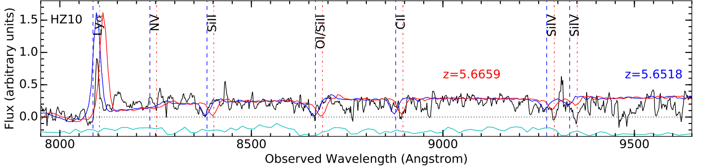
Figure 4. Optical Keck/DEIMOS spectrum of HZ10 shown in black with UV emission/absorption lines identified for two different redshifts ( z = 5.6518 and 5.6659 ). Si II, O I/Si II and Ly \alpha are slightly blue-shifted ( 110 \pm 180 \text{ km s}^{-1} ) relative to the systemic redshift inferred from the FIR [CII] line, likely due to outflowing stellar winds. The UV C II absorption and the high-ionization Si IV lines are redshifted with respect to the systemic velocity ( 522 \pm 200 \text{ km s}^{-1} ) and are compatible with the FIR [NII] emission redshift, which may indicate higher ionization conditions in a part of the galaxy. The blue (red) spectrum shows the stacked z \sim 3 LBG template from Shapley et al. (2003) redshifted to the best fitting match to the two observed sets of lines in HZ10 and scaled to its continuum flux level. The cyan line shows the telluric transmission spectrum (arbitrarily scaled), estimated by the inverse sample variance.
