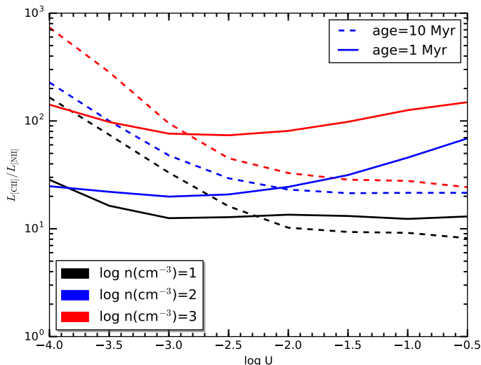
Figure 3. Cloudy model results for the ratio of the [CII] and [NII] line luminosities for a grid of HII region+PDR models. The age of the starburst (1 and 10 Myr, solid and dashed lines) determines the mass of the most massive Main-Sequence star still present and affecting the hardness of the radiation field. The main difference between the different age tracks is that the 1 Myr starburst produces a significant N ^{++} region, while the 10 Myr starburst does not. The density range (from 10 \text{ cm}^{-3} to 1000 \text{ cm}^{-3} ) covers diffuse ionized gas to ultra-compact HII regions. The substantial uncertainty on the intensity of the radiation field at high redshift, in very different environments, is captured by the broad range of ionization parameter (U) considered, along the abscissa. Of particular note are the strong density effect (high density implies higher line ratio) and the slight rise of the ratio for hard radiation and high intensities due to further ionization of N ^{+} to N ^{++} .
