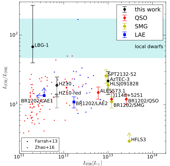
Figure 5. [CII]/[NII] line luminosity ratios observed in high redshift galaxies to date as a function of their FIR luminosity (Carilli & Walter 2013; De Breuck et al. 2014; Bethermin et al. 2016; Rawle et al. 2014; Combes et al. 2012; Carilli et al. 2013; Riechers et al. 2013; R14; C15). For comparison we also show a sample of ULIRGs from Farrah et al. (2013) (using the [NII] 122 \mu\text{m} line) and LIRGs with [NII] (using the [NII] 205 \mu\text{m} line) from Zhao et al. (2016) and [CII] from Diaz-Santos et al. (2013). The range of ratios in dwarfs (Cormier et al. 2015) (using the [NII] 122 \mu\text{m} line) is shown as a cyan band. The [NII] 122 \mu\text{m} line measured in the indicated local samples was converted to a [NII] 205 \mu\text{m} luminosity assuming a ratio of 1/2.5, estimated from Herrera-Camus et al. (2016). The abscissa in the local samples are defined as total FIR luminosity; no attempt was made to convert to a common FIR luminosity scale because it does not affect our interpretation.
