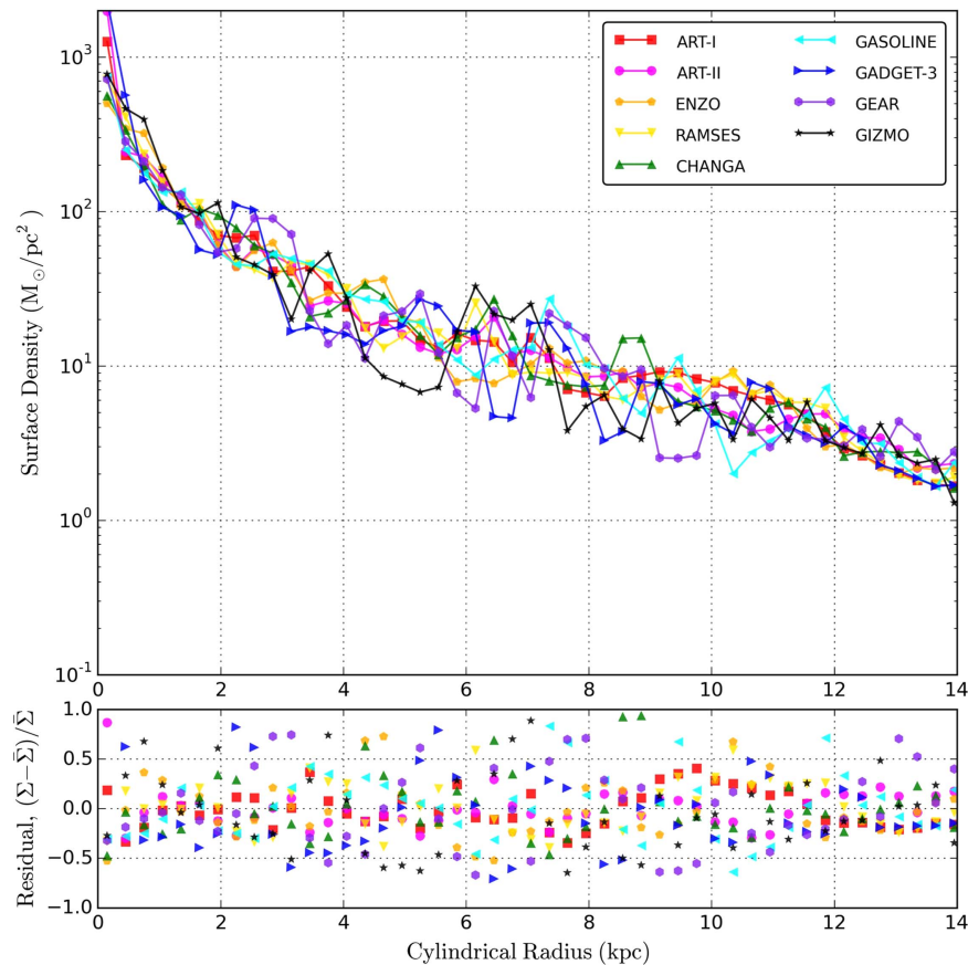
Figure 4. Cylindrically binned gas surface density profiles at 500 Myr for Sim-noSF without star formation or feedback. The cylindrical radius is from the galactic center (location of maximum gas density within 1 kpc from the center of gas mass; in all analyses for particle-based codes hereafter) except the graphical visualizations such as Figures 1–3—raw particle fields are used, not the interpolated or smoothed fields constructed in \gamma\tau . Shown in the bottom panel is the fractional deviation from the mean of these profiles. See Section 6.1 for more information on this figure. The y-axis range of the top panel is kept identical among Figures 4–7 and 22 for easier comparison.
