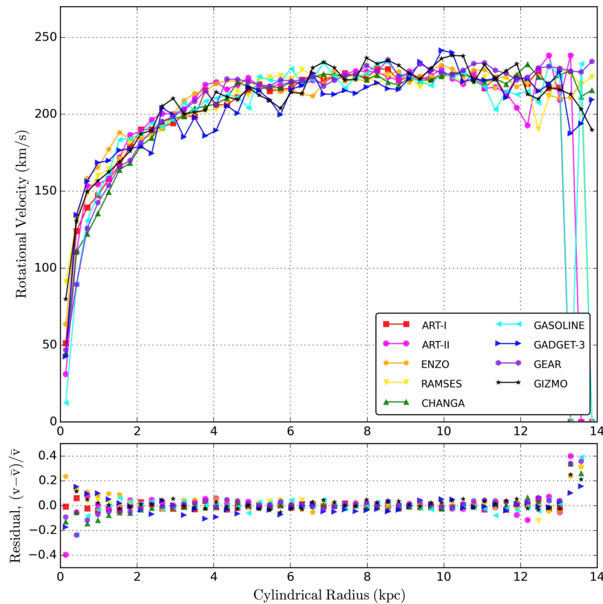
Figure 24. Stellar rotation velocity curves at 500 Myr for Sim-SFF with star formation and feedback. The cylindrical radius and rotational velocity are with respect to the galactic center—location of maximum gas density within 1 kpc from the center of gas mass. Only the newly formed star particles are considered. See Section 6.5 for a detailed explanation on how this figure is made. Compare with Figure 11. The y-axis range of the top panel is kept identical among Figures 10, 11, and 24 for easier comparison.
