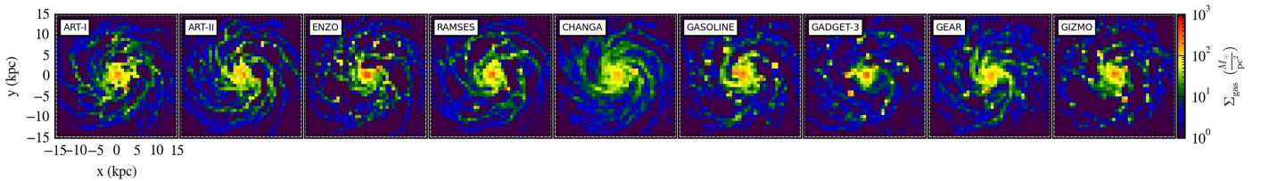
Figure 29. 500 Myr snapshot of face-on gas surface densities for Sim-SFF at 750 pc resolution. For particle-based codes, surface densities are estimated by depositing gas particles via the cloud-in-cell (CIC) scheme on to a two-dimensional uniform grid with 750 pc resolution. This image could be considered as a degraded version of Figure 3 although a different deposit algorithm is used for particle-based codes. See Section 6.6 for a detailed explanation on how this figure is made.
