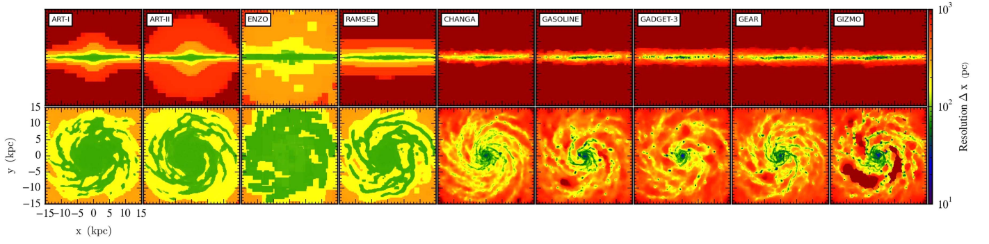
Figure 35. 500 Myr composite of the size of resolution elements along different lines of sight, edge-on (top) and face-on (bottom), for Sim-SFF with star formation and feedback. The color axis spans from 10 to 10^3 pc in a logarithmic scale, with highest resolution shown in dark blue. See Section 6.6 for a detailed explanation on how this figure is made. Compare with Figures 3, 15, and 21.
