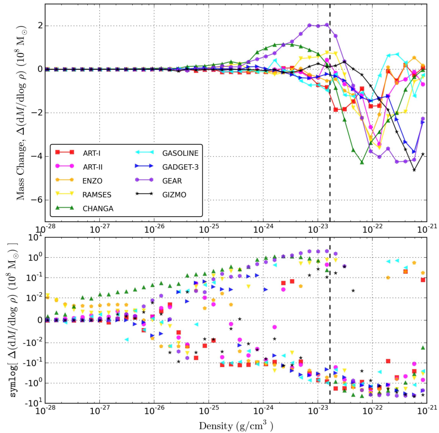
Figure 20. Code-by-code mass change in each density bin from Figures 18 to 19. This plot measures the effect of star formation and feedback by subtracting the density probability distribution function of Sim-noSF from that of Sim-SFF . The y-axis spans from -7 \times 10^8 M_\odot to +3 \times 10^8 M_\odot in a linear scale. Shown in the bottom panel is the sign-preserving logarithm of the mass difference in order to make smaller changes to stand out. 74 The thick dashed line denotes the star formation threshold density, n_{\text{H,thres}} = 10 \text{ cm}^{-3} . See Section 6.3 for more information on this figure.
