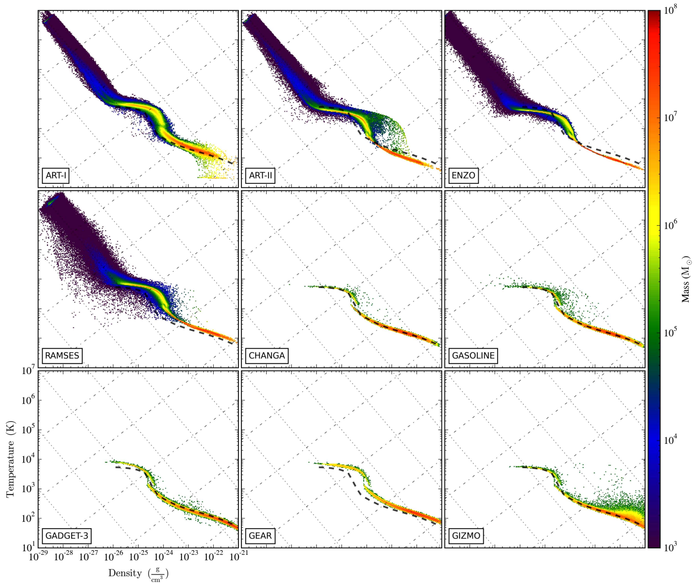
Figure 16. 500 Myr composite of two-dimensional probability distribution function of density and temperature for the gas within 15 kpc from the galactic center in Sim-noSF without star formation or feedback. Colors represent the total gas mass in each two-dimensional bin. A gaseous halo—low-density, high-temperature gas in the upper left corner of each panel—exists only in mesh-based codes, but not in particle-based codes (SPH codes or GIZMO). To guide the eye, we use a thick dashed line in each panel to plot the mean temperature in each density bin for CHANGA. The thin dotted diagonal lines denote the slope of constant pressure process, and the thin dotted-dashed diagonal lines that of constant entropy process. Note that different versions of GRACKLE are interfaced with different codes (GRACKLE v2.1 in CHANGA, GASOLINE, GADGET-3, and GIZMO, vs. GRACKLE v2.0 or below in ART-I, ART-II, ENZO, RAMSES, and GEAR). See Section 6.3 for more information on this figure. The high-resolution versions of this figure and article are available at the Project website, http://www.AGORAsimulations.org/ .
