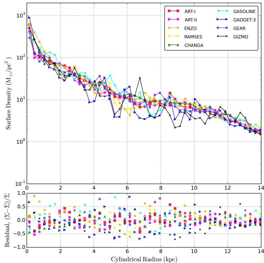
Figure 5. Same as Figure 4 but for Sim-SFF with star formation and feedback. Compare with Figures 22 and 27.
