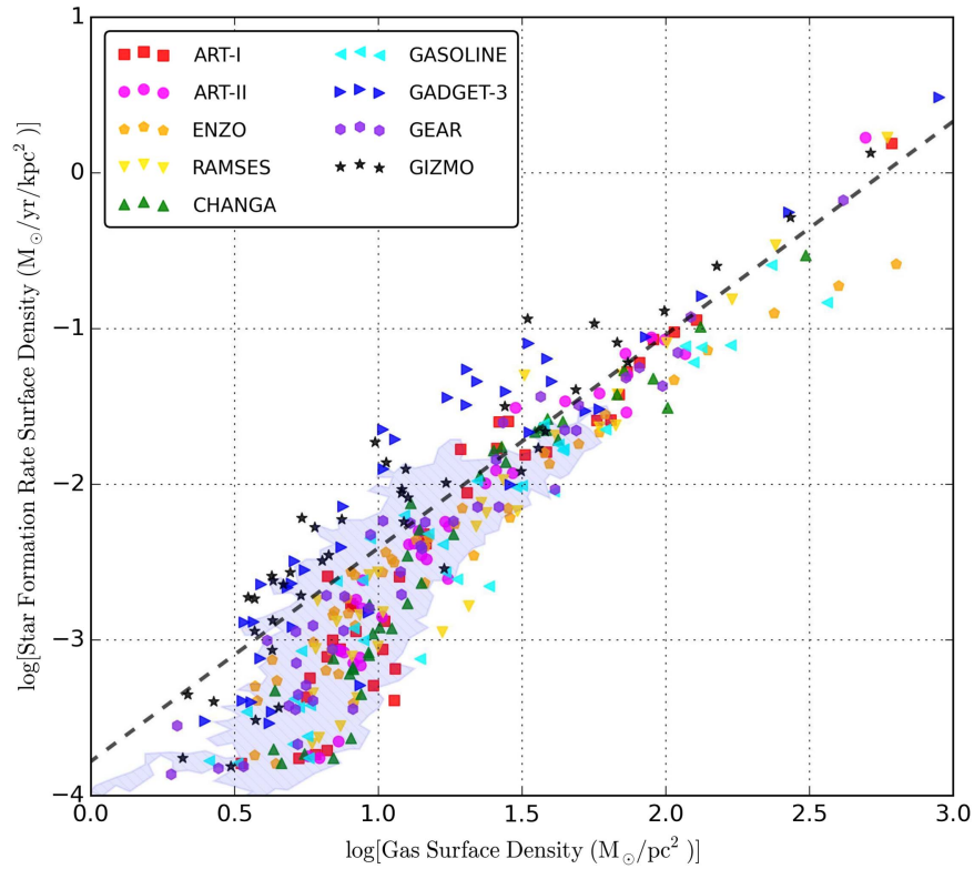
Figure 28. Kennicutt–Schmidt relation for Sim-SFF at 500 Myr using the azimuthally averaged gas surface densities (Figure 5) and SFR surface densities (Figure 27). The thick black dashed line denotes a best observational fit by Kennicutt et al. (2007). The blue hatched contour marks the observed sub-kpc patches in nearby galaxies by Bigiel et al. (2008), where their hydrogen surface density is multiplied by 1.36 to match the total gas surface density in our simulations. See Section 6.6 for a detailed explanation on how this figure is made.
