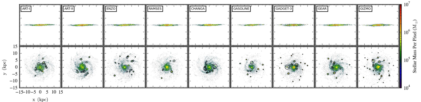
Figure 21. 500 Myr composite of newly formed star particle distributions, edge-on (top) and face-on (bottom), for Sim-SFF with star formation and feedback. Only the newly formed star particles are drawn, not the disk or bulge stars that were present in the IC. Colors represent the total newly formed stellar mass in each two-dimensional bin. We also highlight the clumps of newly formed star particles identified by the friends-of-friends (FOF) algorithm with circles. Clumps with masses below 2.6 \times 10^6 M_\odot and the most massive clump found by FOF (always associated with the stellar bulge at the galactic center) are excluded. See Section 6.4 for a detailed explanation of this figure. Compare with Figures 3, 15, and 35. The high-resolution versions of this figure and article are available at the Project website, http://www.AGORAsimulations.org/ .
