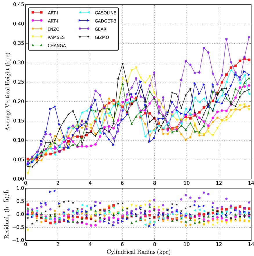
Figure 8. Cylindrically binned, mass-weighted averages of gas vertical heights for Sim-noSF without star formation or feedback. The height is the absolute vertical distance from the x - y disk plane centered on the galactic center, |z_i - z_{\text{center}}| . Shown in the bottom panel is the fractional deviation from the mean of these profiles. See Section 6.1 for an explanation on how this figure is made.
