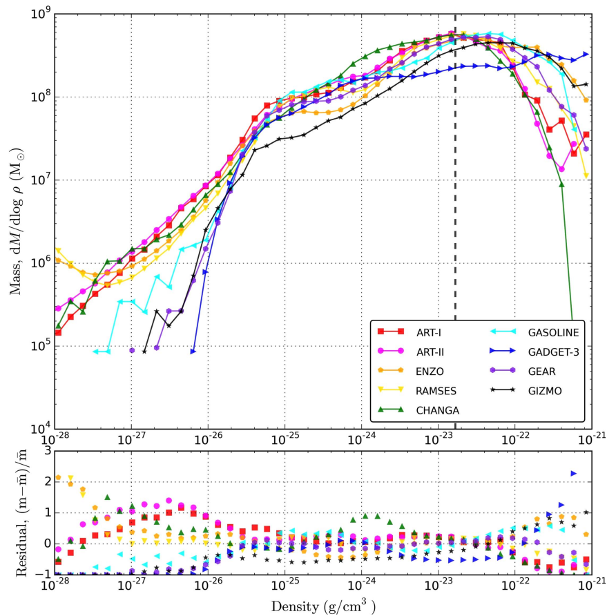
Figure 19. Same as Figure 18 but for Sim-SFF with star formation and feedback. The thick dashed line denotes the star formation threshold density, n_{\text{H,thres}} = 10 \text{ cm}^{-3} .
