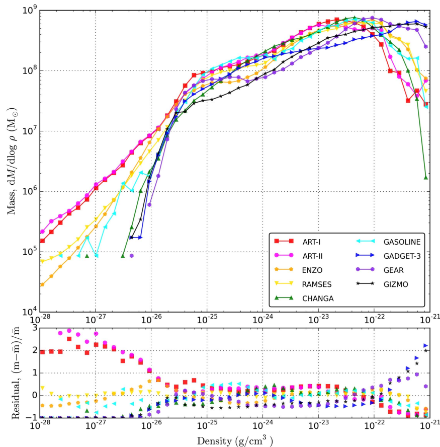
Figure 18. Gas density probability distribution function at 500 Myr for Sim-noSF without star formation or feedback. Note that a gaseous halo—low-density tails toward the left side of this plot—exists only in mesh-based codes, but not in particle-based codes (SPH codes or GIZMO). Shown in the bottom panel is the fractional deviation from the mean of these profiles. See Section 6.3 for more information on this figure.
