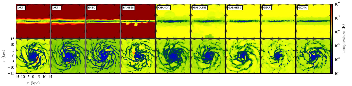
Figure 14. 500 Myr composite of density-square-weighted gas temperature projections, edge-on (top) and face-on (bottom), for Sim-noSF with radiative gas cooling but without star formation or supernova feedback. See Section 5 for descriptions of participating codes in this comparison, and Section 6.3 for a detailed explanation of this figure. Compare with Figure 2. The high-resolution versions of this figure and article are available at the Project website, http://www.AGORAsimulations.org/ .
