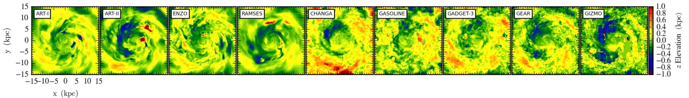
Figure 34. 500 Myr face-on composite of density-weighted averages of gas elevations for Sim-SFF with star formation and feedback. See Section 6.7 for a detailed explanation on how this figure is made. Compare with Figures 3 and 15. The high-resolution versions of this figure and article are available at the Project website, http://www.AGORAsimulations.org/ .
