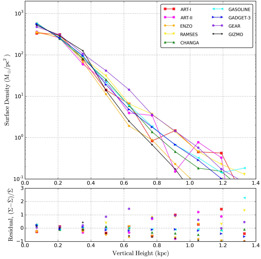
Figure 6. Vertically binned gas surface density profiles at 500 Myr for Sim-noSF without star formation or feedback. The height is the absolute vertical distance from the x - y disk plane centered on the galactic center, |z_i - z_{\text{center}}| . Shown in the bottom panel is the fractional deviation from the mean of these profiles. The y-axis range of the top panel is kept identical among Figures 4–7 and 22 for easier comparison.
