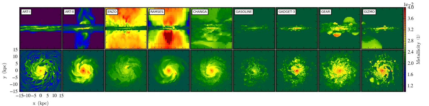
Figure 32. 500 Myr composite of density-square-weighted gas metal fraction projections, edge-on (top) and face-on (bottom), for Sim-SFF with star formation and feedback. Colors represent the ratio of metal density to total gas density (not in units of Z_{\odot} ). The color axis spans from 0.01 to 0.04 in a linear scale. See Section 6.7 for a detailed explanation of this figure. Compare with Figures 3, 15, and 21. The high-resolution versions of this figure and article are available at the Project website, http://www.AGORAsimulations.org/ .
