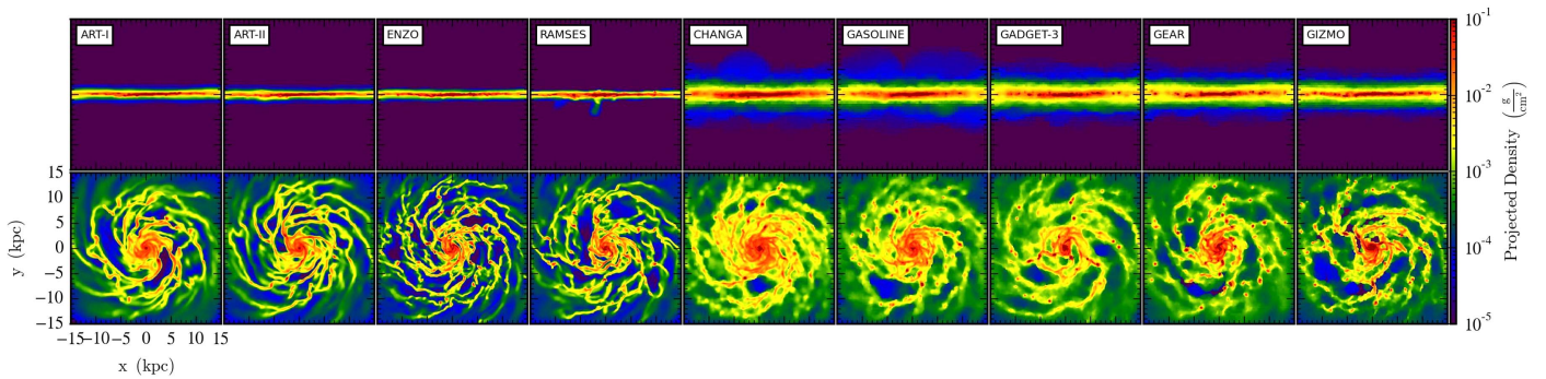
Figure 2. 500 Myr composite of gas surface densities from Sim-noSF with radiative gas cooling but without star formation or supernova feedback. Each frame is centered on the galactic center—location of maximum gas density within 1 kpc from the center of gas mass. For visualizations of the particle-based codes hereafter (Figures 1–3, 14–15, 32, 34, and 35)—but not in any other analyses except these figures—yt uses an in-memory octree on which gas particles are deposited using smoothing kernels. See Section 5 for descriptions of participating codes in this comparison, and Section 6.1 for a detailed explanation of this figure. Compare with Figure 14. Simulations performed by: Daniel Ceverino (ART-I), Robert Feldmann (ART-II), Mike Butler (ENZO), Romain Teyssier (RAMSES), Spencer Wallace (CHANGA), Ben Keller (GASOLINE), Jun-Hwan Choi (GADGET-3), Yves Revaz (GEAR), and Alessandro Lupi (GIZMO). The high-resolution versions of this figure and article are available at the Project website, http://www.AGORAsimulations.org/ .
