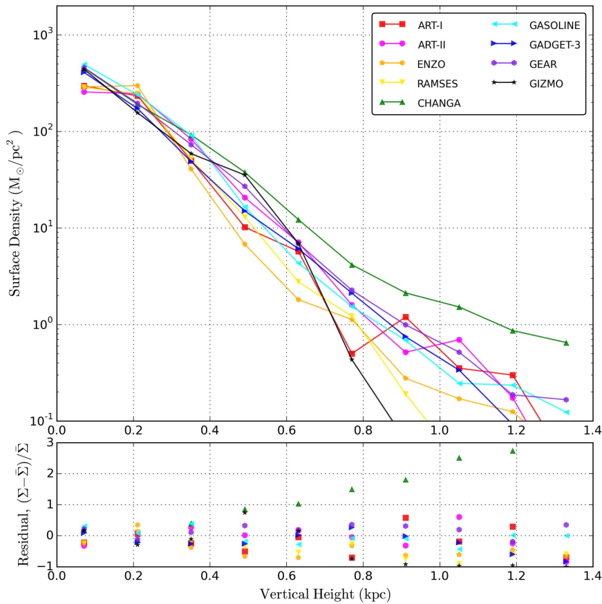
Figure 7. Same as Figure 6 but for Sim-SFF with star formation and feedback.
