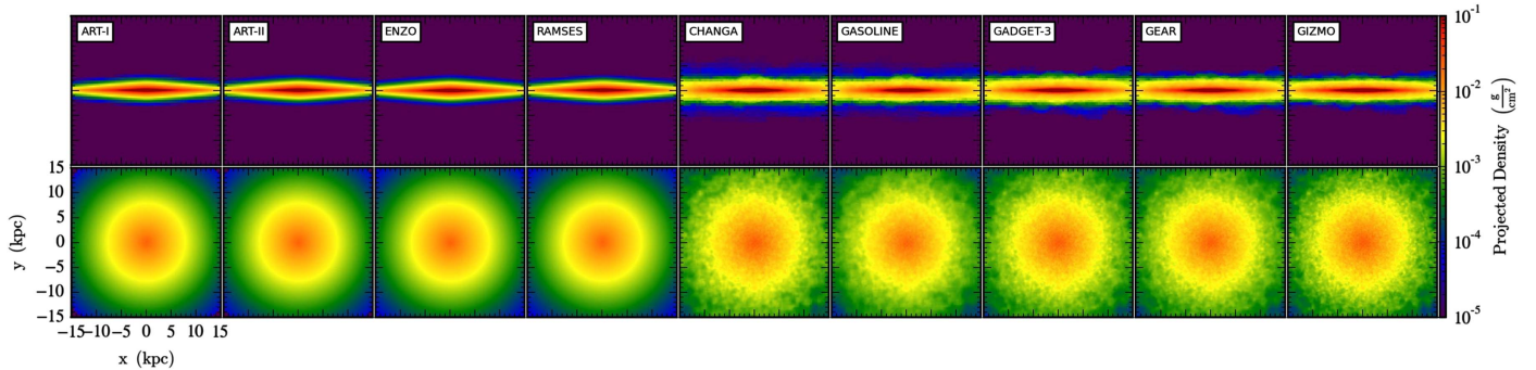
Figure 1. 0 Myr snapshots of the isolated Milky Way-mass galaxy simulations by nine participating codes. Disk gas surface densities in a 30 kpc box, edge-on (top) and face-on (bottom), produced with the common analysis toolkit yt. For visualizations of the particle-based codes hereafter (Figures 1–3, 14–15, 32, 34, and 35)—but not in any other analyses except these figures—yt uses an in-memory octree on which gas particles are deposited using smoothing kernels. Comparing 0 Myr snapshots—dumped immediately after each code reads in the IC—is to check the exact identity of ICs interpreted by each code. See Section 6.1 for more information on this figure, and Section 5 for descriptions of participating codes in this comparison. The high-resolution versions of this figure and article are available at the Project website, http://www.AGORAsimulations.org/ .
