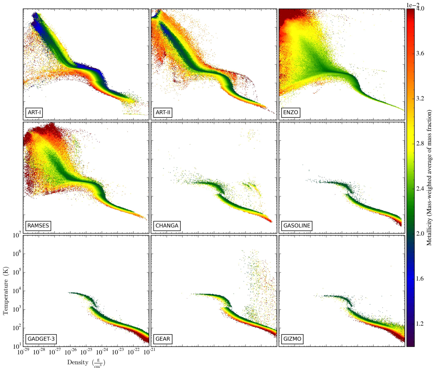
Figure 33. 500 Myr composite of the mass-weighted averages of gas metal fraction on a density–temperature plane for the gas within 15 kpc from the galactic center in Sim-SFF with star formation and feedback. The metal fraction is simply the ratio of metal density to total gas density (not in units of Z_{\odot} ). Note that a gaseous halo—low-density, high-temperature gas in the upper left corner of each panel—exists only in mesh-based codes, but not in particle-based codes (SPH codes or GIZMO). Compare with Figure 17. See Section 6.7 for more information on this figure. The high-resolution versions of this figure and article are available at the Project website, http://www.AGORAsimulations.org/ .
