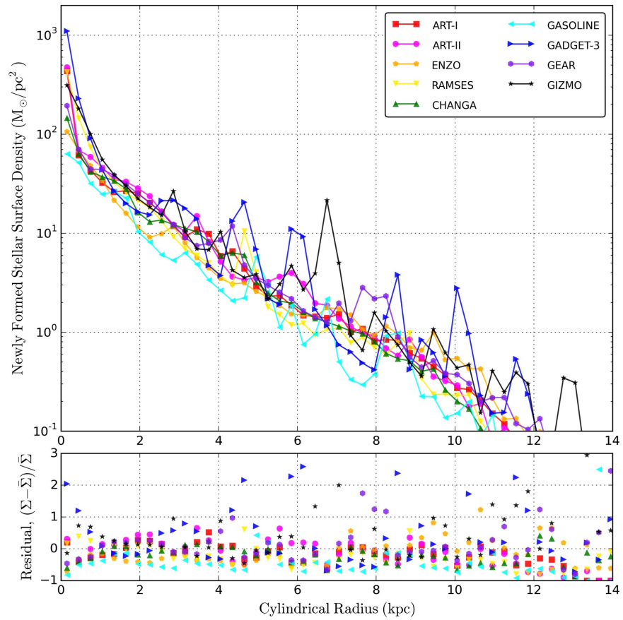
Figure 22. Cylindrically binned newly formed stellar surface density profiles at 500 Myr for Sim-SFF with star formation and feedback. Only the newly formed star particles are considered, not the disk or bulge stars that were present in the IC. Shown in the bottom panel is the fractional deviation from the mean of these profiles. See Section 6.4 for a detailed explanation of this figure. Compare with Figures 5 and 27. The y-axis range of the top panel is kept identical among Figures 4–7 and 22 for easier comparison.
