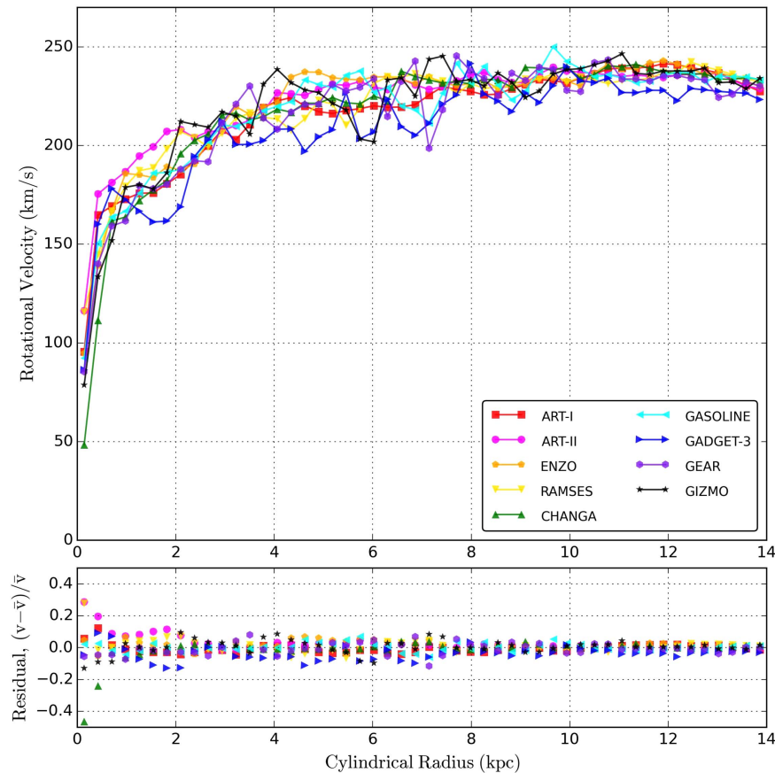
Figure 10. Gas rotation velocity curves at 500 Myr for Sim-noSF without star formation or feedback. The cylindrical radius and rotational velocity are with respect to the galactic center—location of maximum gas density within 1 kpc from the center of gas mass. Shown in the bottom panel is the fractional deviation from the mean of these profiles. See Section 6.2 for a detailed explanation on how this figure is made.
