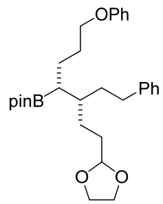
Entry C (CDCl 3 , 400 MHz)
