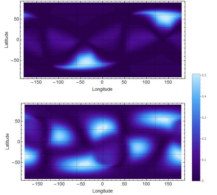
FIG. 3. The effective angular pattern function \mathcal{F}_3(\hat{\Omega}) for network H-L-V (upper panel) and \mathcal{F}_4(\hat{\Omega}) for network H-L-V-K (lower panel) as a function of \hat{\Omega} , the direction of the source. The x axis is the longitude as observed on the earth and y axis the latitude.
