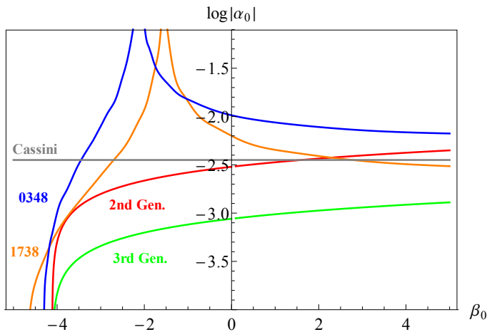
FIG. 4. Discoverable curves of S memory from a collapsing star with M = 10M_{\odot} , R = 100M_{\odot} and r = 10\text{kpc} for 2nd generation detectors (Red) and 3rd generation detectors (Green). The current constraints on the model parameters are from the Cassini Mission (Grey), PSR J1738+0333 (Orange) and PSR J0348+0432 (Blue).
