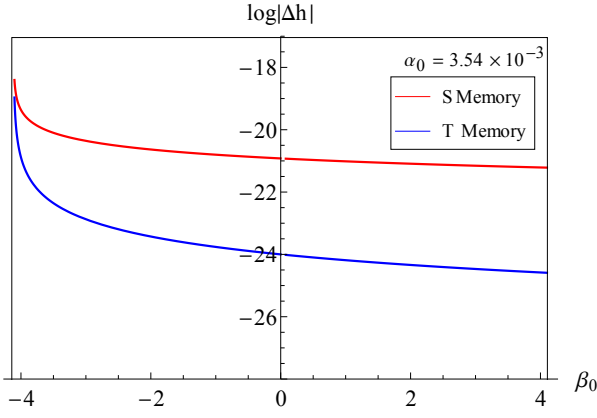
FIG. 2. Scales of T memory and S memory from gravitational collapse of an M = 10M_\odot , R = 100M_\odot , \epsilon = 0.1 and r = 10\text{kpc} Newtonian star.
