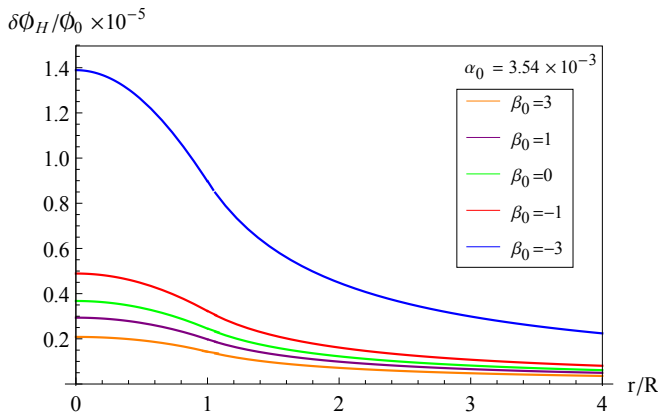
FIG. 1. The stationary interior and exterior scalar field profile of an M = 10M_\odot and R = 100M_\odot Newtonian star for different values of \beta_0 .
