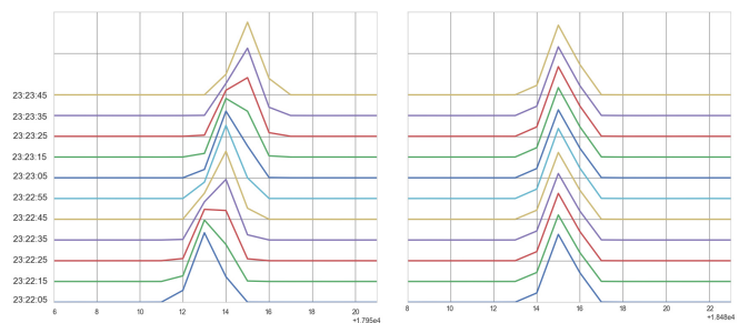
Fig. 8. Zoom into the carrier line without (left panel) and with the Doppler phase correction (right panel). 10 sec integration time, 2^{15} = 32768 points spectral resolution, baseline Hh-Ww, scan 135. 23:22 – 23:24 UTC, December 28, 2013.
