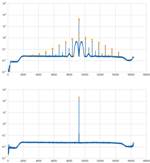
Fig. 9. Averaged amplitude spectrum after applying the Doppler phase correction in arbitrary units, 2^{14} = 16384 points spectral resolution, baseline T6-Sv, scan 209 (top) and 191 (bottom). Only the carrier line was present in the spectrum in the second case, as was the case for \sim 50\% of the time during GR035. The spectral mask is shown in orange dots.
