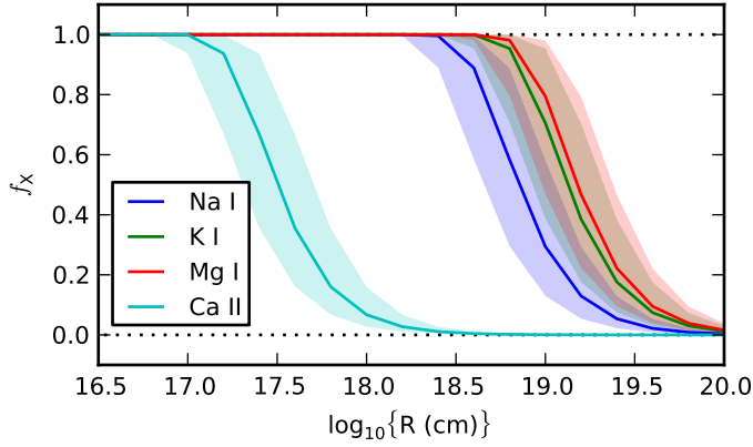
Fig. 11. Total fraction of photoionisation of different ISM species as a function of distance from the SN. The bands indicate a \pm 1 mag change in ionising UV flux.
