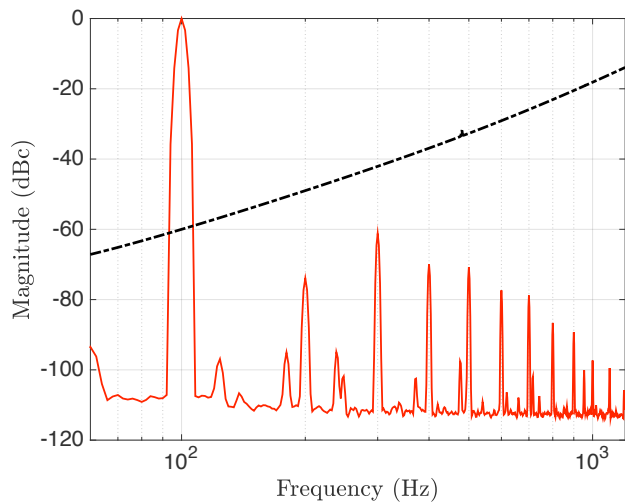
Figure 8. Suppressed modulation harmonics relative to the carrier. The 100 Hz modulation is at 95% of the maximum diffracted power. All harmonics are well below the Advanced LIGO noise requirements (in black).
