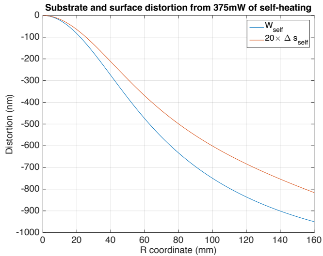
Figure 4: Radial distribution of thermo-refractive wavefront distortion, W_{\text{self}} , from 375mW of self-heating.
