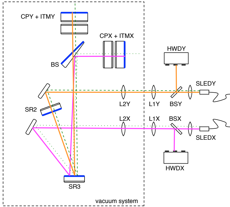
Figure 6: The optical layout of the ITMX and ITMY Hartmann wavefront sensors. Probe beams (X-arm, purple, Y-arm, orange) are produced by fiber-coupled super-luminescent diodes (SLEDX, SLEDY). After being collimated, these beams are passed through several imaging optics inside and outside the vacuum system. The beams are then steered into the interferometer core optics (SR2, SR3) and up to the beam splitter (BS - shown with an exaggerated wedge) where the X-arm beam is reflected from the anti-reflecting (at 1064nm) side of the BS and the Y-arm beam is transmitted. Each beam passes through its respective compensation plate and ITM substrate and is retro-reflected from the ITM HR surface. The beams return all the way out of the vacuum system where they are picked off by 50/50 beam splitters (BSX, BSY) and are incident on their respective detectors (HWD). Leakage of the two green ALS lasers beams (shown by dotted and dashed green lines) are used to align the HWS beams to the test masses [18].
