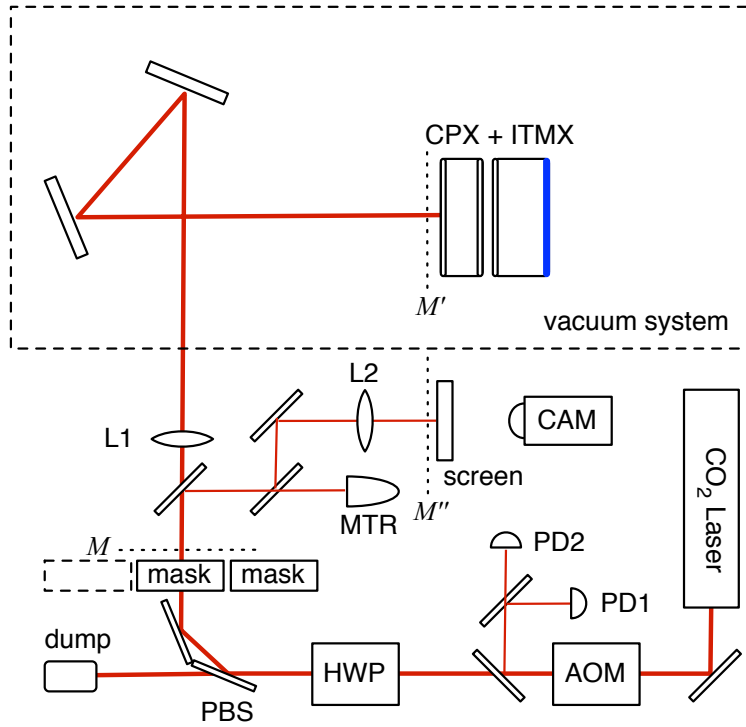
Figure 11: Schematic layout of CO 2 laser projector
