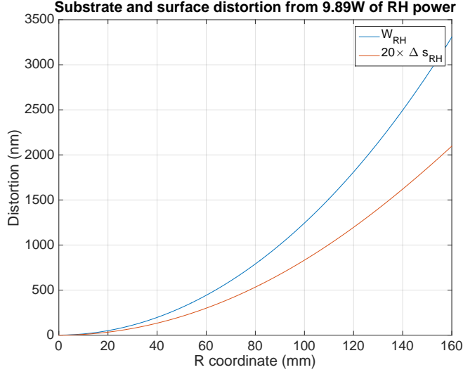
Figure 9: The round-trip wavefront distortion from 9.89W of RH power, W_{RH} .
