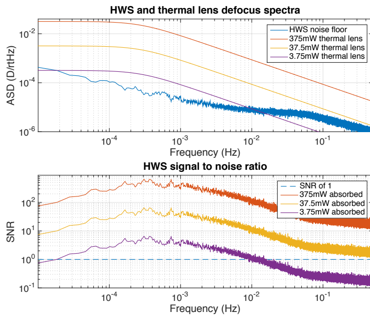
Figure 7: Background defocus noise spectra (in diopters) of the aLIGO HWS. The expected thermal lens magnitudes for different frequencies and absorbed powers are also shown.
