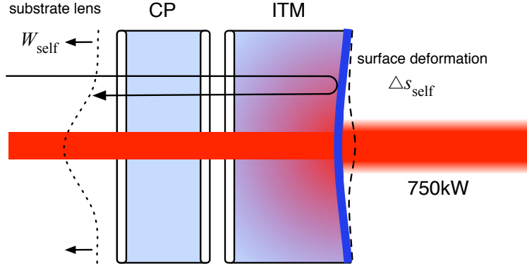
Figure 3: An illustration of the thermo-refractive substrate lens, W_{\text{self}} , and the thermo-elastic surface deformation, \Delta s_{\text{self}} , from self heating.
