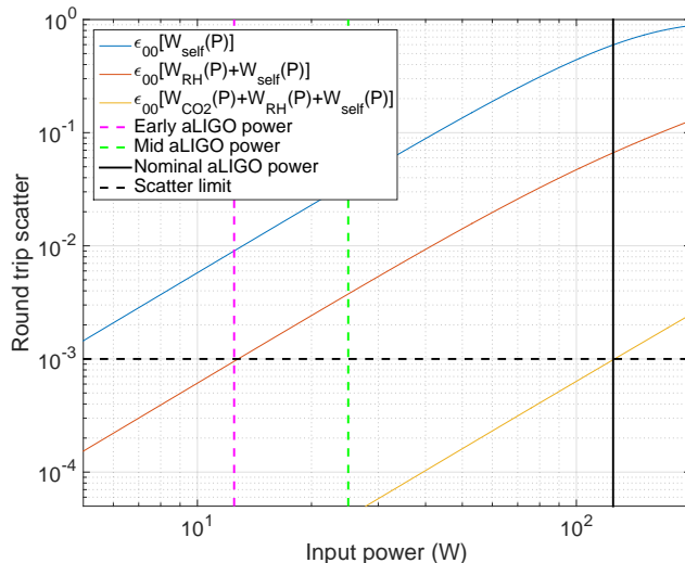
Figure 15: Round-trip scatter vs aLIGO input power. Also shown are the operating power levels for aLIGO. The maximum scatter 0.1%, shown by the black dashed line.
