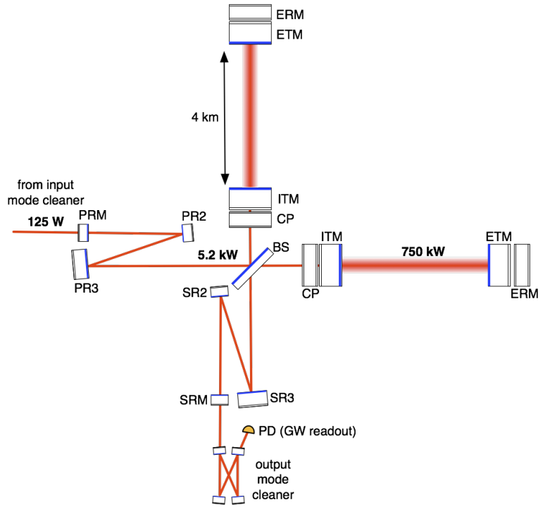
Figure 1: aLIGO layout. The pre-stabilized laser beam is injected into an input mode cleaner (not shown). The output of this is injected into the dual-recycled Fabry-Perot Michelson interferometer through mirror PRM. The Fabry-Perot arms are formed between the high-reflectivity (HR) surfaces of the input test mass (ITM) and end test mass (ETM) of each arm where up to 750kW of circulating power is stored. Any differential change in the arm lengths will result in a change in the output signal from the interferometer through the output mirror SRM where it will be spatially filtered by the output mode cleaner and detected on the GW readout photodiode (PD). See reference [1], from which this figure is adapted, for a full description of the layout.
