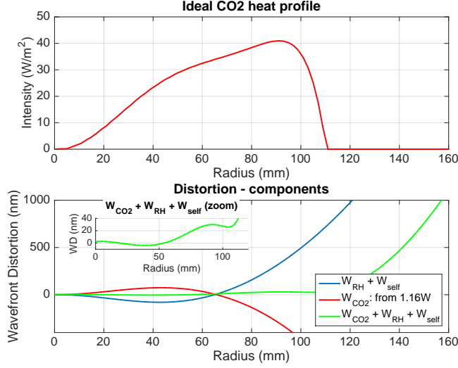
Figure 12: (upper) Optimum CO 2 heating pattern and (lower) the resulting wavefront distortion due to thermo-refractive lensing.
