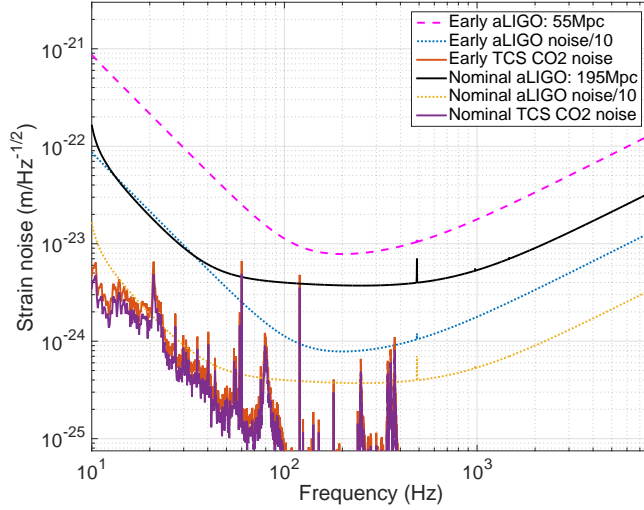
Figure 13: Estimated displacement noise from the CO 2 laser for LIGO during Early and Nominal aLIGO. The dotted blue line is the maximum allowed technical displacement noise for Early aLIGO. The solid red line is the estimated contribution of displacement noise from approximately 750mW of central heating. The dotted yellow line is the maximum allowed technical displacement noise for Nominal aLIGO. The solid purple line is the estimated contribution from approximately 1.16W of annular heating.
