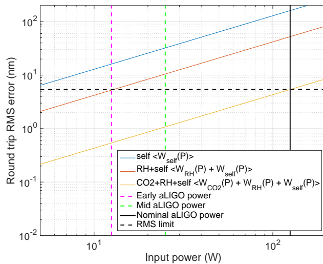
Figure 14: RMS error vs aLIGO input power. Also shown are the operating power levels for aLIGO. The maximum allowed RMS is 5.4nm, shown by the black dashed line.
