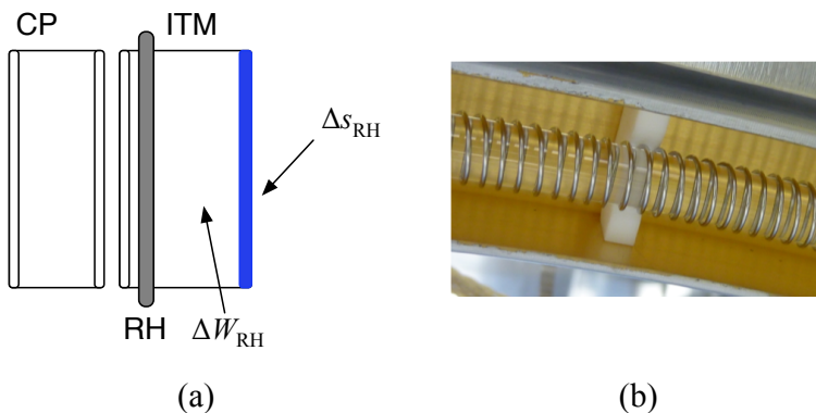
Figure 8: (a) the aLIGO RH torus, (b) the nichrome wire encircled RH torus
