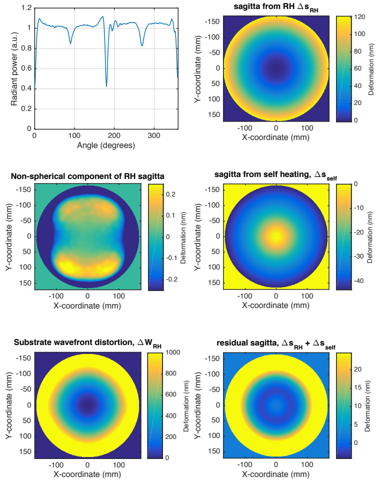
Figure 10: Example of the residual thermal lens error (once spherical power has been removed) from the non-idealized RH
