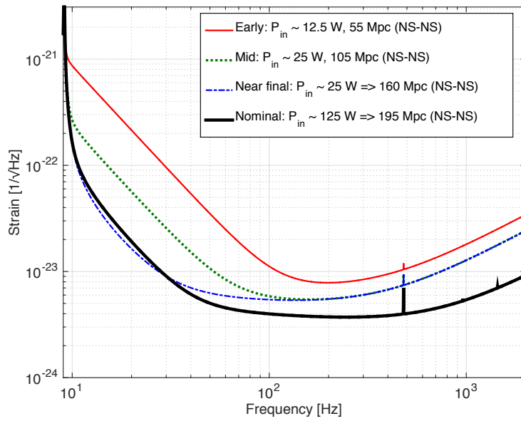
Figure 2: Strain sensitivity curves for the different stages of aLIGO. The proposed early configuration (red) is 12.5W input power all the way to 125W input power (to the PRM) for the final aLIGO configuration (black): see reference [9], from which this figure is adapted, for full details.
