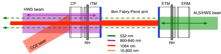
Figure 5: aLIGO TCS overview. Absorption of the main interferometer beam [1064nm] (red) in the test masses induces thermal lenses (and subsequent wavefront distortion). Hartmann wavefront sensors (HWS) probe beams, [800-840nm] (purple) and [532nm] (green), measure the thermal lens in the substrates of the ITM+CP and ETM+ERM. Ring heaters (RH), gray, encircle the test masses and radiate heat onto the barrel to induce thermo-elastic and thermo-refractive distortion. CO 2 laser beams [10,600nm] (pink) heat the CP to induce a spatially tunable thermal lens. Note that the green laser beam at the ETM is also part of the Arm Length Stabilization (ALS) system [17]. A small fraction the green laser leaks through the 4km arm (dashed green) and is used to align the ITM HWS beam to the ITM.
