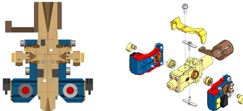
Figure 1. Left picture: cross-section of the new 2SB mixer block. The RF input horn is at the top, the LO horn at the bottom. Left and right of the hybrid are two standard ALMA band 9 mixer backpieces, below them the magnet coils. Right picture: exploded view of the new 2SB mixer, showing the way it is disassembled to replace the mixer backpieces.
