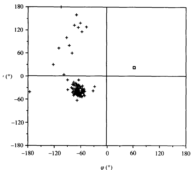
Fig. 2. The Ramachandran plot. Glycine residues are indicated by □ and non-glycines are indicated by +.
