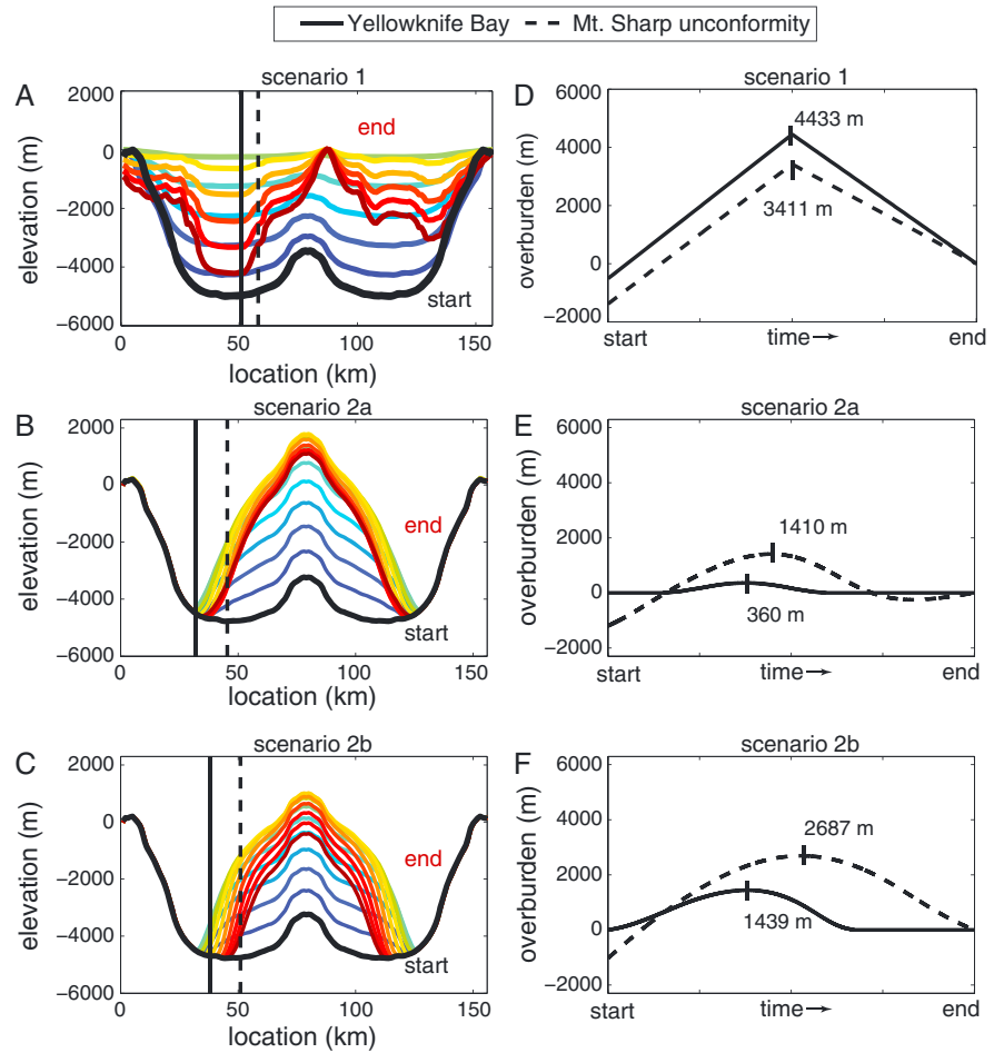
Figure 5. Topography versus time and overburden versus time for (a and d) scenario 1, (b and e) scenario 2a, (c and f) and scenario 2b. Black line shows initial topography, and the colors proceed successively from blue (early stage evolution) stage to red (present-day topography).
