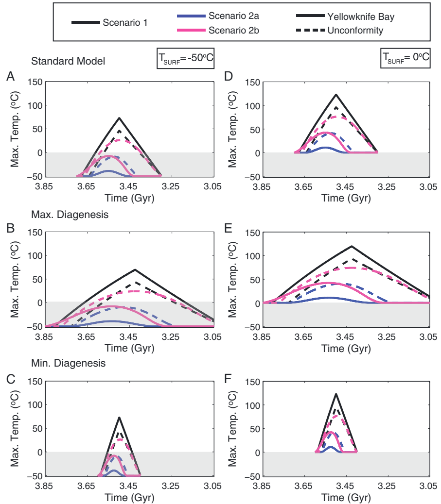
Figure 6. (a–f) Temperature as a function of timing scenarios for scenarios 1, 2a, and 2b considering an early mean surface temperature of either -50^{\circ}\text{C} or 0^{\circ}\text{C} . Solid lines represent location at Yellowknife Bay; dashed lines represent location at the Mount Sharp unconformity.
