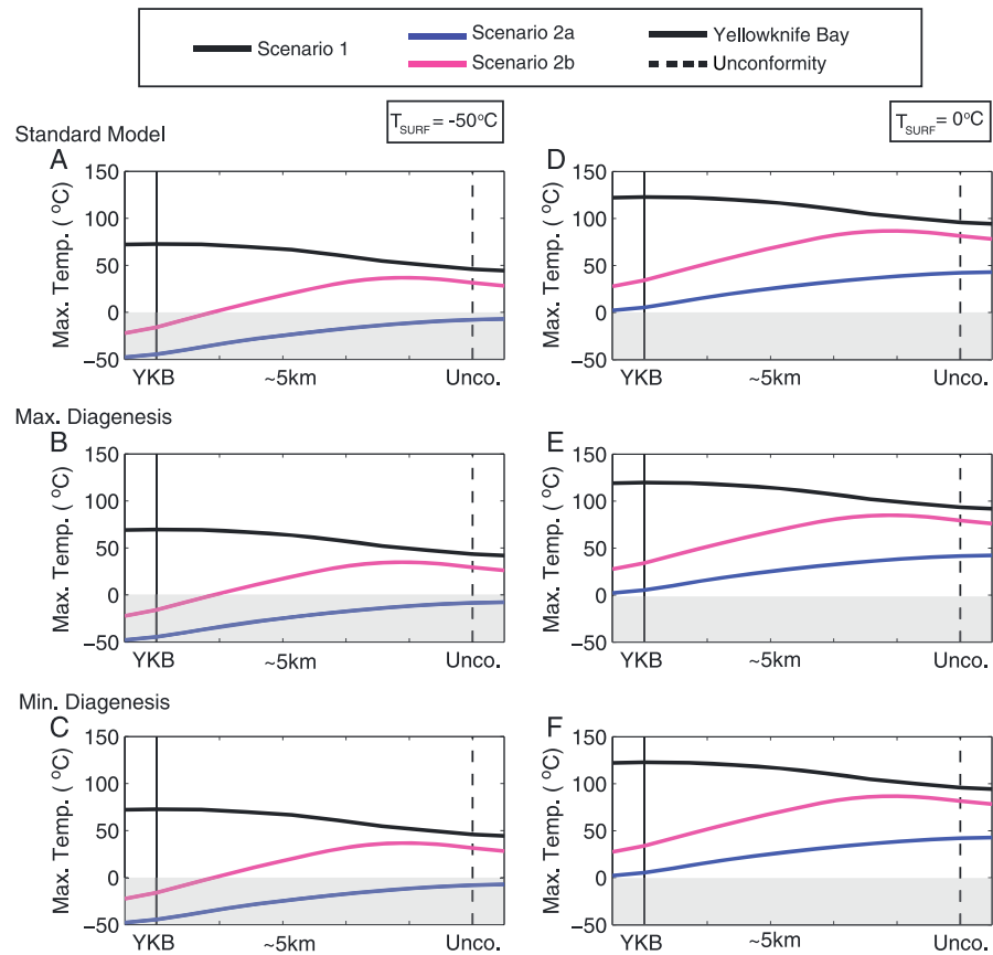
Figure 8. Maximum paleotemperatures experienced by sediments that currently crop out along MSL’s traverse, considering different sedimentary scenarios and timescales for cold and warm early Mars.
