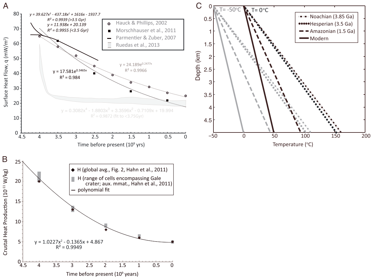
Figure 3. (a) Secular evolution of surface heat flow, q(t) , from Parmentier and Zuber [2007], Hauck and Phillips [2002], Morschhauser et al. [2011], and Ruedas et al. [2013]. The intermediate Morschhauser et al. model is utilized for the modeling results in subsequent figures. Results of q(t) sensitivity analyses are shown in Table 3. (b) Crustal heat production versus time, H(t) , as calculated by Hahn et al. [2011b, supporting information] was obtained for the two 5^{\circ} \times 5^{\circ} grid cells around Gale Crater, averaged, and then fit with a polynomial for straightforward incorporation into the model. The true functional form is a sum of exponentials. Estimated heat production near Gale Crater is similar to estimated global average values. (c) Calculated temperature versus depth relationships for two different mean surface temperatures ( 0^{\circ}\text{C} and -50^{\circ}\text{C} ) as well as four time periods using the models from Figures 3a and 3b along with equation (1).
