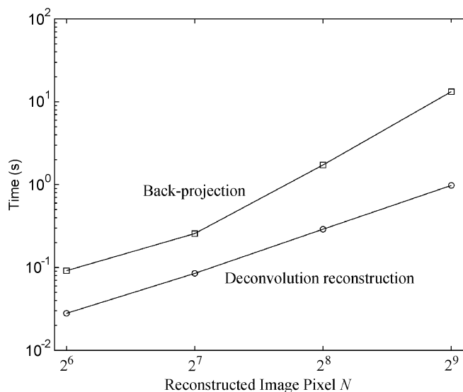
Fig. 5. Time costs of the back-projection algorithm and deconvolution reconstruction algorithm when reconstructing N \times N images using signals from N detection angles.
