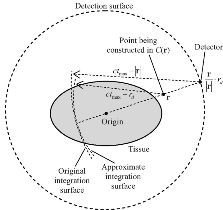
Fig. 1. Detection geometry and PA signal integration.
