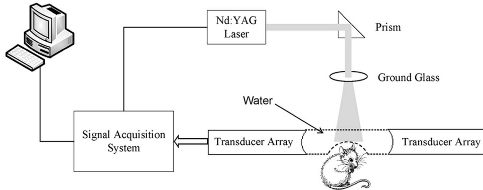
Fig. 2. Experimental setup.
