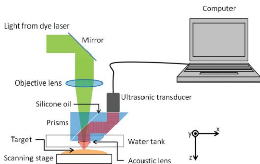
Fig. 2 System diagram of optical resolution photoacoustic microscope.
