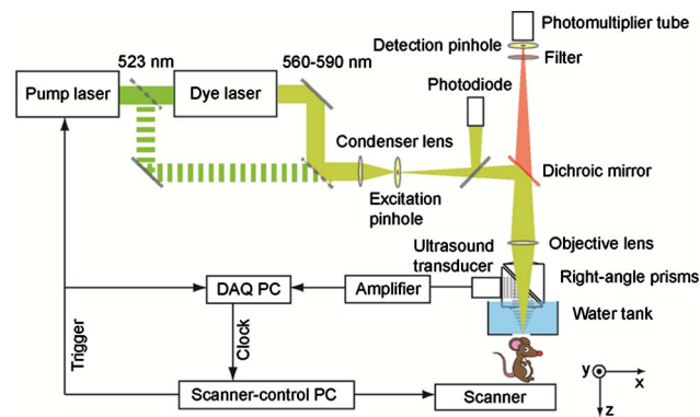
Fig. 1. (Color online) Schematic of the integrated photoacoustic and confocal microscopy setup.
