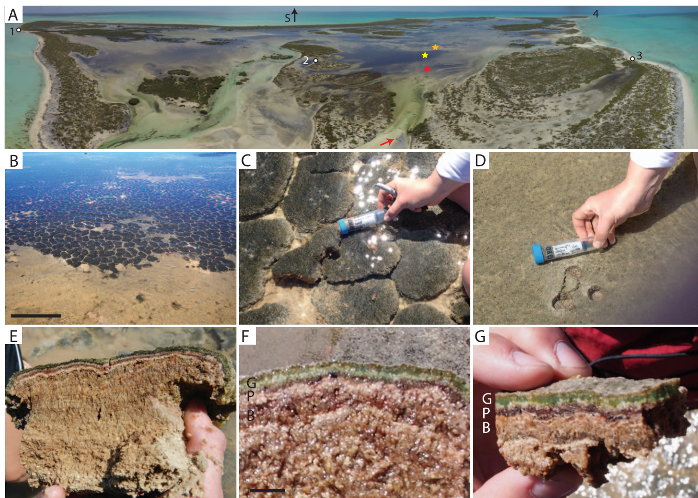
FIG. 1.— A ) UAV photo mosaic from north shore of Little Ambergis Cays over tidal marsh. Red star indicates the sampling location of flat mats, yellow star in darker region marks the sampling location of biscuit mats. Orange star indicates sediment-filled channel with no mat growth, and red arrow highlights a person for scale. White dots numbered 1–4 orient the mosaic with the following GPS coordinates: 1) 21.306231° N, 71.675926° W; 2) 21.301820° N, 71.686693° W; 3) 21.305593° N, 71.691211° W; 4) 21.297430° N, 71.725451° W. B ) Close-up of contact between and examples of flat mats (lower half of image) and biscuit mats (upper half). Black bar is approximately 0.5 m. C ) Close-up of biscuit mats in the sampled region with hand for scale. D ) Close-up of the flat mats in the sampled region with hand for scale. E ) Vertical cross-section through a biscuit mat showing shape and internal structure with hand for scale. F ) Vertical cross section through a biscuit mat showing annotated pigmentation layers (G, green; P, purple and pink; B, brown). Black bar is approximately 1 cm. G ) Vertical cross section through flat mat showing annotated pigmentation layers (G, green; P, purple and pink; B, brown). Hand is for scale.
