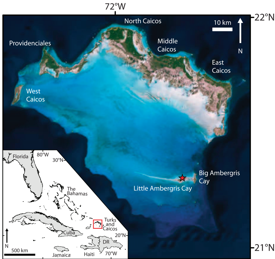
FIG. 2.—Location of study on Little Ambergris Cay within the Caicos platform. Inset shows location of Turks and Caicos with respect to the Bahamas, and neighboring Caribbean countries.
