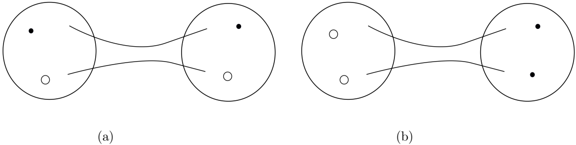
Figure 2: Illustration of geometric realization of Argyres-Seiberg duality for T_3 theory. The dots represent simple punctures while circles are maximal punctures. (a) The theory A, which is an SU(3) superconformal gauge theory with six hypermultiplets, is pictured as two spheres connected by a long tube. Each of them has two maximal and one simple punctures. (b) The theory B, which is obtained by gauging an SU(2) subgroup of the flavor symmetry of the theory T_3 . This gauge group connects a regular puncture and an irregular puncture.
