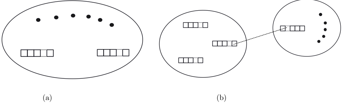
Figure 7: Illustration of the geometric realization of generalized Argyres-Seiberg duality for T_N theories. (a) The theory A' is obtained by compactifying 6d (2,0) theory on a Riemann sphere with two maximal SU(N) punctures and N - 1 simple punctures. (b) The theory B', obtained by colliding N - 1 simple punctures, is then the theory that arises from gauging a SU(N - 1) flavor subgroup of T_N by a quiver tail.
