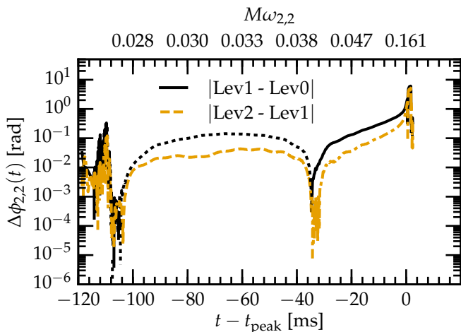
FIG. 9: Phase difference \Delta\phi_{n,m}(t) = \phi_n(t) - \phi_m(t) in the (2, 2)-mode of the GW strain r h^{2,2} during the inspiral phase of the simulation. The solid (black) line shows the phase difference between the low and medium resolution runs, while the dashed (orange) line shows the phase difference between the medium and high resolution runs. Dotted (black) and dash-dotted (orange) line segments indicate time intervals during which the phase difference \Delta\phi_{n,m}(t) is negative. The upper x -axis is labeled by the GW frequency \omega_{2,2} of the (2, 2)-mode of the GW strain of the highest resolution (Lev2) run. We observe convergent behavior in the GW phase. However, no clear convergence order can be assigned. This is most likely due to interactions between numerical errors in the finite volume hydrodynamics part and in the adaptively refined spectral metric part of the code.
