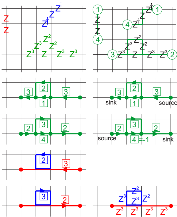
FIG. 3: Illustration of the steps towards constructing the optimal canonical path for quantum double \mathbb{Z}_5 : (a) the support of the error can be partitioned into three connected components, coloured in red, blue and green; (b) each elementary error can be interpreted as fusions, decays and moving of anyons; (c) an elementary error can be mapped onto a fully connected directed graph with weighted edges (reversing the orientation of an edge changes the weight from k to d - k ); (d) this can be interpreted as a flow of charges; (e) the flow can be partitioned into a rotational (blue) and irrotational (red) part; and (f) these different partitionings of the flow are all equivalent to applying the same combination of operators in either loops or strings.
