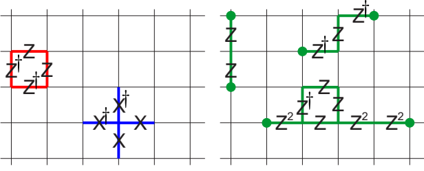
FIG. 1: (a) Star operator A(v) in blue and plaquette operator B(p) in red. (b) Examples of anyon paths for an Abelian quantum double ( d > 2 ).
