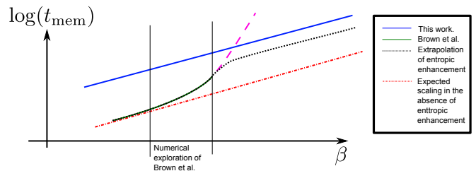
FIG. 6: Conceptual scaling of the logarithm of the quantum memory time t_{\text{mem}} as a function of the inverse temperature \beta .
