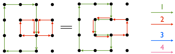
FIG. 5: Merging of loops at a qudit initially affected by three loops for the quantum double of \mathbb{Z}_5 . The weight of each edge of the graph is represented by a colour coding.
