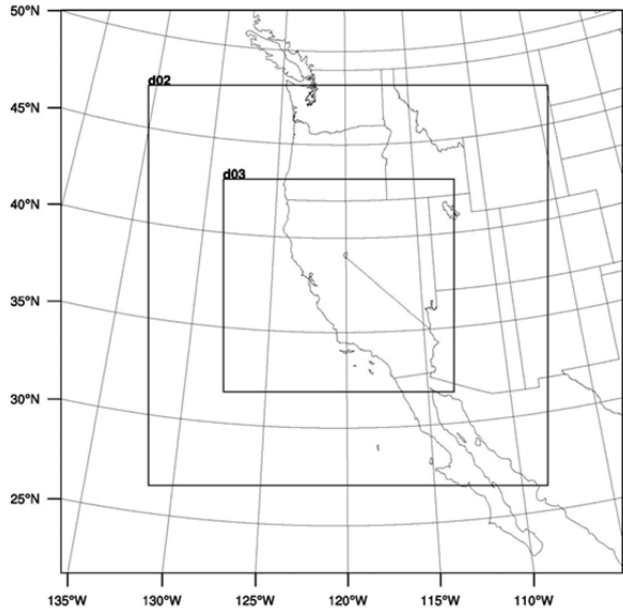
Figure S1: Nested WRF domains with 36, 12 and 4 km horizontal resolutions for domain 1 to 3, respectively.
