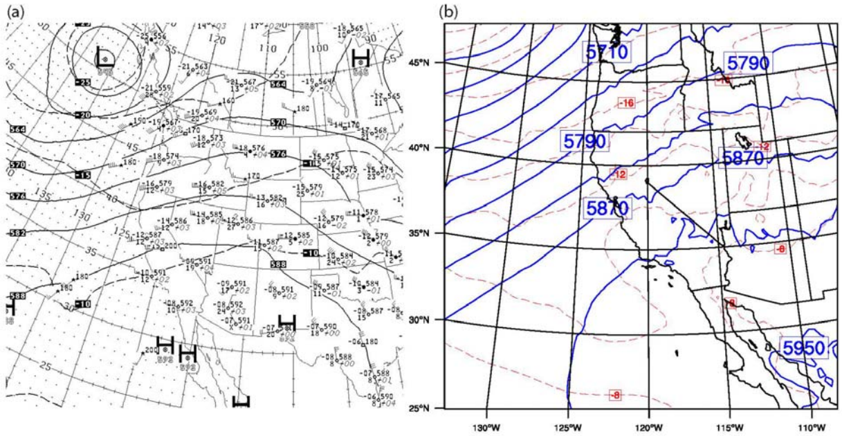
Figure S2: (a) 500 mb weather map with height (solid lines; units in m/10) and temperature (dashed lines; units in °C); (b) WRF simulated 500 mb height (blue contours; units in m) and temperature (red dashed contours; units in °C from the outermost domain (with a 36 km resolution) on June 20 2008 00 UTC.
