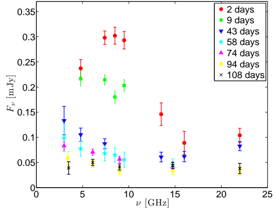
FIG. 1.— Radio spectra of GRB 130925A at various VLA observation epochs. The initial spectrum shows a peculiar cut off at frequency \geq 10 GHz. Moreover, the spectral evolution suggest the existence of an underlying (and slowly variable) constant-flux component. However, more than a year after its discovery, the radio emission from GRB 130925A faded away below our detection limit (See Table 2).
