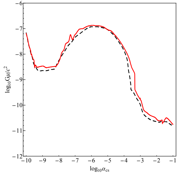
Figure 15. Exclusion limits for different cosmic string network configurations with the same \Omega h^2 value at a frequency f = 1 \text{ yr}^{-1} in the G\mu/c^2 - \alpha_{cs} parameter space, for p = 1 . Both the amplitude and spectral slope information of the GWB limits were used to construct the limits. The dashed black and solid red curves, are based on the results of models (ii) and (iii) presented in Fig. 14 respectively. In the mid- \alpha_{cs} region, the tension upper limits are provided by the n_* = 1 networks, whereas in the regime of large and small loops, by the n_* = 10^4 networks.
