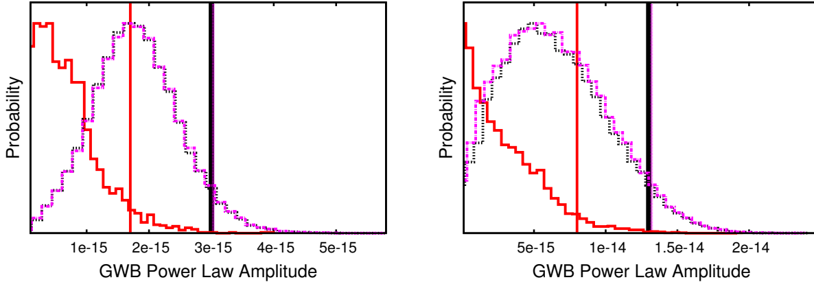
Figure 6. One-dimensional marginalised posterior parameter estimates for the amplitude of a correlated GWB in the 6 pulsar dataset presented in this paper when: (left) Fixing the spectral index of the power law to a value of 13/3, consistent with a background dominated by a population of SMBHB, and (right) when marginalising over the spectral index given a prior range of [0,7]. In each case we show the posterior given: (red solid line) Fixed intrinsic noise parameters for each pulsar, where the values of the parameters are given by the maximum likelihood estimates listed in Table 1, (black dotted line) varying noise parameters for each pulsar, and (magenta dashed line) varying noise parameters for each pulsar, and additionally including a common uncorrelated red noise process, clock errors, and errors in the Solar System ephemeris in the model. Vertical lines in each case represent the 95% upper limits for each model.
