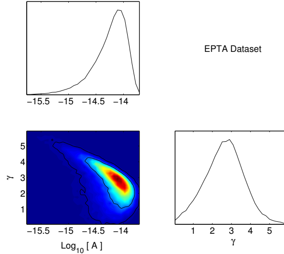
Figure 7. One and two-dimensional marginalised posterior parameter estimates for the amplitude and spectral index of a correlated GWB in the 6 pulsar dataset presented in this paper when varying the intrinsic noise parameters for each pulsar. The amplitude and spectral index are highly correlated, resulting in a significantly higher upper limit when allowing the spectral index to vary, as opposed to fixing it at a value of 13/3 .
