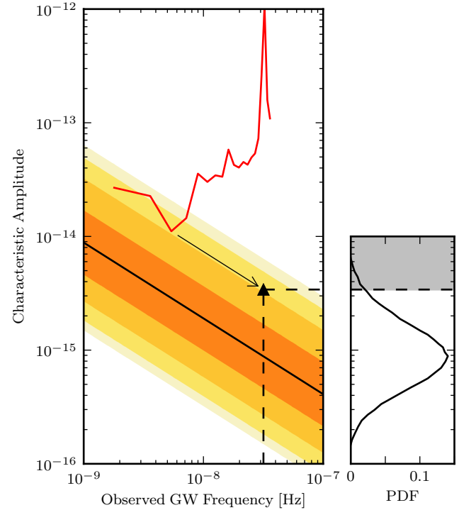
Figure 13. Comparison between the expected GWB amplitude from a cosmological population of SMBHBs and the 95% upper limit obtained with our PTA experiment. Shaded areas represent the central 68%, 95%, 99.7% and 100% confidence interval of the predicted signal according to Sesana (2013b), whereas the red curve is the 95% upper limit presented in this paper, obtained by converting the unparametrised power spectrum shown in Fig. 9 to characteristic amplitude. The black triangle is the extrapolated 95% upper limit on A at f = 1 \text{ yr}^{-1} . The right panel shows the PDF of the predicted h_c at f = 1 \text{ yr}^{-1} , and the shaded area marks the region excluded at 95% confidence by our limit (less than 5% of the distribution).
