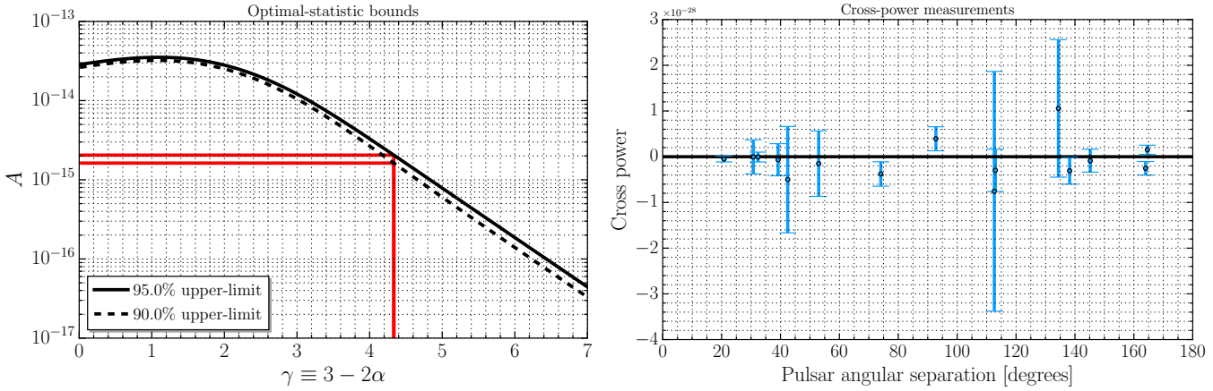
Figure 12. (left) Frequentist upper-limits on the strain amplitude of the stochastic GWB obtained via the optimal-statistic for our 6 pulsar dataset. Red lines indicate 90% and 95% upper-limits at the fiducial slope of the strain-spectrum of -2/3 , which corresponds to a slope of the residual PSD of -13/3 . (right) The individual cross-power values are shown for our 6 pulsar dataset. All values are consistent with zero cross-correlation.
