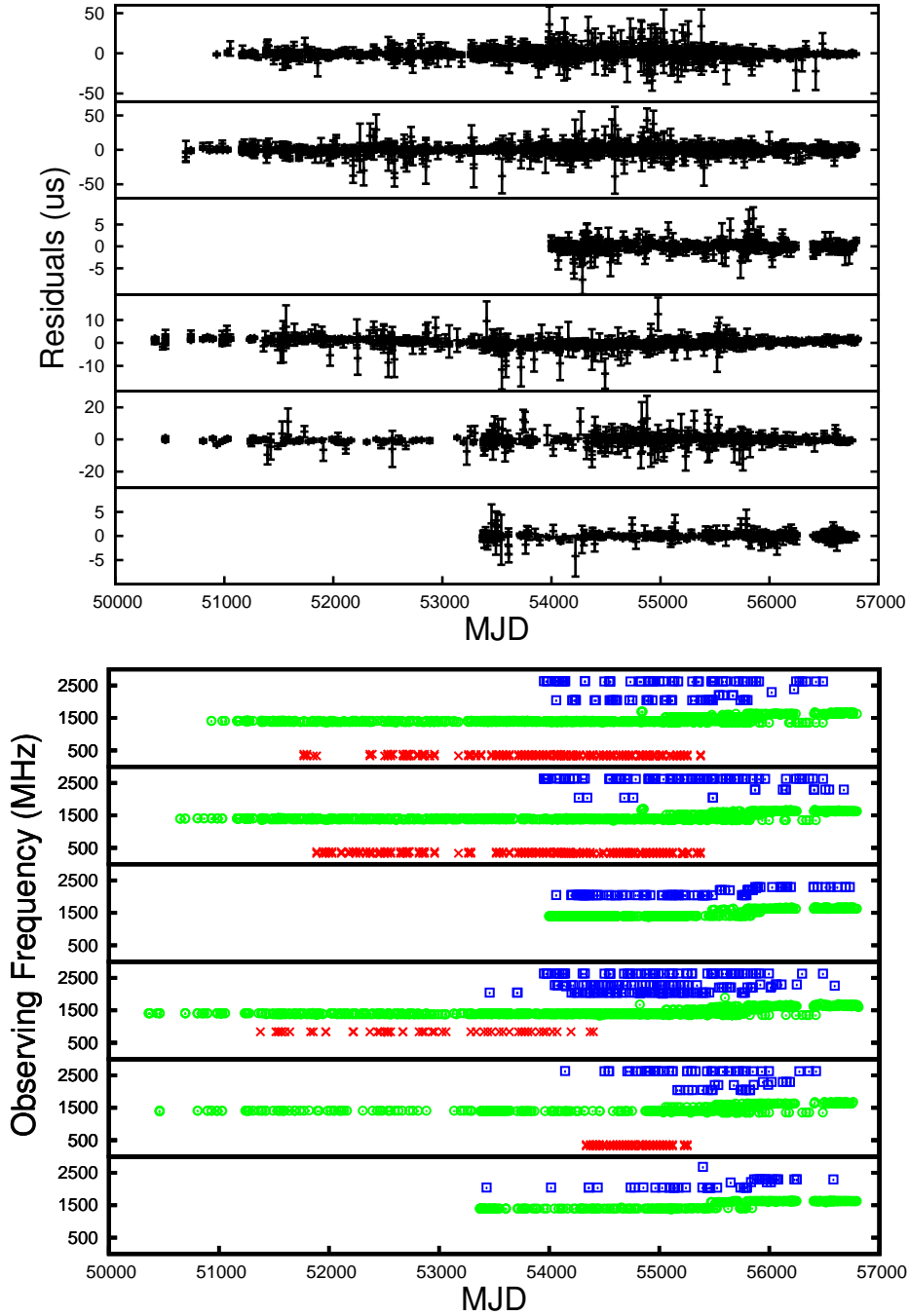
Figure 3. Top: timing residuals as a function of Modified Julian Date (MJD) for the 6 pulsars included in the stochastic GWB analysis presented in this work, after the maximum likelihood DM variations signal realisation has been subtracted. From top to bottom these are PSRs: J0613–0200, J1012+5307, J1600–3053, J1713+0747, J1744–1134, and J1909–3744. While the overall timing baseline for this dataset is \sim 18 yr, only four of the 6 pulsars have data that extends across the majority of this timespan, and in particular, PSR J1909–3744 contributes only to the latter half of the dataset, significantly reducing our overall sensitivity to signals at the lowest frequencies supported by the dataset. Bottom: Frequency coverage for the 6 pulsars included in the stochastic GWB analysis presented in this work. The order of the pulsars is as in the top plot. Colours indicate observing frequencies < 1000 MHz (red crosses), between 1000 and 2000 MHz (green circles) and > 2000 MHz (blue squares). In addition to fewer pulsars extending across the full dataset, there is also less multi-frequency coverage in the early data. This further decreases our sensitivity to a stochastic GWB at the lowest sampled frequencies as the signal becomes highly covariant with the DM variations for the individual pulsars in the first half of the dataset.
