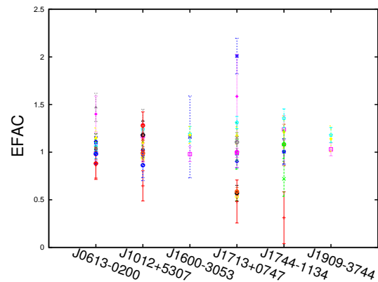
Figure 4. EFAC values obtained for all systems from the initial analysis performed for the 6 pulsars used in our analysis. All EFACs are consistent with values equal to or greater than 1 within uncertainties, with the exception of the Westerbork 1380 MHz data in PSR J1713+0747 which have values consistent with \sim 0.5 . This could be the result of systematic effects that occur in the template forming phase, and is the subject of ongoing work.
