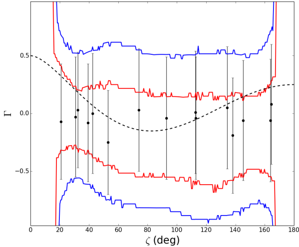
Figure 11. The recovered correlation between pulsars as a function of angular separation on the sky for a power law noise process. The red and blue lines represent the 68% and 95% confidence intervals for the correlation function when modelled by the lowest 4 Chebyshev polynomials, while the individual points are the mean correlation coefficient with 1\sigma uncertainty for each pulsar pair when fitting without assuming a smooth model. The Hellings-Downs correlation is represented by the dotted line. For both models the correlation of a common power law model between pulsars is consistent with effectively all possible values (the range [-1,1] ).
