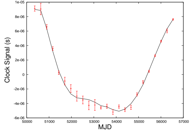
Figure 2. Simulated clock error used used in our analysis (black line) after subtracting the maximum likelihood timing models from the joint analysis, and the time averaged maximum likelihood recovered clock signal with 1\sigma uncertainties (red points with error bars). We find the recovered signal is consistent with the injected signal across the whole dataspan.
