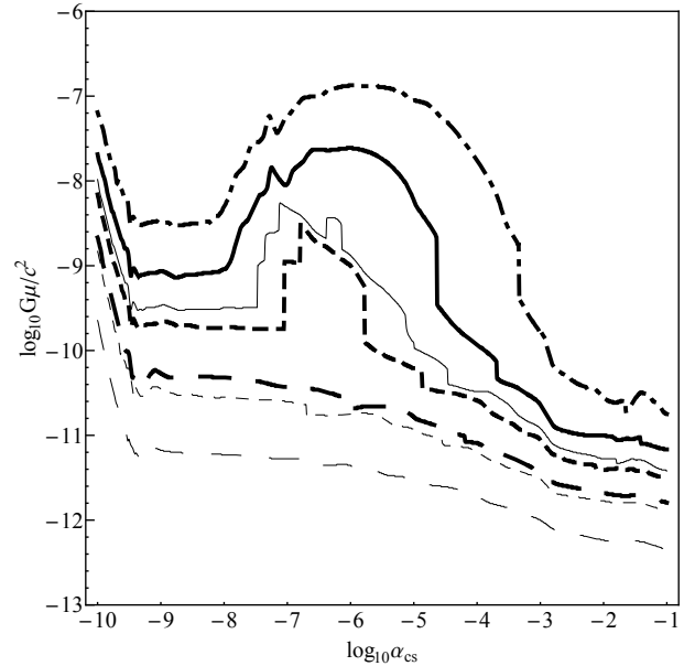
Figure 16. Exclusion curves for a set of network configurations with p \neq 1 . With thick lines are the configurations with k = 0.6 and with thin lines the configurations with k = 1 . We present exclusion curves for p = 0.1 (solid lines), p = 10^{-2} (short dashed lines) and p = 10^{-3} (long dashed lines). The dot-dashed curve is the exclusion curve for p = 1 , for reference purposes. For all the results, we used the stochastic GWB limit of model (iii), placed at a frequency f = 1 \text{ yr}^{-1} .
