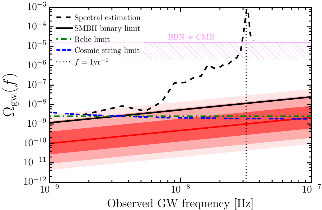
Figure 1. Summary of key results from the analysis of a 6 pulsar dataset from the 2015 EPTA data release (D15). Results are presented in terms of \Omega_{\text{gw}}(f) as a function of GW frequency, with H_0 = 70 \text{ km s}^{-1} \text{ Mpc}^{-1} . We indicate the 95% upper limits on the amplitude of a correlated GWB assuming a power law model with a spectral index of \gamma = 13/3 (solid black line; Section 5) and for a more general analysis where the power is determined simultaneously at a set of discrete frequencies (dashed line) as discussed in Section 5.1.1. The red shaded areas represent the central 68%, 95%, and 99.7% confidence interval of the predicted GWB amplitude according to Sesana (2013b) under the assumptions that a SMBHB evolves purely due to gravitational radiation reaction and binaries are circular (See Section 6.1 for more details). Only about 5% of the distribution is excluded, meaning that our limit does not place significant restrictions on the cosmic SMBHB population. We also indicate 95% upper limits obtained for a stochastic relic background (green dash-dotted line; Section 6.3), and for cosmic string network backgrounds (blue triple-dashed line; Section 6.2). The cosmic string limit plotted corresponds to a fiducial model for a population of cosmic strings, with the following parameters: string tension G\mu/c^2 = 10^{-7} , the birth-scale of loops relative to the horizon \alpha_{\text{cs}} = 1.6 \times 10^{-6} , spectral index q = 4/3 , cut-off on the number of emission harmonics n_* = 1 and intercommutation probability p = 1 . Finally we indicate recent constraints placed by CMB (Sendra & Smith 2012), and BBN (Allen 1997; Maggiore 2000; Planck Collaboration et al. 2015) observations.
