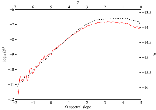
Figure 14. The 95% confidence upper limits on the amplitude of an isotropic, stochastic GW as a function of the local spectral index at the frequency of 1 \text{ yr}^{-1} , imposed by models (ii) (dashed black) and (iii) (solid red) of Section 5.1. The limits are expressed in terms of the strain of the GW, h_c , and the dimensionless spectral energy density of GWs, \Omega h^2 , where H_0 = 100h \text{ km s}^{-1} \text{ Mpc}^{-1} , as a function of their respective spectral indices.
