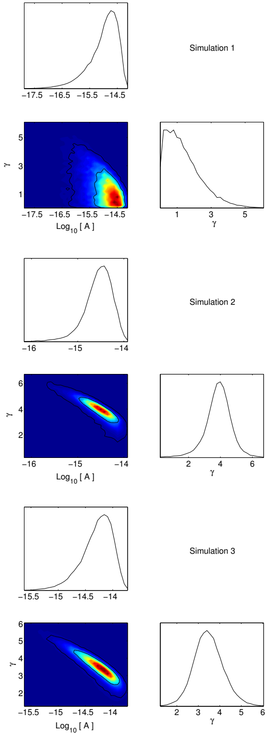
Figure 8. One and two-dimensional marginalised posterior parameter estimates for the amplitude and spectral index of a correlated GWB in 3 simulated datasets, including (Top) White noise only, (Middle) White and intrinsic spin-noise only, and (Bottom) White noise, intrinsic spin-noise, and dispersion measure variations. In each case we use the TOAs from the 6 pulsars used in the GWB analysis presented in this work, and use the maximum likelihood noise parameters from Table 1 when constructing the simulations. The upper limits obtained in each case are 4.3 \times 10^{-15} , 7.2 \times 10^{-15} , and 1.2 \times 10^{-14} . We find both the upper limit, and the form of the posterior to be consistent between the third simulation and the real dataset. In both cases we are simply recovering our uniform prior on the amplitude of the GWB signal at small amplitudes, before the data begins to place constraints on the upper limit at large amplitudes.
