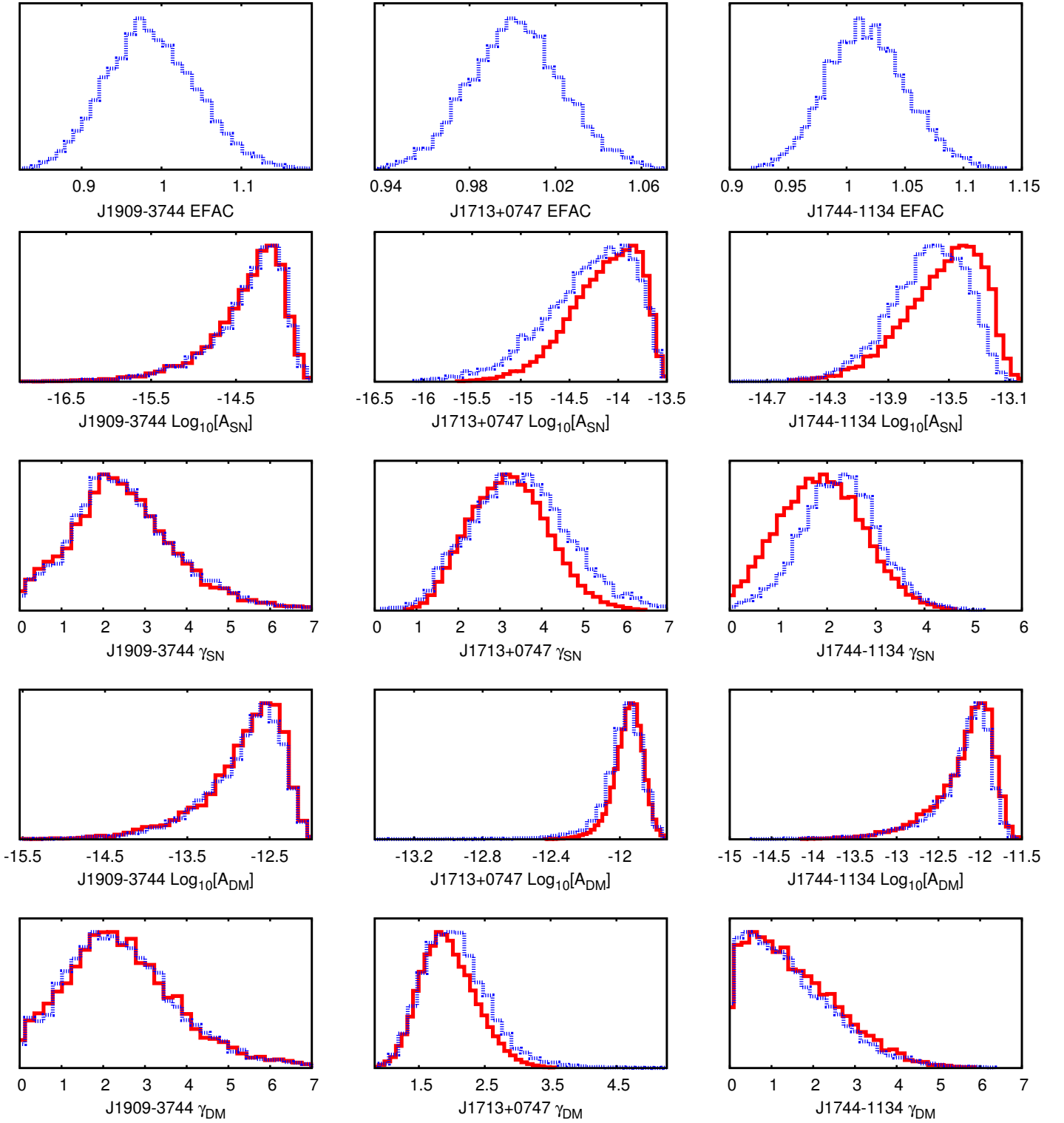
Figure 5. Comparison of the 1-dimensional marginalised posterior probability distributions for PSRs (left to right) J1909–3744, J1713+0747, and J1744–1134. The y-axis in all plots represents probability. In each case we show the spin-noise and DM variation power law parameters for the full noise analysis (red solid lines) and 5-dimensional analysis where the TOA error bars have been pre scaled by the mean value of the EFAC/EQUAD parameters for each pulsar backend (blue dashed lines). In both cases parameter estimates have been obtained using a uniform prior on the amplitude of the spin-noise and DM variations power law models. We also show the global EFAC parameters from the 5-dimensional analysis in each case. We find the posteriors are consistent between the two sets of analysis.
