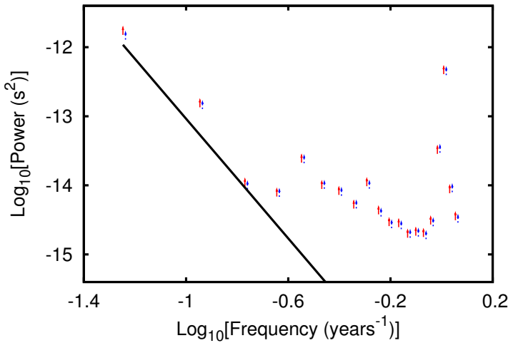
Figure 9. (Top) 95% upper limits from an unparameterised power spectrum analysis for a correlated GWB (red points), and uncorrelated common red noise process (blue points) for the 6 pulsar dataset described in Section 4 obtained while varying the intrinsic noise parameters for each pulsar. The upper limit obtained from a power law analysis of the GWB at a spectral index of 13/3 of 3 \times 10^{-15} is overplotted as a straight line. Frequencies were included from 1/T up to 20/T , with T = 17.66 yr. Beyond these frequencies the data provides increasingly poorer constraints on a steep red noise process, and so we do not consider higher frequency terms in our model. Both the correlated and uncorrelated power spectrum are completely consistent with one another at all frequencies. The difference in the log Evidence between the correlated and uncorrelated models was 0.2 \pm 0.3 , indicating no support for the presence of a correlated signal in the dataset.
