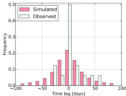
Figure 7. Distributions of observed \tau_{\text{obs}} and simulated \tau_{\text{simul}} time lags between middle points of rotations and t_p of gamma-ray flares.
