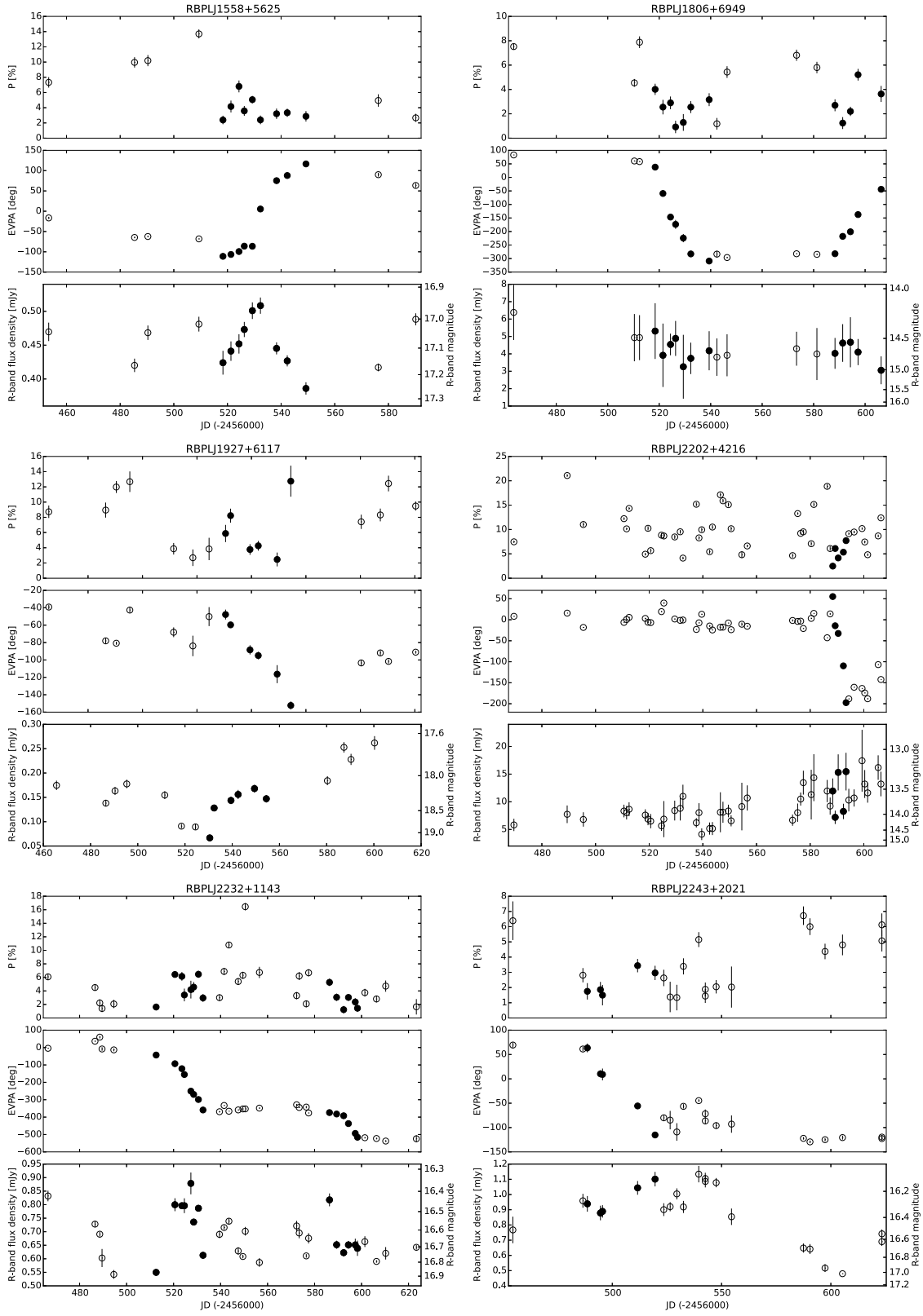
Figure 2 – continued (Continued) Evolution of polarization degree, polarization position angle and R-band magnitude for blazars with a detected rotation in the first RoboPol season. Periods of rotations are marked by filled black points.
