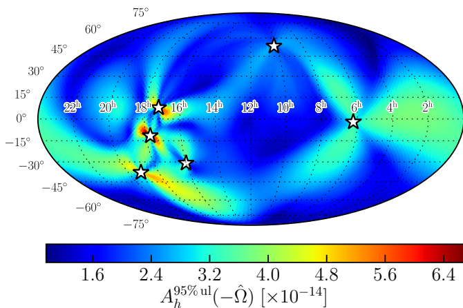
FIG. 2: 95% upper limits on the GW strain amplitude in each pixel. These limits are obtained by mapping from the Bayesian MCMC-sampled cross-correlation values to a pixelated ORF basis ( N_{\text{pix}} = 12288 ). White stars show the pulsar locations.
