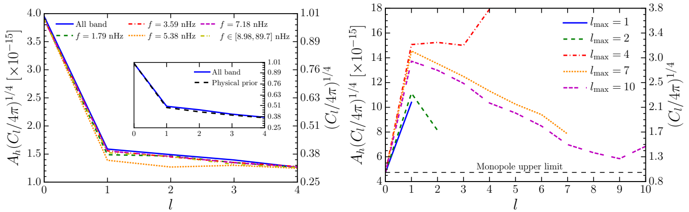
FIG. 1: 95% upper limits on the strain amplitude, where C_l = \sum_{m=-l}^l |c_{lm}|^2 / (2l + 1) . Left: all-band anisotropy parametrization and frequency-dependent parametrization (ii). The right axis is the ratio of the upper limit to the monopole. The inset figure shows 95% upper limits on (C_l/4\pi)^{1/4} which are marginalized over the strain amplitude for the all-band anisotropy parametrization and a constant likelihood analysis. Our limits reflect the constraints of the physical prior. Right: all-band anisotropy parametrization , where the c_{lm} values are obtained by mapping cross-correlation values to the spherical harmonic basis, without physical prior rejection.
