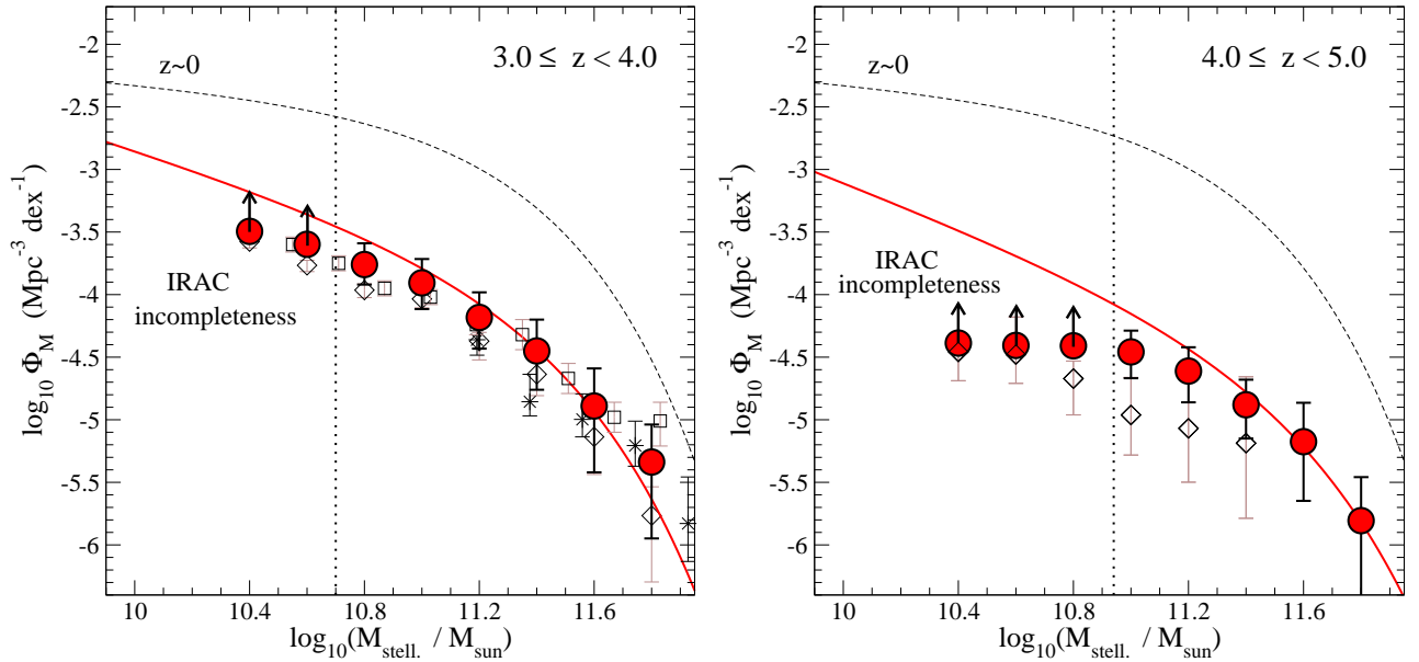
FIG. 5.— The GSMF at 3.0 \leq z < 4.0 (left) and 4.0 \leq z < 5.0 (right), obtained by considering the results of previous K_s < 24 surveys and the new [4.5] < 23 , K_s > 24 galaxies analysed here. The circles correspond to the GSMF computed with the V/V_{\max} method. Other symbols correspond to the other previous K_s < 24 surveys: diamonds (Caputi et al. 2011), squares (Ilbert et al. 2013) and asterisks (Muzzin et al. 2013). All V/V_{\max} data points correspond to a Salpeter IMF over (0.1 - 100) M_{\odot} , and the stellar masses from Caputi et al. (2011) have been multiplied by a factor of 1.24 to obtain a crude conversion from BC07 to BC03 templates. The solid red line in each panel indicates the resulting GSMF obtained with the STY maximum likelihood analysis, assuming a single Schechter function. This maximum likelihood analysis has been performed on a combination of Caputi et al. (2011) sample and the new galaxies analysed in this paper. The vertical dotted line in each panel indicates the stellar mass completeness limit imposed by the IRAC [4.5] = 23 magnitude cut. The dashed line indicates the local GSMF (Cole et al. 2001).
