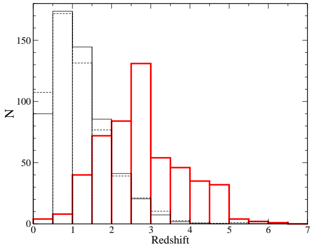
FIG. 2.— Redshift distribution of our [4.5] < 23 , K_s > 24 sample (thick solid histogram). For a comparison, we also show the renormalised redshift distributions of the [4.5] < 23 , K_s < 24 galaxies (thin solid histogram), and all K_s < 24 galaxies (thin dashed histogram).
