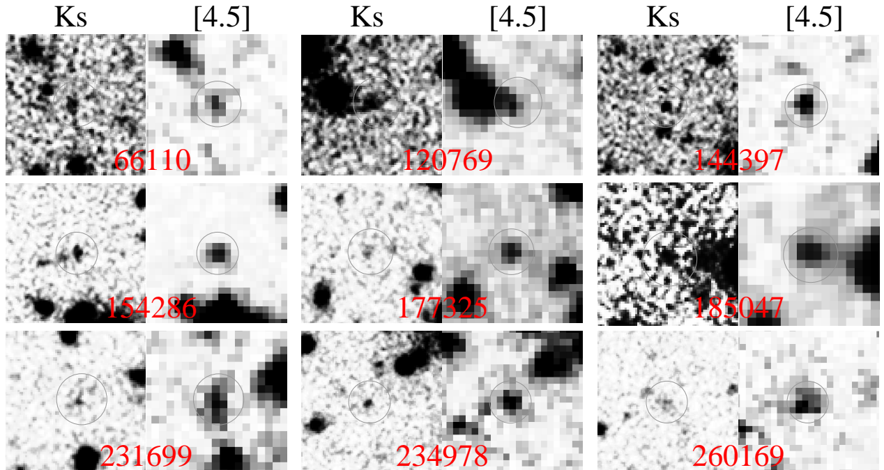
FIG. 9.— K_s and 4.5\ \mu\text{m} postage stamps of our z \geq 5 galaxy candidates. The field shown in each stamp is of \sim 12 \times 12\ \text{arcsec}^2 .
