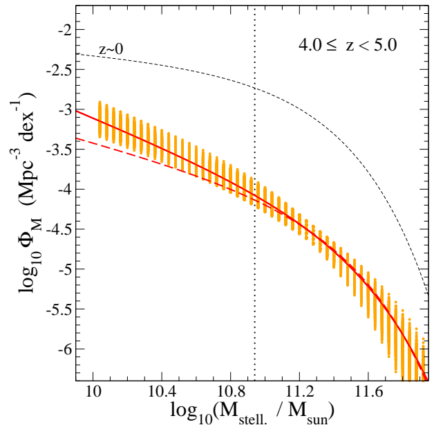
FIG. 8.— Different GSMF at 4.0 \leq z < 5.0 obtained from 100 mock galaxy catalogues. The red solid line indicates the GSMF obtained applying the STY maximum likelihood analysis on our real sample. This plot shows that the uncertainty on the GSMF produced by the z_{\text{phot}} and stellar mass errors is non-negligible, especially at the lowest and highest stellar masses. The long-dashed line corresponds to the Eddington-bias corrected GSMF.
