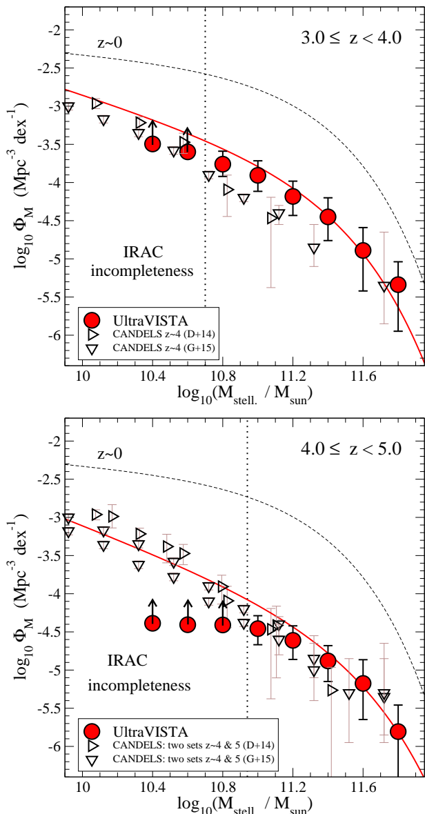
FIG. 6.— The GSMF obtained in this paper at 3.0 \leq z < 4.0 and 4.0 \leq z < 5.0 , compared to those obtained with datasets from the CANDELS survey (Duncan et al. 2014; Grazian et al. 2015). No GSMF determination is available for CANDELS at z < 4 , so we only show the z \sim 4 results in the upper panel. As in Fig. 5, the vertical dotted line in each panel indicates the stellar mass completeness limit imposed by our IRAC magnitude cut. Stellar masses correspond to a Salpeter IMF over (0.1 - 100) M_{\odot} in all cases.
