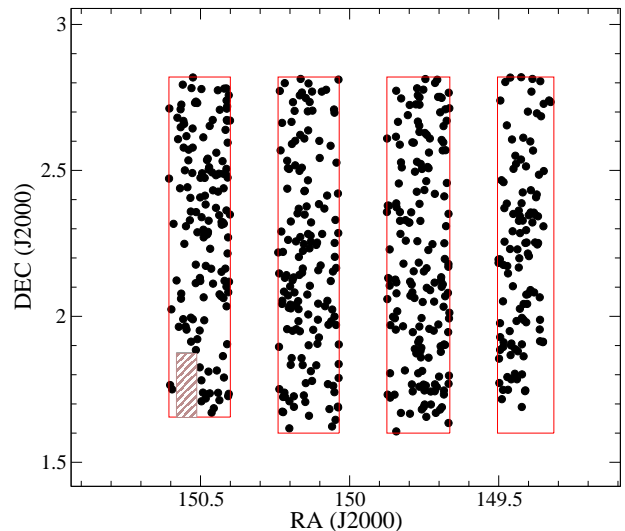
FIG. 1.— Distribution of our [4.5] < 23 sample with K_s > 24 counterparts in the UltraVISTA/COSMOS field, where the red rectangles indicate the UltraVISTA ultra-deep stripes.
