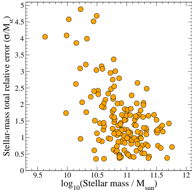
FIG. 7.— The total relative error on the stellar mass versus the stellar mass for the 3.0 \leq z < 5.0 galaxies in our sample. In most cases, these errors are dominated by the uncertainties in the photometric redshifts. The stellar mass relative errors at fixed redshift only have a contribution of \sim 0.35 , while most total values are quite larger than this number.
