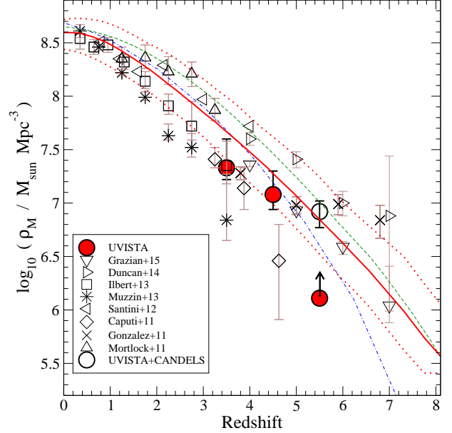
FIG. 13.— The redshift evolution of the cosmic stellar mass density, given by our new GSMF determinations and a compilation of recent results from the literature. At 3 \leq z < 5 , our stellar mass density values have been computed by integrating the best STY Schechter functions obtained here at stellar masses \log_{10}(M) > 10^8 M_{\odot} (after correction for Eddington bias). At 5 \leq z < 6 , we only sum up the contributions of our galaxies in the stellar mass bins above the IRAC completeness limit (see Fig. 11), so the stellar mass density constitutes a lower limit. The open circle indicates our best estimate of the total stellar mass density at 5 \leq z < 6 , taking into account the results of the CANDELS survey and our own, in complementary stellar-mass regimes. We include also different model predictions: solid and dotted lines correspond to the mean and 99% confidence interval in Lu et al. (2014); the dashed and dotted-dashed lines correspond to mean values in Somerville et al. (2012) and Croton et al. (2006), respectively. All stellar mass density values in this plot refer to a Salpeter IMF over (0.1 - 100) M_{\odot} .
