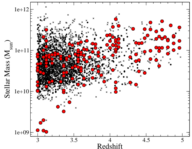
FIG. 4.— Estimated stellar masses versus photometric redshifts for our [4.5] < 23 , K_s > 24 galaxies at 3 \leq z < 5 (red filled circles). The data points in the background indicate [4.5] < 23 , K_s < 24 galaxies from two different samples: the UDS sample analysed by Caputi et al. (2011) (small black dots) and the UltraVISTA DR1 sample analysed by Ilbert et al. (2013) (cross-like symbols). The stellar masses derived by Caputi et al. (2011) have been multiplied by a factor of 1.24 to obtain a crude conversion from BC07 to BC03 templates, while the Ilbert et al. (2013) stellar masses have been multiplied by a factor of 1.7 to convert from a Chabrier to a Salpeter IMF over (0.1 - 100) M_{\odot} .
