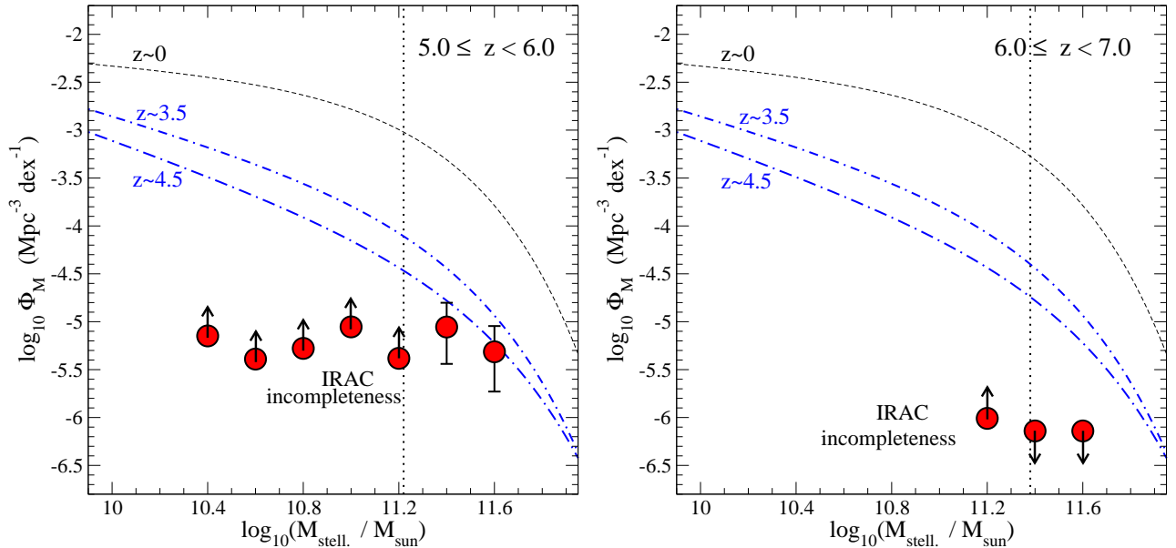
FIG. 11.— The GSMF high-mass end at 5.0 \leq z < 6.0 (left) and 6.0 \leq z < 7.0 (right). For the GSMF at 5.0 \leq z < 6.0 , we considered the combination of all UltraVISTA sources in the DR1 release, and our new sources with [4.5] < 23 , K_s > 24 over the UltraVISTA ultra-deep stripes. The GSMF constraints at 6.0 \leq z < 7.0 are based on our single z > 6 candidate (as no z \geq 6 galaxies were identified in the UltraVISTA DR1) and upper limits obtained from the absence of very massive galaxies in the UltraVISTA ultra-deep area. Note that with our sample selection cut at [4.5] < 23 , we only aim at constraining the highest-mass end of the GSMF at these high redshifts.
