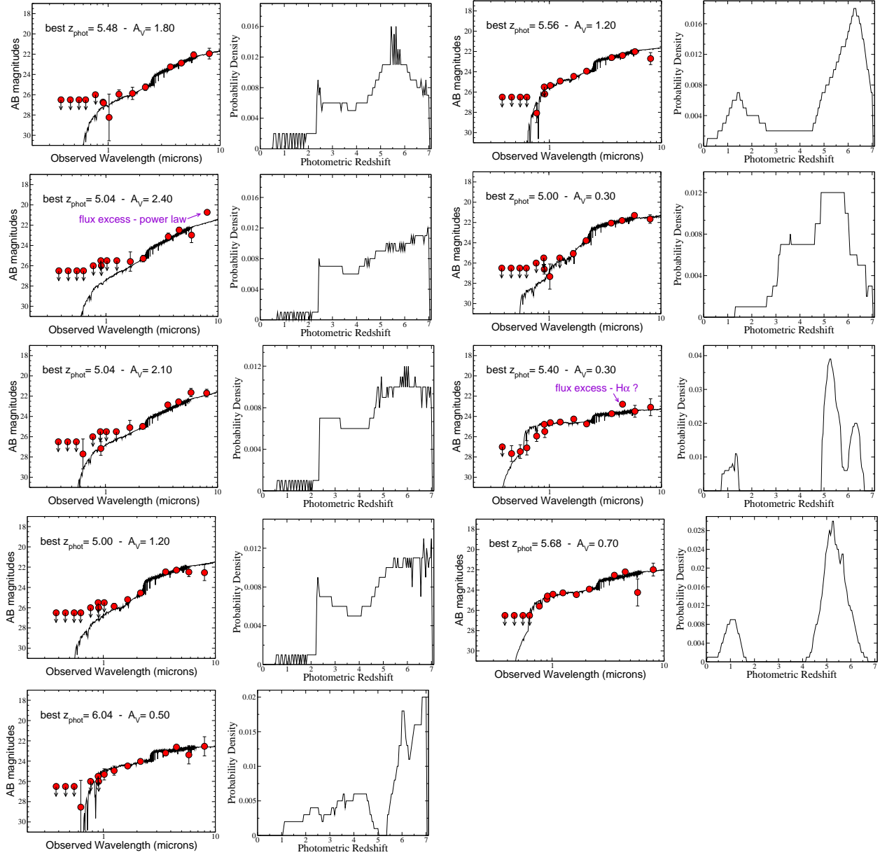
FIG. 10.— Best SED fittings and marginalized probability density distributions P(z) versus z for our z \geq 5 galaxy candidates. For clarity, only the broad-band photometric data points are shown in the SEDs.
