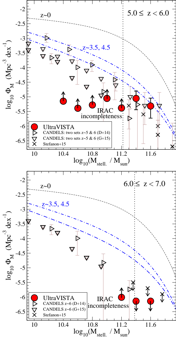
FIG. 12.— GSMF constraints provided by our sample at 5.0 < z < 7.0 , in the context of the results obtained in the CANDELS survey (Duncan et al. 2014; Grazian et al. 2015), and the upper limits obtained by Stefanon et al. (2015), at similar redshifts. As in fig. 5, the vertical dotted line indicates the stellar mass completeness limit imposed by our IRAC magnitude cut. Stellar masses correspond to a Salpeter IMF over (0.1 - 100) M_{\odot} in all cases.
