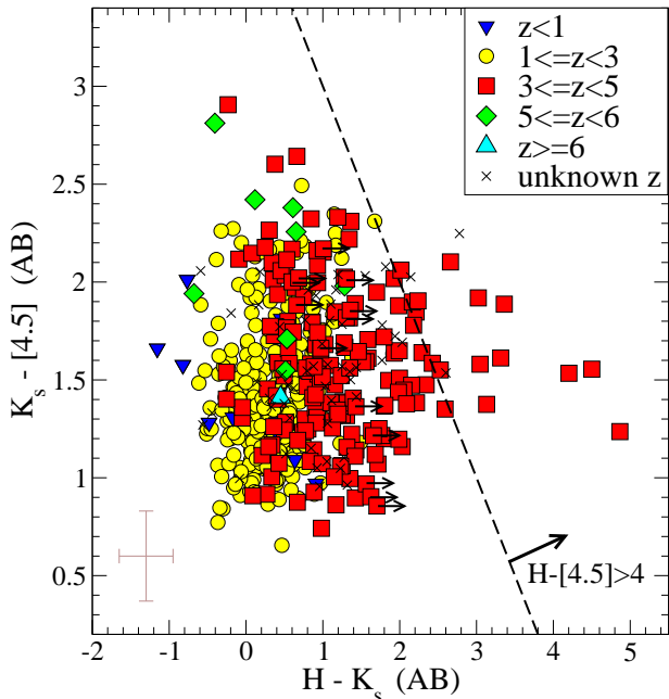
FIG. 3.— K_s - [4.5] versus H - K_s colour-colour diagram for our [4.5] < 23 , K_s > 24 sources at different redshifts. The dashed line delimits the region corresponding to H - [4.5] > 4 colours, which is the colour-cut imposed for the sample selection in Caputi et al. (2012).
