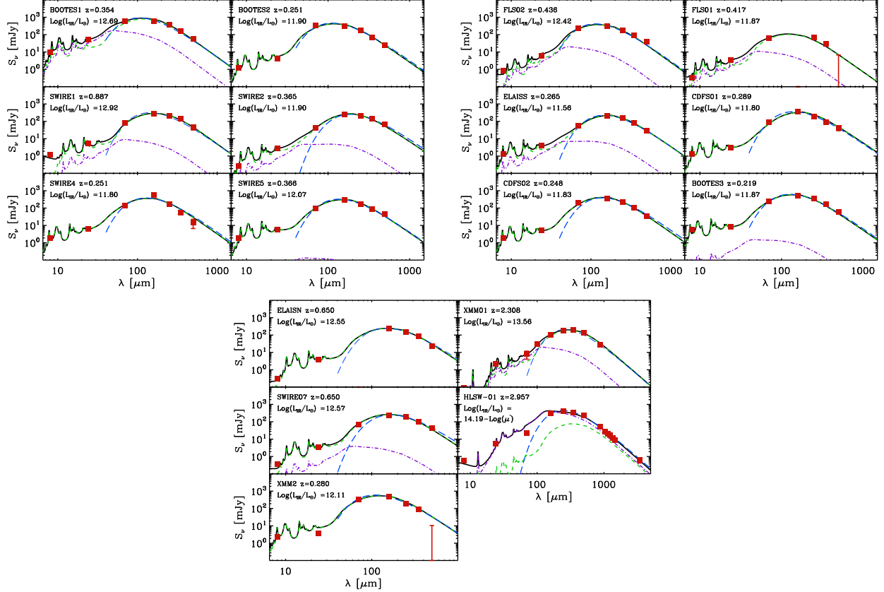
FIG. 4.— Spectral energy distributions (observed frame) of sources from our sample, including IRAC 8\mu\text{m} , MIPS 24 , 70 and 160\mu\text{m} (where available) and SPIRE 250 , 350 and 500\mu\text{m} observed data points (red squares). The observed data are overlaid with the best-fit DL07 model (black line). The “PDR” and diffuse ISM components are shown in purple and green, respectively. The dashed blue line is the best-fit modified blackbody model with \beta = 1.5 . For XMM01 and HLSW-01 we also include (sub)mm photometry from Fu et al. (2013) and Conley et al. (2011), respectively.
