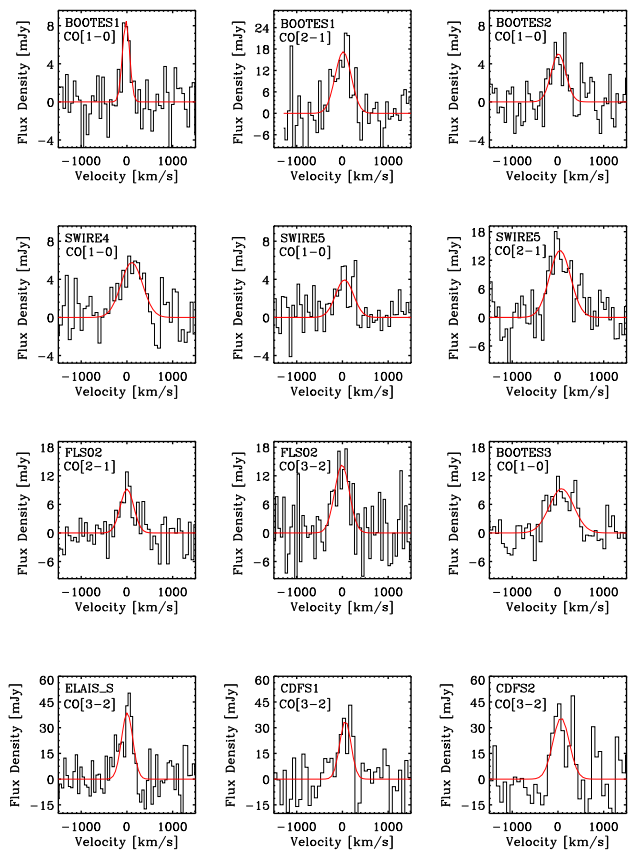
FIG. 3.— CO spectra of the detected galaxies in 50\text{--}60 \text{ km s}^{-1} bins. Zero velocity corresponds to the CO-determined redshift, listed in Table 4. According to the redshift, the lowest frequency observable is either the CO[1-0] or CO[2-1] or CO[3-2] line. The vertical scale is the flux density in mJy. The last row depicts spectra obtained by APEX, while the rest were obtained by IRAM.
