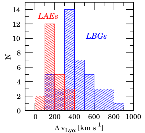
Figure 9. Histograms of Ly \alpha velocity offset for the 22 LAEs in this study and literatures (McLinden et al. 2011; Finkelstein et al. 2011; Hashimoto et al. 2013; Guaita et al. 2013; Chonis et al. 2013), and 41 LBGs given by Steidel et al. (2010).
