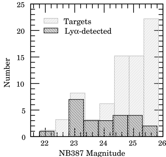
Figure 1. Success rate in identifying a Ly \alpha emission line in the LRIS spectroscopy as a function of NB387 magnitude. The gray histogram shows the number of targeted LAEs. The black histogram indicate the number of LAEs with a Ly \alpha detection. The histogram of targeted LAEs is slightly shifted for clarity.
