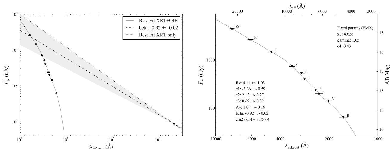
Figure 4. Late-time SED of GRB 120119A inferred from our light-curve model extrapolated to 38.7 min after the burst (Table 1). Values were corrected for the host redshift ( z = 1.728 ) and Galactic extinction ( A_V = 0.288 mag). Left panel: The dashed line and light grey cone represent the best-fit value and uncertainty (respectively) of \beta inferred from the XRT spectrum alone using the products of Butler & Kocevski (2007): \beta_{\text{XRT}} = 0.78 \pm 0.12 . The solid grey curve shows the best-fit dust model (FMX; \chi^2/\text{dof} = 8.9/4 ), and the dotted line is the \beta inferred from that fit. Right panel: Zoomed in SED highlighting the Optical/NIR points. The horizontal bars at each point show the FWHM of the corresponding filter. The solid grey curve shows the best-fit dust model (FMX).
