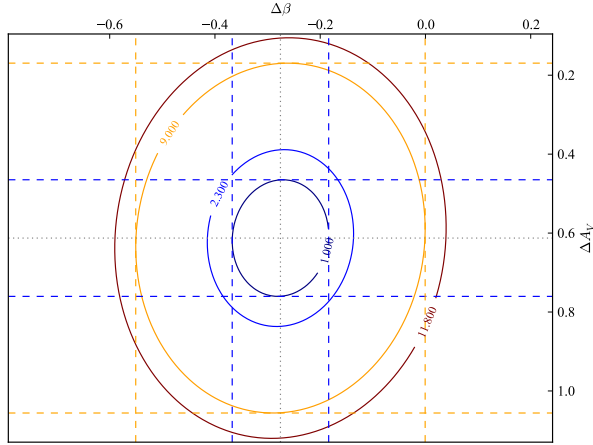
Figure 8. Covariance between parameters \Delta A_V and \Delta\beta from Equations 3 and 4. These parameters correspond to the total change in the values of A_V and \beta over the course of the light curve (i.e., a value of \Delta A_V = 0 would be consistent with no change in the amount of dust). The outer blue ellipse ( \Delta\chi^2 = 2.3 ) and the outermost red ellipse ( \Delta\chi^2 = 11.8 ) show the 68.3% and 99.73% confidence intervals for two degrees of freedom. The dotted blue and orange lines show the projections for a further marginalization to a single parameter of interest, corresponding to the 1\sigma and 3\sigma confidence intervals for \Delta A_V and \Delta\beta alone.
