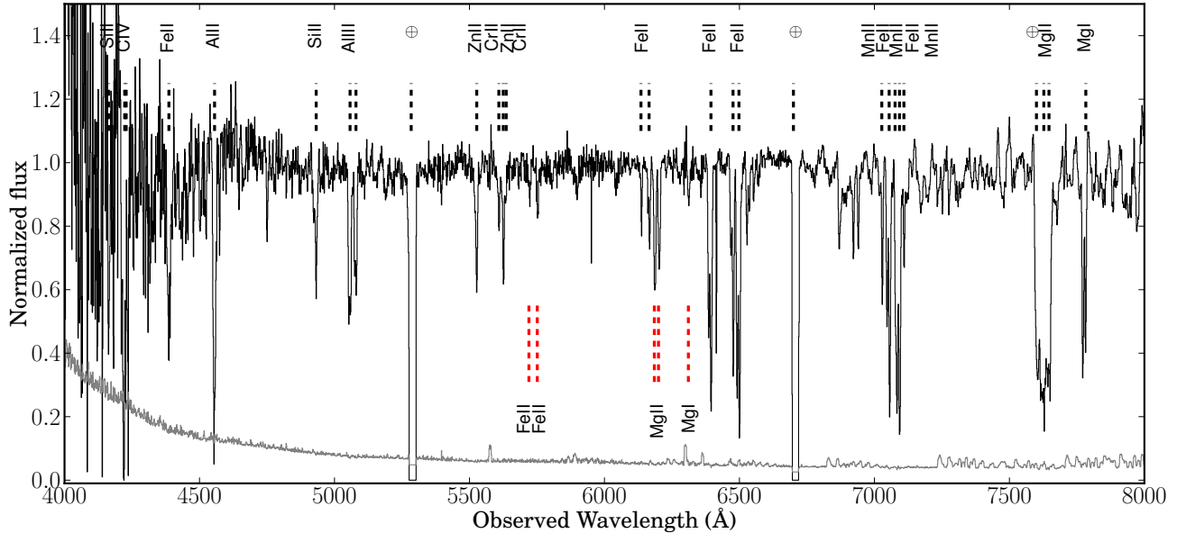
Figure 1. Normalized, combined spectrum of GRB 120119A obtained with GMOS-South. Two systems of absorption features are clearly identified. Indicated in black are the host-galaxy ( z = 1.728 ) metal lines, while in red we see a strong Mg II absorber at z = 1.212 , based on Mg II and Fe transitions. At the bottom, we show the noise spectrum.
