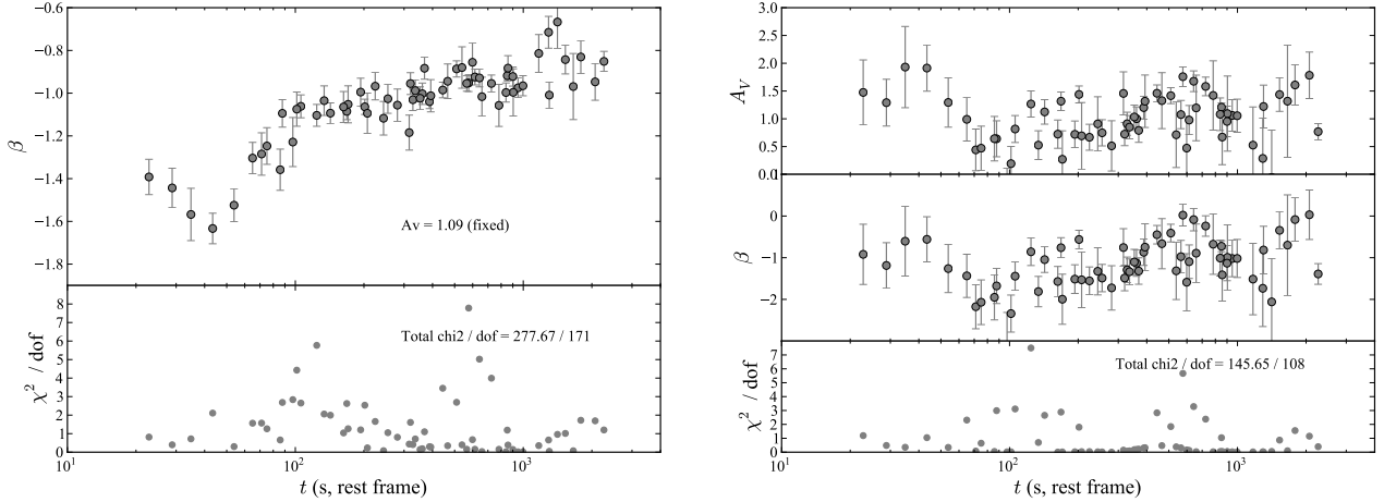
Figure 6. Left panel: The best-fit values of \beta for each interpolated SED as a function of time. The extinction A_V was fixed to the late-time value of 1.09 and FMX-like dust was assumed (see §3.2). Plotted below is the reduced \chi^2 statistic for each individual fit. Right panel: Same as the left panel, but where both A_V and \beta were allowed to vary freely.
