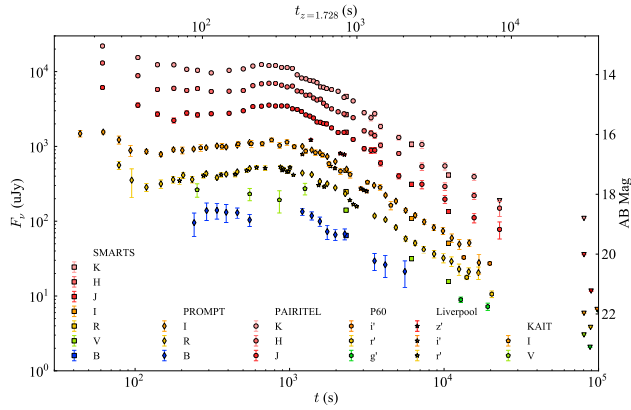
Figure 2. First-day optical/NIR light curve of GRB 120119A. A significant red-to-blue colour change is observed during the first 200s after the trigger. An achromatic rise is seen around 800s after the trigger, followed by some mild undulations before settling to a single power-law decay with index \alpha_{\text{oir}} = -1.30 \pm 0.01 . Unfiltered data are not included in this plot. The upper and lower time-axis scales refer to the rest frame and the observed frame, respectively.
