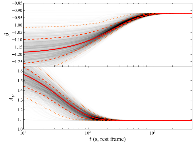
Figure 7. Best-fit values for A_V(t) (mag) and \beta(t) according to the functional forms of Equations 3 and 4, simultaneously fit to all available data at each SED interpolation point. FMX-type dust was assumed (§3.2). Light-grey lines show the resultant curve from one of the 1500 samples drawn from the multivariate normal distribution from the best-fit model. The mean value is plotted in red, with confidence contours overlotted with dashed lines (containing 68% of the curves) and dotted lines (containing 95% of the curves).
