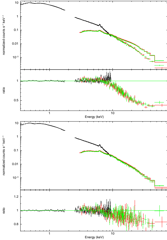
Figure 5. Upper panel: The XMM-Newton 0.3-10 keV spectrum and best fit model extrapolated to the NuSTAR 3-79 keV spectra. Here, the model is composed of a power law, reflection components, Gaussian iron lines, and a second, steeper power law to reproduce the soft X-ray excess. Lower panel: The same, but with a cutoff power law for the soft excess.
