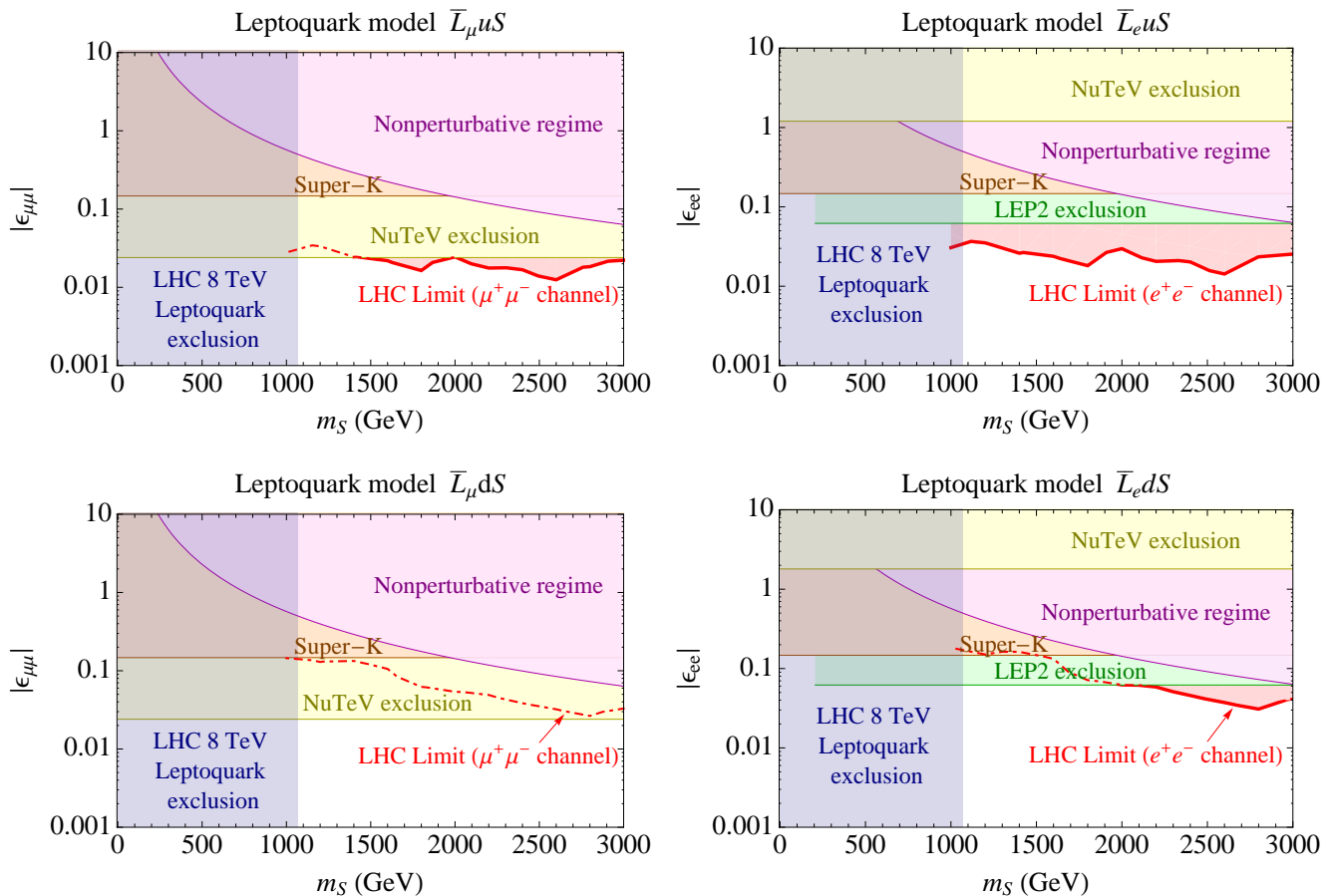
FIG. 1. Red curves: upper bounds on |\epsilon_{\mu\mu}| (left) and |\epsilon_{ee}| (right) from LHC data on \mu^+\mu^- , e^+e^- pair production rates, in \bar{L}uS (first row) and \bar{L}dS (second row) leptoquark models. The blue region is the LHC exclusion of the mass of leptoquark from its pair production and decays. The yellow region is excluded by NuTeV experiment on neutrino-quark scatterings. The orange region is excluded by the Super-K experiment as mentioned in the introduction. The LEP2 exclusion on |\epsilon_{ee}| from e^+e^- \rightarrow u\bar{u} channel is the green region. The magenta region is non-perturbative regime when the leptoquark coupling |\lambda_{\alpha i}| > \sqrt{4\pi} , ( \alpha = e, \mu , i = u, d ). All shaded regions are excluded.
