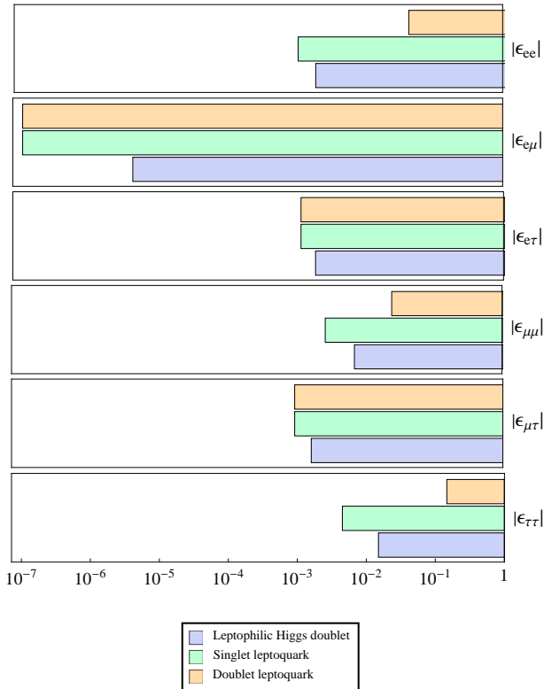
FIG. 2. Summary of constraints on |\epsilon_{\alpha\beta}| in various simple renormalizable BSM models for non-standard neutrino interactions. Shaded bands represent excluded values of epsilons for different models. We would like to highlight that for the doublet leptoquark model one of the diagonal elements \epsilon_{\alpha\alpha} can still be “large”, i.e. , \sim 10^{-2} for \epsilon_{ee} , \epsilon_{\mu\mu} , and \sim 10^{-1} for \epsilon_{\tau\tau} .
