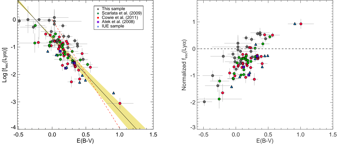
Fig. 10. Ly \alpha escape fraction as a function of the nebular dust extinction. The figure shows the z \sim 0.3 Ly \alpha emitters of this work with black circles. We also derived f_{\text{esc}}(\text{Ly}\alpha) for other galaxy samples: z \sim 0 IUE sample represented by blue triangles, z \sim 0.3 sample of Scarlata et al. (2009) with green circles, Cowie et al. (2011) sample with red circles, z \sim 0 galaxies of Atek et al. (2008) with purple squares. Note that the negative values of E(\text{B-V}) are shown in the plot but were assigned E(\text{B-V})=0 before f_{\text{esc}}(\text{Ly}\alpha) calculation or fitting the f_{\text{esc}}-E(\text{B-V}) relationship. The left panel shows f_{\text{esc}}(\text{Ly}\alpha) as a function of E(\text{B-V}) assuming a Cardelli et al. (1989) extinction law. The solid black line denotes the best 2-parameter fit to the relationship with both the slope and the intercept as free parameters. The yellow region covers the 1\sigma uncertainties of the fit derived from MC simulations. The dashed red line is the expected attenuation law at the Ly \alpha wavelength. In the right panel we plot the normalized escape fraction f_{\text{esc,rel}}(\text{Ly}\alpha)=\log[f_{\text{esc}}(\text{Ly}\alpha)/f_{\text{esc}}(\text{cont})] as a function of extinction. The normalized escape fraction represents the deviation of f_{\text{esc}}(\text{Ly}\alpha) from the classical dust attenuation law at 1216 Å. The color code for the samples is the same as in the left panel.
