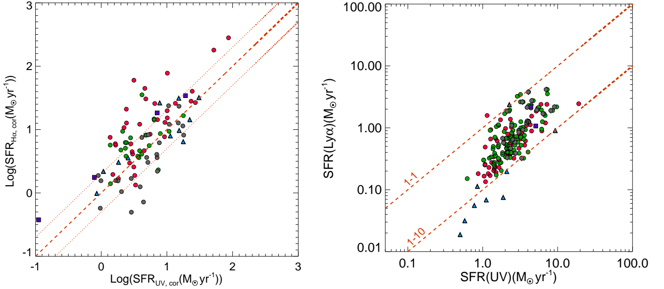
Fig. 11. Comparison between SFR indicators. The SFR values are calculated using Kennicutt (1998) calibration. The left panel shows SFR(H \alpha ) versus SFR(UV) both corrected for dust extinction derived from the Balmer decrement. The dashed line denotes the line of equality, while the dotted lines have a factor of 2 deviation. The right panel presents the observed SFR(Ly \alpha ) as a function of SFR(UV), with no correction for dust extinction. The two dashed lines marks the 1:1 and 1:10 ratios for SFR _{Ly\alpha} :SFR _{UV} . The symbols are the same as in Fig. 10.
