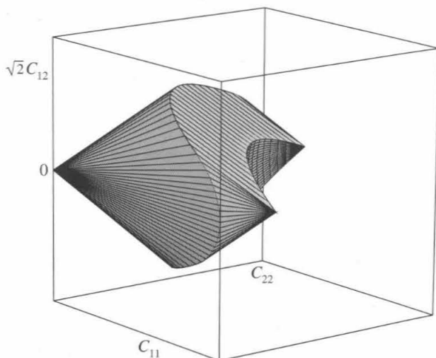
Figure 6. The set (O(2)U_1 \cup O(2)U_2)_{\mathbb{C}}^{\text{qc}} for the diagonal matrices U_1 = \text{diag}(a, b) and U_2 = \text{diag}(b, a) . This is also equal to the set (SO(3)\hat{U}_1 \cup SO(3)\hat{U}_2)_{\mathbb{C}}^{\text{qc}} for the diagonal matrices U_1 = \text{diag}(a, b, c) and U_2 = \text{diag}(b, a, c) .
