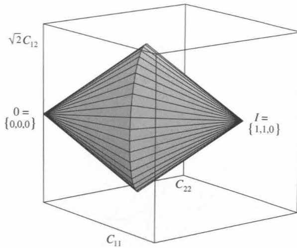
Figure 3. The quasiconvex hull K_c^{qc} for K = O(2) .
