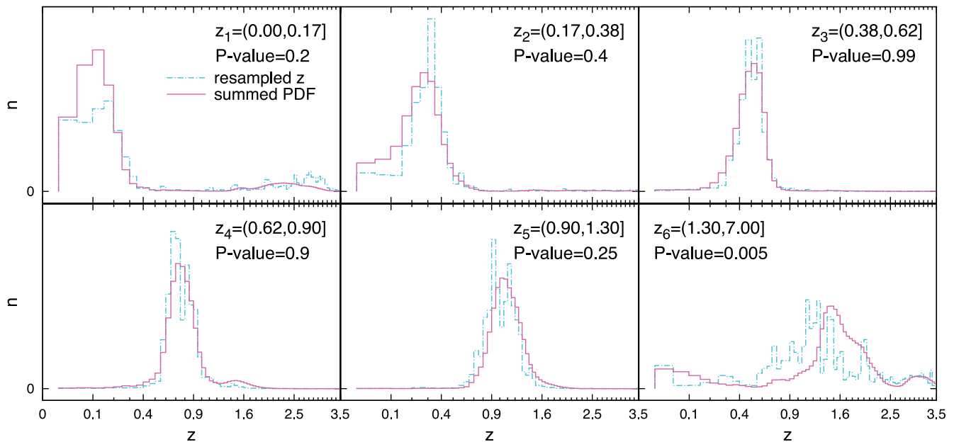
Figure 2. Comparison of the predicted redshift distributions with a magnitude cut of i' < 24.7 . The solid lines (pink) show the summed PDFs for all galaxies within a given redshift bin. The dot-dashed histogram (cyan) shows the result of resampling the CFHTLenS redshifts using the constructed conditional probability P(z_{30}|z_p) . The P -values are the result of a KS test; we reject the null hypothesis for the highest redshift bin at \alpha = 0.05 .
