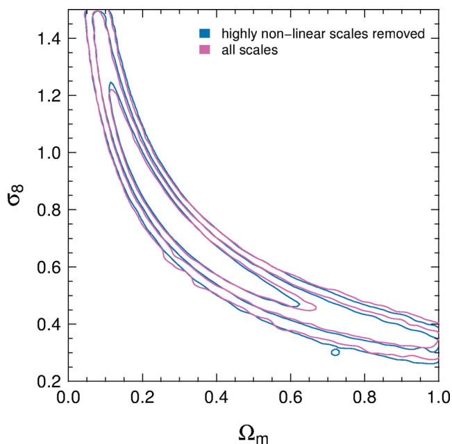
Figure 12. Marginalized parameter constraints (68.3, 95.5 and 99.7 per cent confidence levels) in the \Omega_m - \sigma_8 plane for a flat \Lambda CDM cosmology. The pink contours show the result when all eight scales are included; this is the same as the result for CFHTLenS shown in Fig. 7. The blue contours show the result of removing highly non-linear scales, which are possibly biased due to the non-linear correction to the matter power spectrum or the effect of baryons. We remove the five smallest scales of \xi_{-} , corresponding to \theta < 10 arcmin. The contours are only slightly different, indicating that we are not sensitive to these effects given the level of precision of our results.
