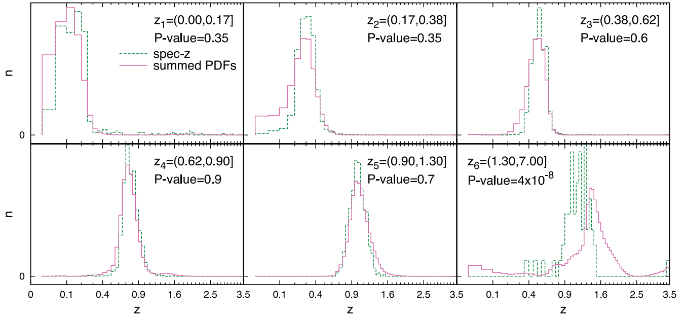
Figure 1. Comparison of the predicted redshift distributions within each broad redshift bin, labelled z_i . A magnitude cut of i' < 23.0 is used for comparison with spectroscopic redshifts. The solid lines (pink) show the summed PDFs for all galaxies within a given redshift bin. The dashed lines (green) show the spectroscopic redshift distribution. The listed P -values are the result of a two-sample Kolmogorov–Smirnov test of the distributions; we adopt a significance level of \alpha = 0.05 rejecting the null hypothesis that the two distributions are drawn from the same population for the highest redshift bin.
