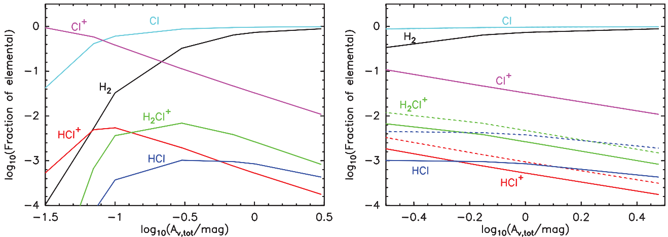
Figure 6. Left: abundance of the Cl-bearing molecules, chlorine atom or ion (X), normalized relative to the gas-phase chlorine abundance, \bar{f}(X) = N(X)/N(\text{Cl}) , obtained with the Meudon PDR code, \text{Cl}^+ (magenta), Cl (cyan), HCl (blue), \text{HCl}^+ (red), and \text{H}_2\text{Cl}^+ (green) together with the \text{H}_2 fractions (black), \bar{f}(X) = 2N(\text{H}_2)/(2N(\text{H}_2) + N(\text{H}_1)) , averaged along the line of sight, as a function of total visual extinction A_{v,\text{tot}} . The initial density is n_{\text{H}} = 316 \text{ cm}^{-3} , and the radiation field intensity is 10. Right: comparison of the predicted fraction of gas-phase chlorine present in HCl, \text{HCl}^+ , \text{H}_2\text{Cl}^+ , Cl, and \text{Cl}^+ assuming a branching ratio of 90% for chlorine and 10% for hydrogen chloride (solid lines) and the predicted fractions for a reduced branching ratio of 56% for chlorine (dashed line).
