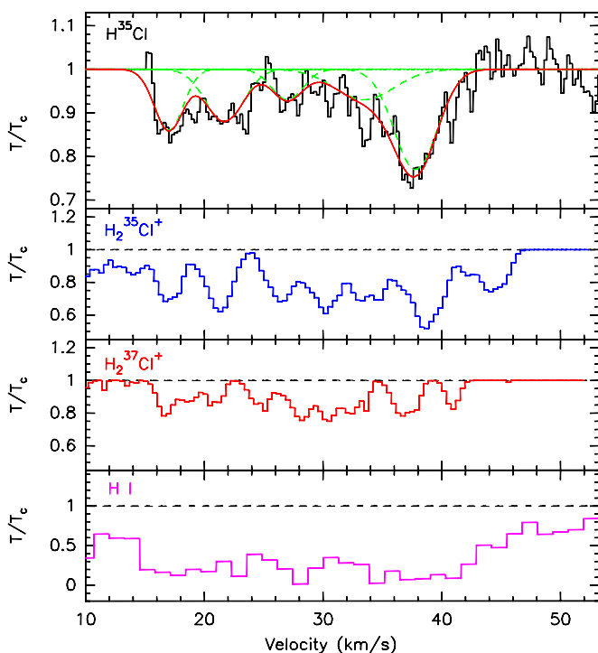
Figure 5. Top panel: multiple Gaussian fits (red) to the hyperfine deconvolved spectrum of \text{H}^{35}\text{Cl} J = 0-1 (black) associated with foreground clouds on the line of sight toward W31C. For comparison, we show the HFS deconvolved spectra of \text{H}_2^{35}\text{Cl}^+ (blue), \text{H}_2^{37}\text{Cl}^+ (red) from Neufeld et al. (2012), and H I (magenta) from Fish et al. (2003).
