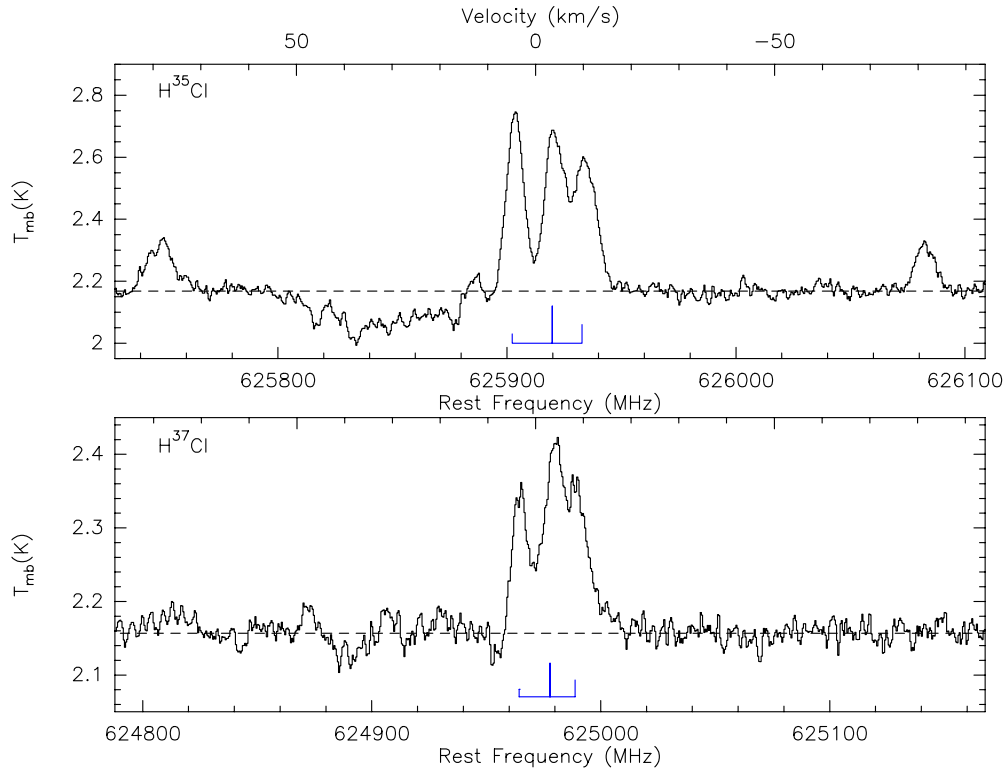
Figure 1. Spectra of the J = 1-0 transition of \text{H}^{35}\text{Cl} (upper panel) and \text{H}^{37}\text{Cl} (lower panel) toward W31C. The velocity scale in the upper axis is with respect to the frequency of the main ( F = 5/2-3/2 ) hyperfine component of both isotopologues. The blue lines indicate the position of the HFS components. (A color version of this figure is available in the online journal.)
