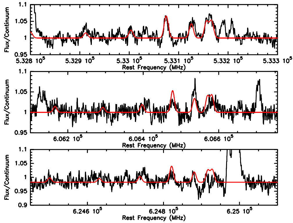
Figure 3. LTE model of \text{CH}_3\text{CN} (red), using \text{CH}_3\text{CN} transition lines J = 29-28 (upper panel) at 533.123 GHz, J = 33-32 (middle panel) at 606.533 GHz, and J = 34-33 (lower panel) at 624.878 GHz. The fit parameters are shown in Table 1. (A color version of this figure is available in the online journal.)
