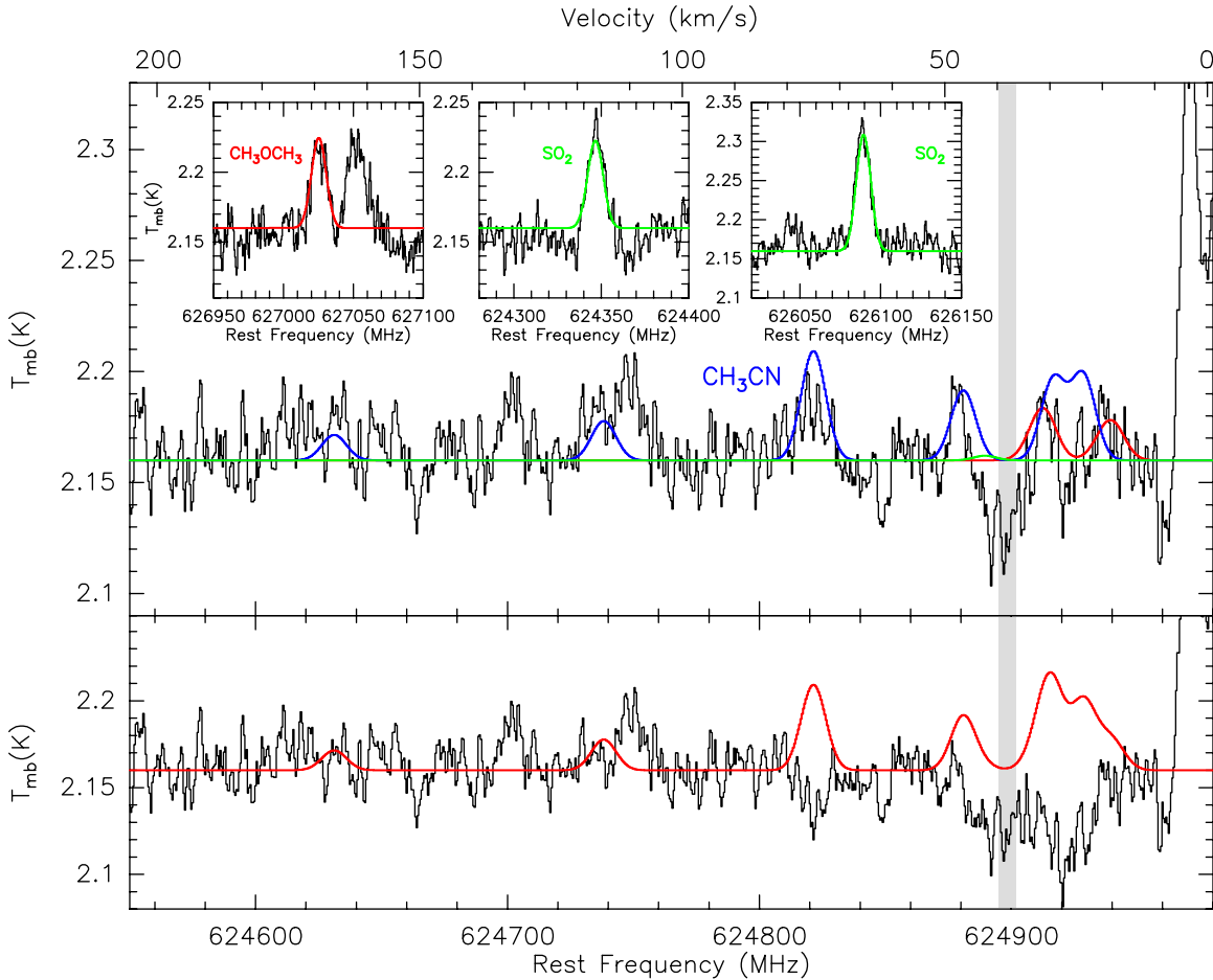
Figure 2. Upper panel: XCLASS LTE models of the dimethyl ether (red), methyl cyanide (blue), and sulfur dioxide (green) emission lines blended into the \text{H}^{37}\text{Cl} absorption line spectrum, using the parameters given in Table 1. Additional lines (within the observations bandwidth) used in the model are shown in small windows at the top of the plot. The horizontal axis is in frequency units, with the corresponding velocity scale plotted on the top horizontal axis for consistency with Figure 1. Lower panel: for illustration purposes only; shows the resulting \text{H}^{37}\text{Cl} spectrum (black) after subtracting the contamination from emission lines shown in red. The gray area highlights the emission line contamination-free area within the \text{H}^{37}\text{Cl} absorption line spectrum.
