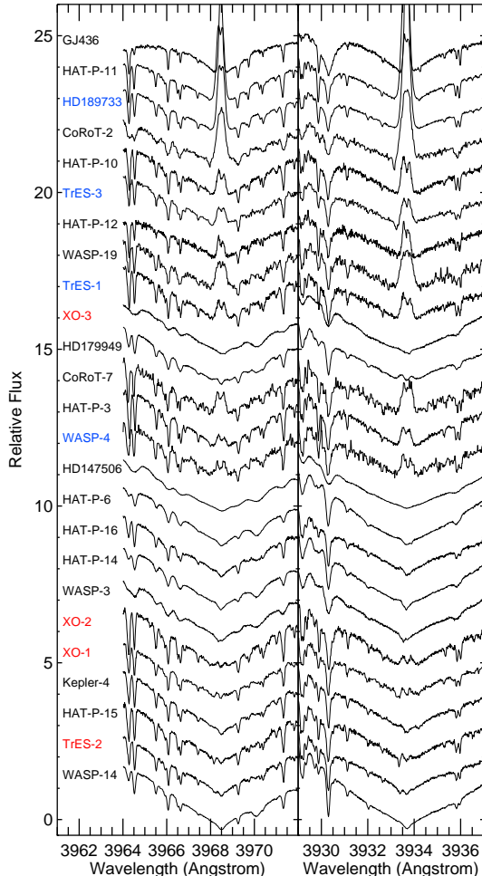
Figure 1. Ca II H & K lines for transiting planet host stars observed with Keck/HIRES, plotted in order of increasing S_{HK} . This plot shows half of our sample, with the second half plotted in Fig. 2. Active stars have significant emission in the line cores (high values of S_{HK} ) and lie at the top of the plot; a majority of the stars in our sample appear to have no detectable emission. Star names are given on the left, with systems hosting planets with temperature inversions shown in red and those without temperature inversions shown in blue, while names in black denote systems with insufficient data. It is possible that cooler ( < 1000 K) and/or higher density planets, such as the Neptune-mass planets GJ 436 and HAT-P-11, may not fit into the simple classification scheme used to describe hot Jupiters atmospheres (indeed this appears to be the case for GJ 436; Stevenson et al. 2010), but we include HIRES observations in this plot where available for completeness.
