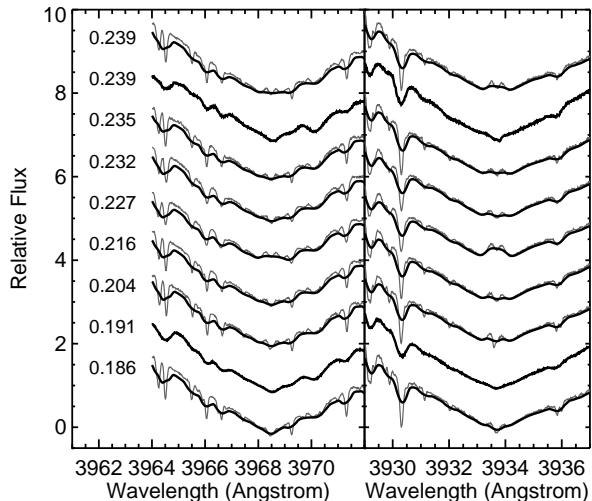
Figure 3. Ca II H & K lines for a sample of seven F stars observed with Keck/HIRES as part of ongoing CPS programs, plotted in order of increasing S_{HK} (values given on left). These stars were selected to have effective temperatures between 6000 – 6500 K, v \sin i less than 10 \text{ km s}^{-1} , and S_{HK} values in the range 0.18–0.24, comparable to the values measured for XO-3 ( S_{HK}=0.239 ) and HD 147506 ( S_{HK}=0.191 ). The original spectra (thin grey lines) for these stars were then artificially broadened to a v \sin i of 20 \text{ km s}^{-1} (thick black lines), comparable to that of XO-3 (second from top) and HD 147506 (second from bottom) which are plotted for comparison. The effective temperatures for the stars shown in this plot are, from bottom to top, 6170, 6080, 6260, 6090, 6130, 6090, 6190, 6430, and 6090 K, respectively.
