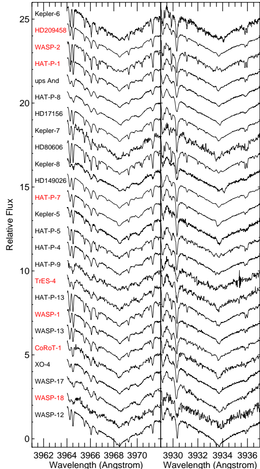
Figure 2. Ca II H & K lines for transiting planet host stars observed with Keck/HIRES, plotted in order of increasing S_{HK} . This plot is a continuation of Fig. 1, and includes stars with lower values of S_{HK} .
