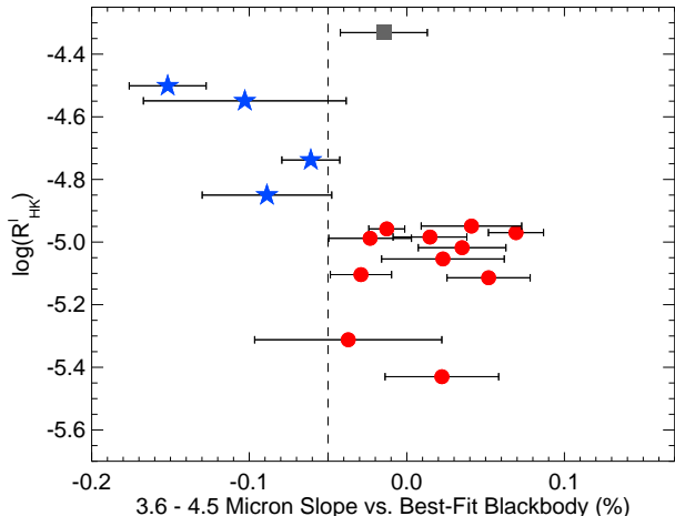
Figure 5. Empirical index for classifying hot Jupiter emission spectra vs Ca II H & K activity index \log(R'_{\text{HK}}) . We derive our index by fitting the 3.6 and 4.5 \mu\text{m} secondary eclipse depths as measured in the Spitzer IRAC bands with a blackbody function for the planet and take the difference between the measured slope across the 3.6 and 4.5 \mu\text{m} bands and the value predicted by the best-fit blackbody function. Planets with blackbody emission will have an index close to zero, whereas planets with negative values are brighter than predicted at 3.6 \mu\text{m} and fainter at 4.5 \mu\text{m} , and planets with positive values have the opposite behavior. Planets classified in the literature as having atmospheric temperature inversions are shown as red circles, while planets without temperature inversions are shown as blue stars (see §3 for a discussion of WASP-2b). CoRoT-2b (grey square) has an unusual spectrum that is not well-described by either model, and we have excluded XO-3 from this plot as its activity level is ambiguously determined from its spectrum (see §2.1). The vertical dashed line at -0.05 delineates a distinction between atmosphere types; in reality there is likely a continuum of behaviors ranging from the default strong absorption (i.e., no inversion), to weak absorption (corresponding to a weak inversion), to no absorption or even emission from an increasingly strong stratosphere.
