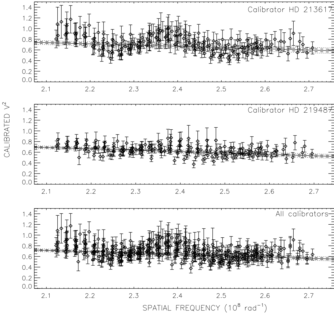
Figure 2. \theta_{LD} fit for HR 8799 on 2010 September 7. The symbols are the same as in Figure 1.
