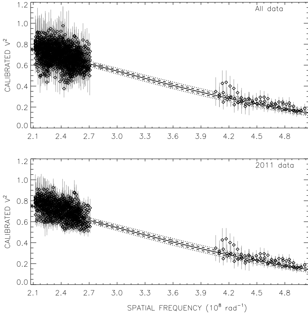
Figure 9. \theta_{\text{LD}} fit for HR 8799 using all calibrators. The symbols are the same as in Figure 1.
