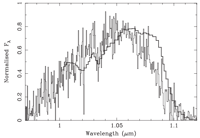
Figure 8. Expanded region of the unbinned spectra in the vicinity of 1.03 \mu\text{m} , along with the 500 K model of Saumon et al. (2012) including opacities due to \text{NH}_3 (thick line). The two spectra have been normalized to F_\lambda = 0.75 in the range 1.045–1.055 \mu\text{m} .
