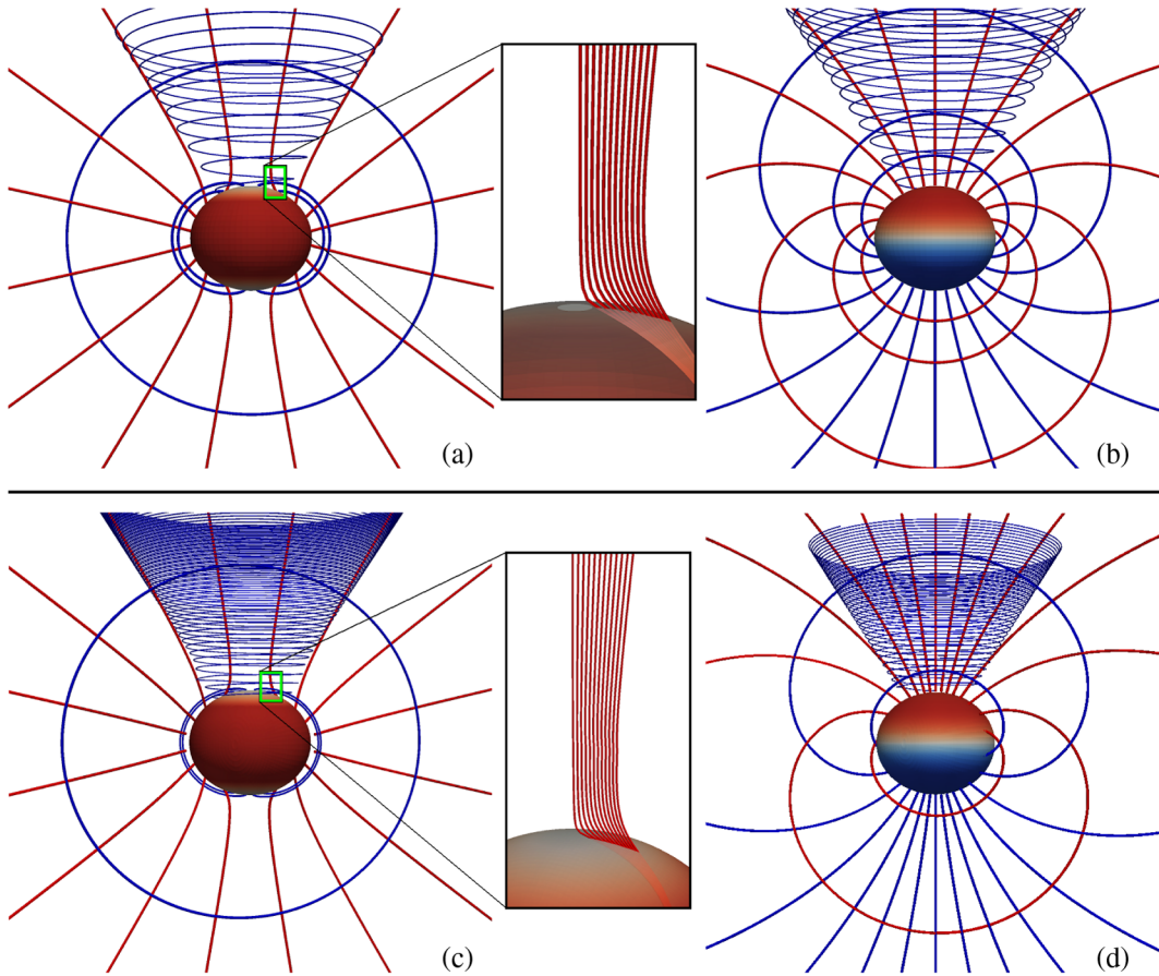
FIG. 6 (color online). Tendex lines and vortex lines for a Kerr black hole with a/M = 0.875 in Kerr-Schild spatial coordinates , for two different slicings: Kerr-Schild \bar{t} = \text{constant} , and Cook-Scheel \bar{t} = \text{constant} . The left and center columns of drawings [panels (a) and (c)] show tendex lines; the right column of drawings [panels (b) and (d)] show vortex lines. The top row of drawings [panels (a) and (b)] is for Kerr-Schild slicing; the bottom row [panels (c) and (d)] is for Cook-Scheel slicing. Since the slicings are different, it is not possible to focus on the same sets of field lines in the Kerr-Schild (upper panels) and Cook-Scheel (lower panels) cases. However, we have attempted to identify similar field lines by ensuring they pass through the same Kerr-Schild spatial coordinate locations on selected surfaces. (The color of the lines and horizon are similar to Fig. 5.)
