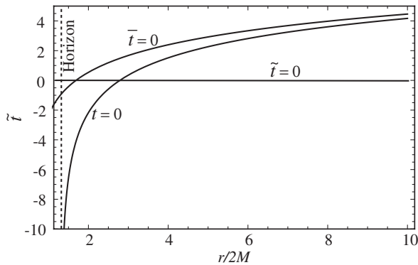
FIG. 3. Slices of constant Boyer-Lindquist time t , Kerr-Schild time \tilde{t} , and Cook-Scheel time \bar{t} , drawn in a Kerr-Schild space-time diagram for a black hole with a/M = 0.95 .
