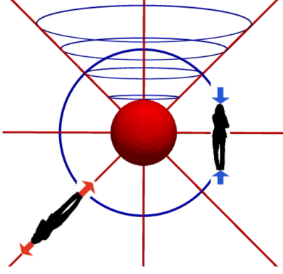
FIG. 1 (color online). Tendex lines for a nonrotating (Schwarzschild) black hole. These lines are identical to those generated by a spherically symmetric mass distribution in the Newtonian limit. Also shown are observers who experience the tidal stretching and compression associated with the tendex lines.
