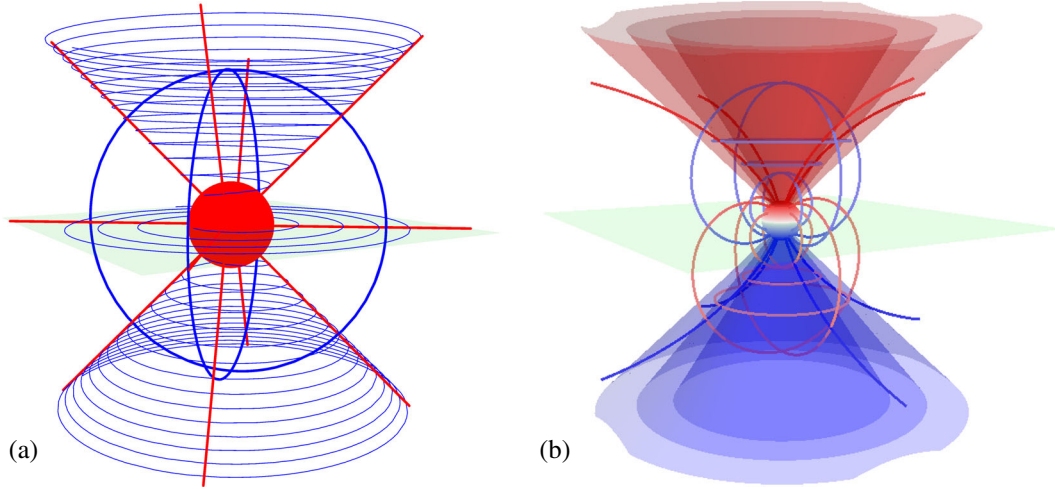
FIG. 2 (color online). (a) Tendex lines and (b) vortex lines for a slowly rotating (Kerr) black hole. Here we take a/M = 0.1 . The horizon is color coded by its tendicity \mathcal{E}_{NN} in (a) (uniformly red [gray] signifying negative tendicity) and vorticity \mathcal{B}_{NN} in (b) (red on top and blue on the bottom), and the field lines are color coded by the sign of their tendicity or vorticity (blue for positive, red for negative). (That is, the radial tendex lines, the vortex lines emerging from the north pole and the azimuthal vortex lines on the bottom carry negative tendicity or vorticity, while all other lines have positive tendicity or vorticity.) In (a), the spiraling lines have been made to spiral more loosely by multiplying the rate of change in the r direction by 5. The semitransparent conelike surfaces emerging from the horizon's north and south polar regions show where the magnitude of the vorticity at a given radius has fallen to 80% (outermost cones), 85%, and 90% (innermost cones) of the polar magnitude. We identify the innermost cone (the 90% contour) as the edge of the frame-drag vortex. The equatorial plane is shown for reference in both panels.
