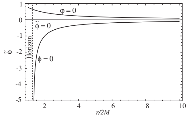
FIG. 4. Curves of constant Boyer-Lindquist angle \phi , Kerr-Schild angle \varphi , and ingoing-Kerr angle \tilde{\phi} for a black hole with a/M = 0.95 .
