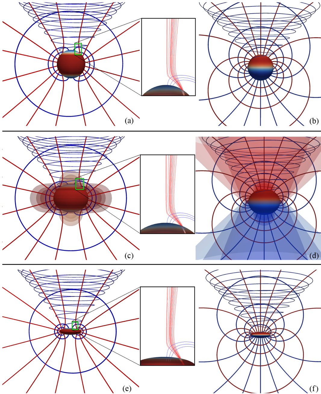
FIG. 5 (color online). Kerr black hole with a/M = 0.95 in Kerr-Schild slicing , drawn in three different spatial coordinate systems. The left and center columns of drawings [panels (a), (c), (e)] show tendex lines; the right column of drawings [panels (b), (d), (f)] show vortex lines. The three rows, from top downward, use ingoing-Kerr spatial coordinates \{r, \theta, \bar{\phi}\} [panels (a) and (b)], Kerr-Schild spatial coordinates \{x, y, z\} [panels (c) and (d)], and Cook-Scheel spatial coordinates \{\bar{x}, \bar{y}, \bar{z}\} [panels (e) and (f)]. In all cases, the lines with positive tendexity or vorticity are colored blue; those with negative tendexity or vorticity are colored red. (The radial tendex lines and vortex lines emerging from the top half of the horizon are red, while all other lines are blue.) The horizon is shown with its horizon tendexity (left column of drawings) and horizon vorticity (right column) color coded from dark blue for strongly positive to dark red for strongly negative. (Horizon tendexity is negative near the equator and positive near the poles. Vorticity on the other hand transitions from being negative on top to positive on the bottom.) In Kerr-Schild coordinates [panels (c) and (d)], we have also shown as semitransparent surfaces, contours of \tilde{r}^3 times tendexity and \tilde{r}^4 times vorticity, where \tilde{r}^2 = x^2 + y^2 + z^2 for Kerr-Schild spatial coordinates. In panel (c), the innermost equatorial contour has the most negative tendexity while the others have 90, 80, 30, 20, and 10% this value, and the innermost polar contour has the least negative tendexity. In panel (d) the contour with the most negative vorticity consists of the innermost red cone and the outermost red bubble (at the north pole), and the others are at 90 and 80% this value. The blue contours of panel (d) (at the bottom half of that panel) are arranged similarly but with positive vorticity.
