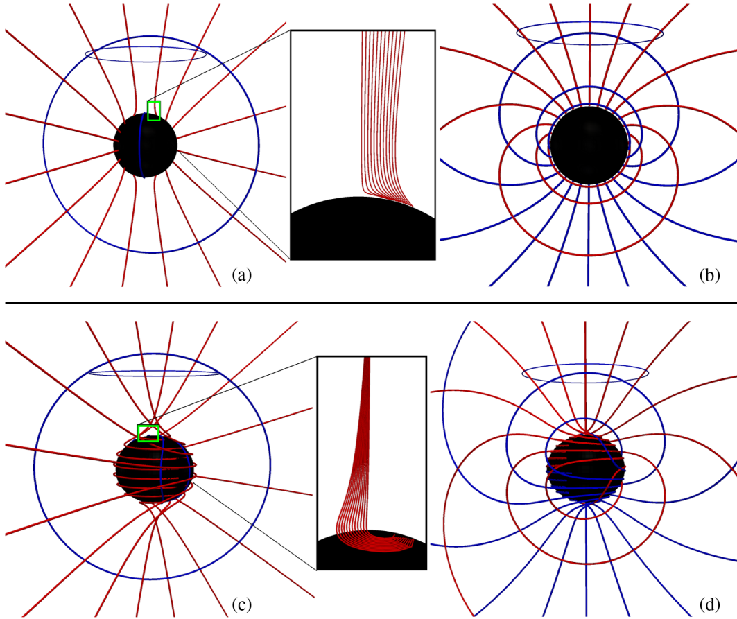
FIG. 7 (color online). (a) Tendex lines for a Kerr black hole with a/M = 0.875 on a slice of constant Boyer-Lindquist time t , plotted in Boyer-Lindquist spatial coordinates . The lines with positive tendicity are colored blue and negative are colored red. (b) Vortex lines for this same black hole, slicing and coordinates, with lines of positive vorticity colored blue and negative colored red. (c), (d) Tendex and vortex lines for the same black hole and same Boyer-Lindquist slicing, but drawn in the Kerr-Schild spatial coordinates . (The color of the lines are similar to Fig. 5.)
