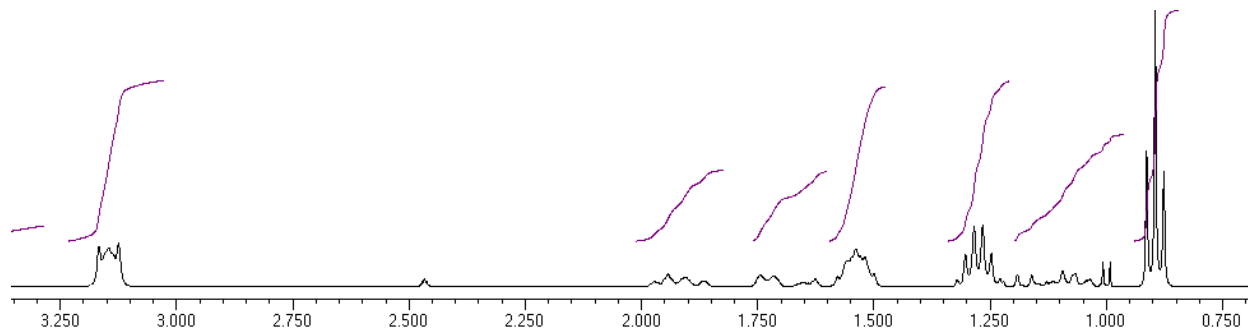
Figure 17: The 1 H NMR spectrum of the monoanion of cis -1,2-CDCA in DMSO using tetrabutylammonium as counterion.
