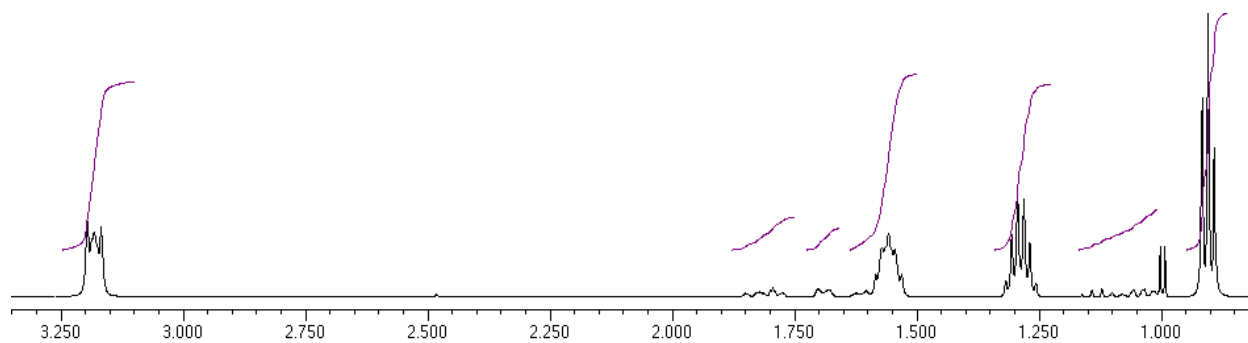
Figure 18: The 1 H NMR spectrum of the dianion of cis -1,2-CDCA in DMSO using tetrabutylammonium as counterion.
