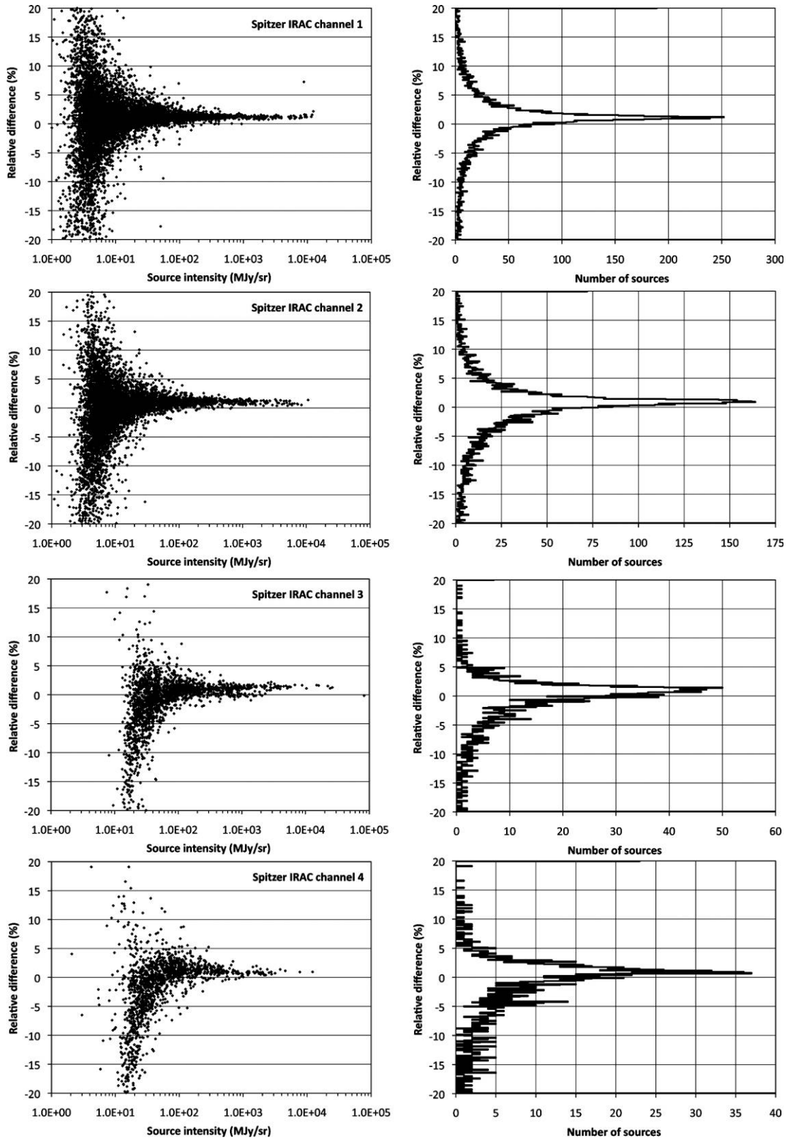
FIG. 10.—Comparison of case Bi source intensity computed by APT vs. SExtractor for filtered sources extracted from the Spitzer IRAC mosaics, channels 1–4. Left : Scatter plots of the relative percentage differences in source intensities between SExtractor and APT as a function of source intensity for all filtered sources of a given Spitzer IRAC channel. Right : Each panel corresponds to the adjacent left panel and is a histogram of the same relative percentage differences.
