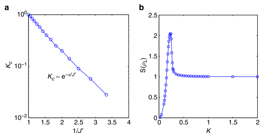
Figure 4 | Critical coupling and von Neumann entropy. (a) The critical coupling K_c as a function of 1/J' in a chain of length N = 400 which shows the exponential scaling predicted in refs 35,36. (b) The von Neumann entropy of \rho_L for the symmetric cut versus the RKKY coupling K for a chain of length N = 800 .
