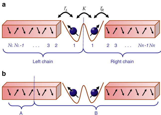
Figure 1 | Schematic picture of the spin-only version of the TIKM. (a) The two impurities interact with their neighbouring spins by Kondo couplings J'_L and J'_R , respectively, and with each other via the RKKY coupling K ; cf. equation (1). (b) Partitioning of the system into two parts A and B , with n_A and n_B = N_L + N_R - n_A spins, respectively. The entanglement spectrum with the associated Schmidt gap is obtained by tracing out one of the subsystems.
