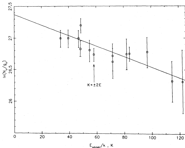
FIG. 2.—LTE rotation diagram of the observed ^{13}\text{CH}_3\text{OH} transitions, with data points centered in 1\sigma error bars. The best fit, shown by the solid line, gives T_{\text{ROT}} = 120 K and N_{\text{COLM}} = 1.3 \times 10^{15} \text{ cm}^{-2} . The K = \pm 2E transitions identified earlier as \text{CO}^+ are indicated by the arrow.
